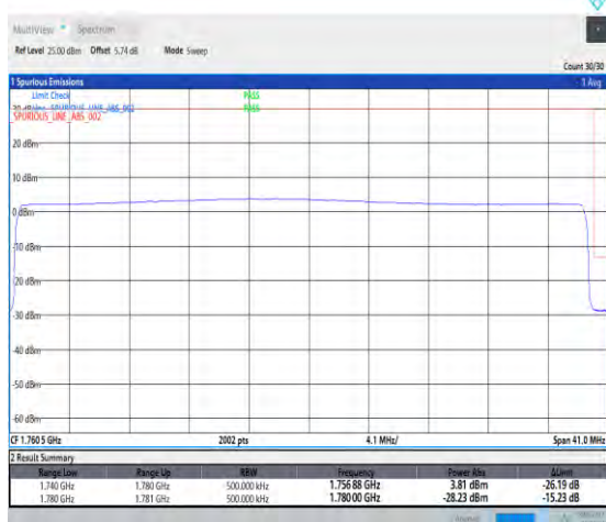
1-N66--15-40-H-6-CP-QPSK-Outer_Full-216@0-A nt1-seegraph-PASS-see graph
