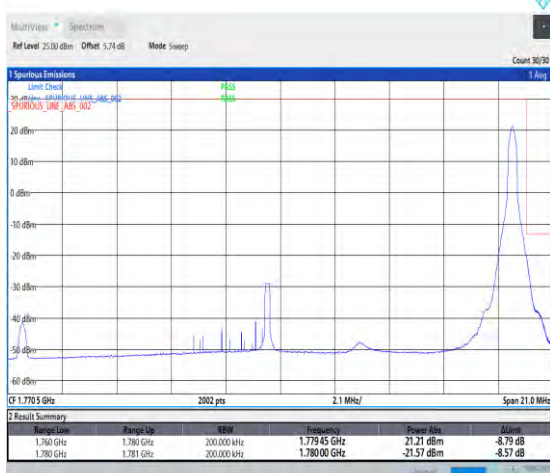
1-N66--15-20-H-5-CP-QPSK-Edge_1RB_Right-1@105 -Ant1-seegraph-PASS-see graph
