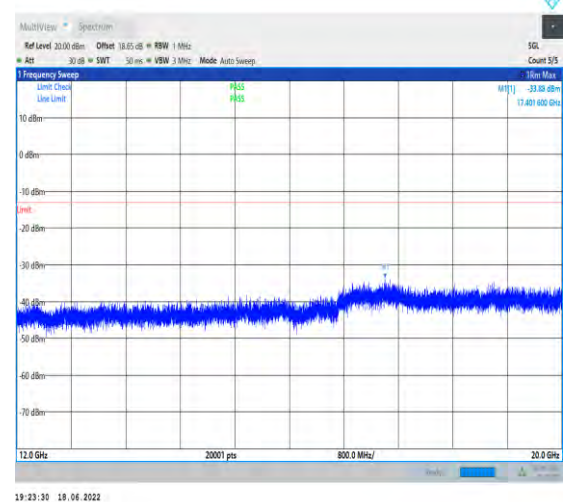
1-N66--15-40-M-1-DFT-PI2BPSK-Inner_1RB_Left-1 @1-12000-20000-Ant1--33.88--13-PASS
