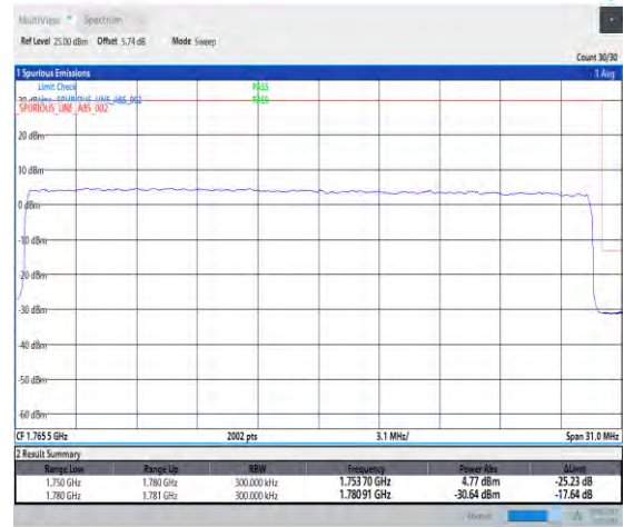
1-N66--15-30-H-3-DFT-PI2BPSK-Outer_Full-160 @0-Ant1-seegraph-PASS-see graph
