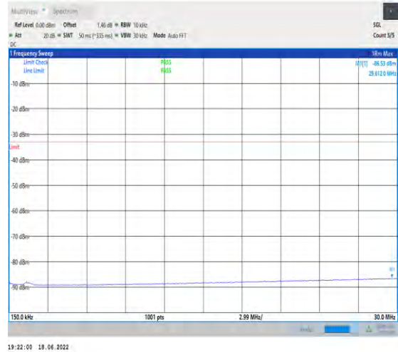
1-N66--15-40-L-1-DFT-PI2BPSK-Inner_1RB_Left-1@ 1-0.15-30-Ant1--86.53--33-PASS
