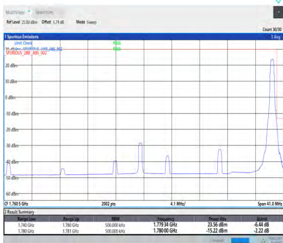
1-N66--15-40-H-2-DFT-PI2BPSK-Edge_1RB_Right-1 @215-Ant1-seegraph-PASS-see graph
