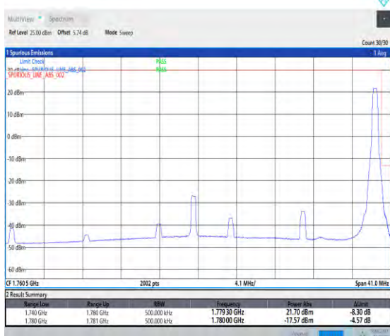
1-N66--15-40-H-5-CP-QPSK-Edge_1RB_Right-1@215 -Ant1-seegraph-PASS-see graph
