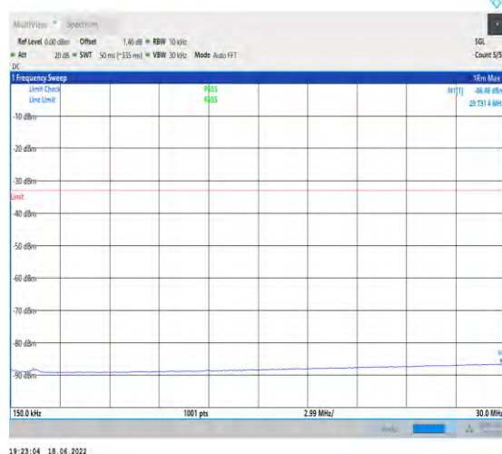
1-N66--15-40-M-1-DFT-PI2BPSK-Inner_1RB_Left-1 @1-0.15-30-Ant1--86.49--33-PASS
