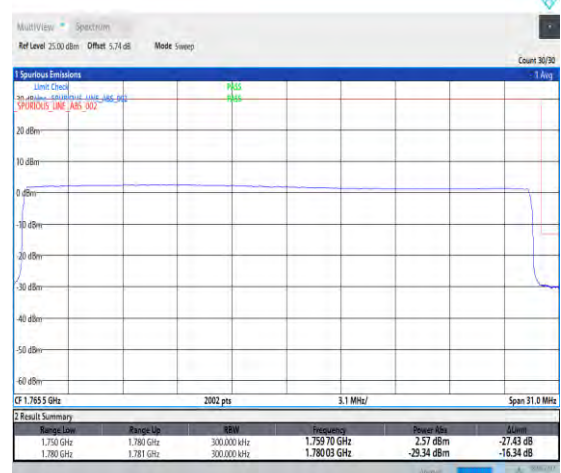
1-N66--15-30-H-6-CP-QPSK-Outer_Full-160@0-A nt1-seegraph-PASS-see graph
