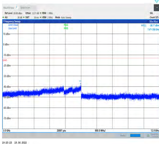
1-N66--15-40-M-1-DFT-PI2BPSK-Inner_1RB_Left-1 @1-3000-12000-Ant1--38.17--13-PASS
