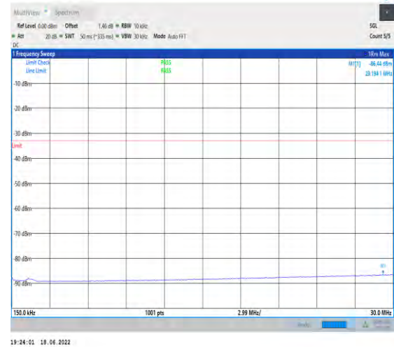
1-N66--15-40-H-1-DFT-PI2BPSK-Inner_1RB_Left-1 @1-0.15-30-Ant1--86.44--33-PASS
