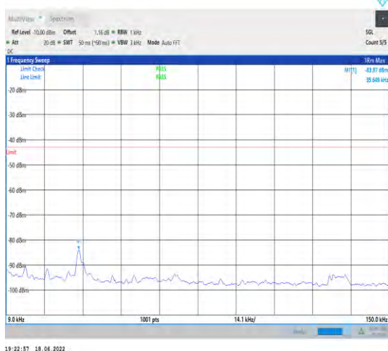
1-N66--15-40-M-1-DFT-PI2BPSK-Inner_1RB_Left-1 @1-0.009-0.15-Ant1--83.97--43-PASS
