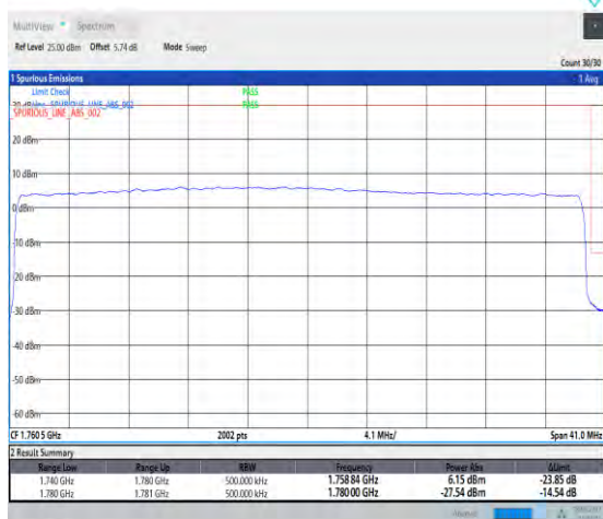
1-N66--15-40-H-3-DFT-PI2BPSK-Outer_Full-216 @0-Ant1-seegraph-PASS-see graph
