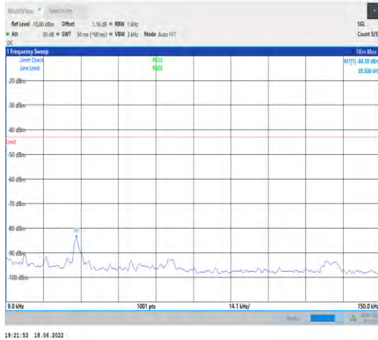
1-N66--15-40-L-1-DFT-PI2BPSK-Inner_1RB_Left-1 @1-0.009-0.15-Ant1--84.39--43-PASS
