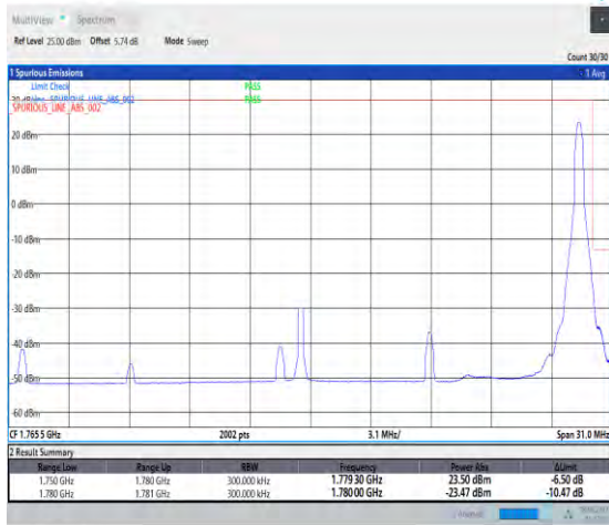
1-N66--15-30-H-2-DFT-PI2BPSK-Edge_1RB_Right-1 @159-Ant1-seegraph-PASS-see graph
