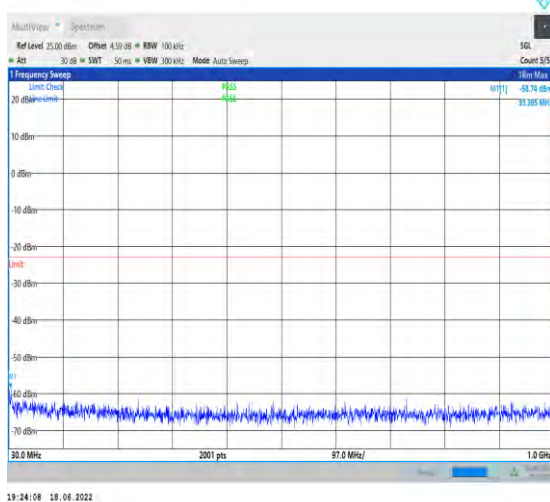
1-N66--15-40-H-1-DFT-PI2BPSK-Inner_1RB_Left-1 @1-30-1000-Ant1--58.74--23-PASS
