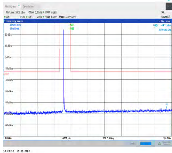
1-N66--15-40-L-1-DFT-PI2BPSK-Inner_1RB_Left-1@ 1-1000-3000-Ant1--45.23--13-PASS
