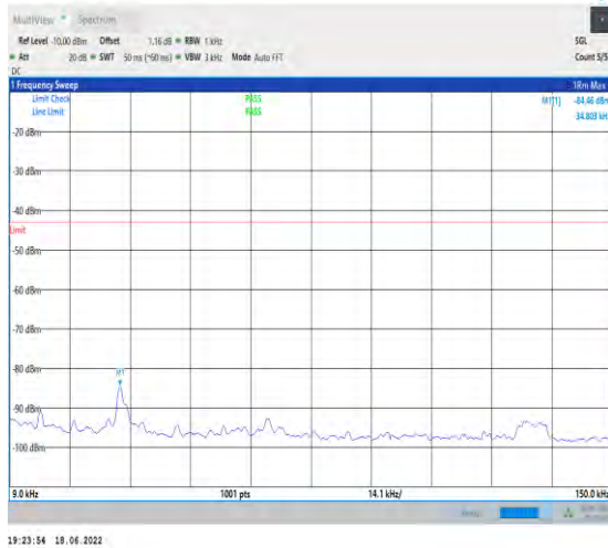
1-N66--15-40-H-1-DFT-PI2BPSK-Inner_1RB_Left-1 @1-0.009-0.15-Ant1--84.46--43-PASS
