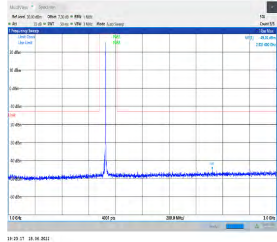
1-N66--15-40-M-1-DFT-PI2BPSK-Inner_1RB_Left-1 @1-1000-3000-Ant1--45.02--13-PASS
