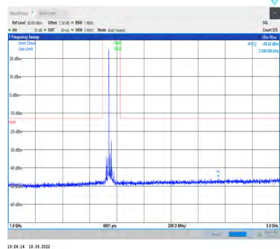
1-N66--15-40-H-1-DFT-PI2BPSK-Inner_1RB_Left-1 @1-1000-3000-Ant1--45.43--13-PASS
