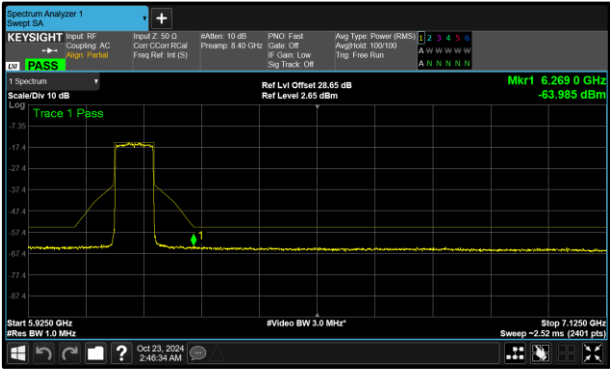
Figure 359 - A (Core 0) 802.11ax HE80 SU VLP 6145 MHz (CH39)
