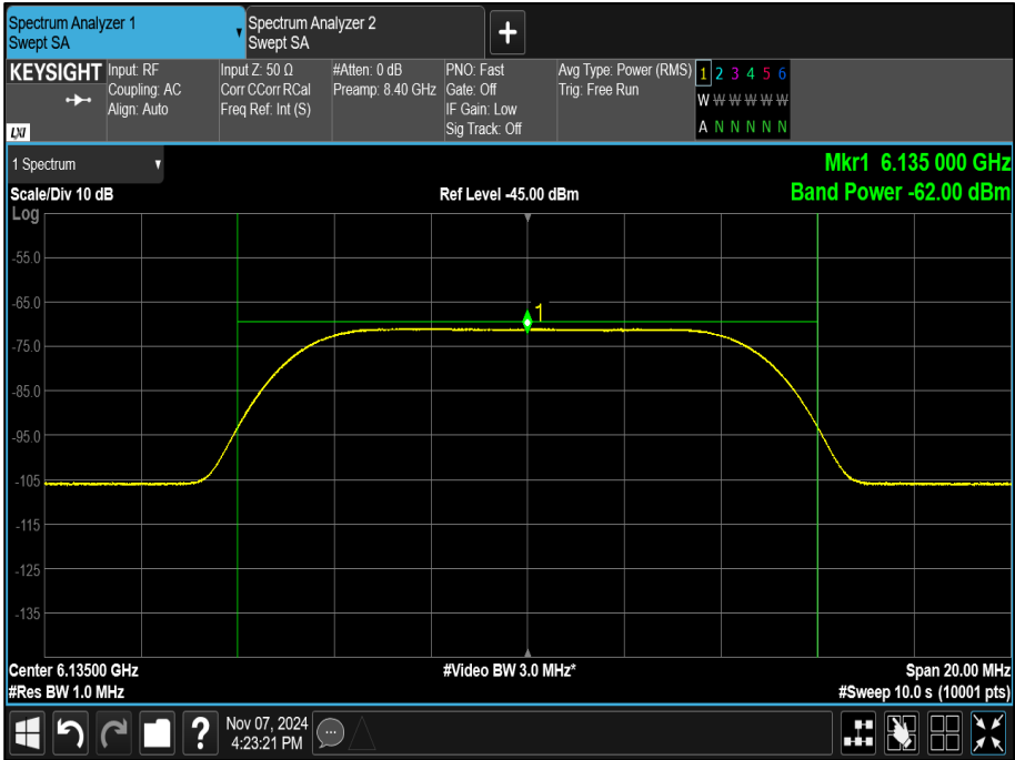
Figure 361 - Example of AWGN Signal
