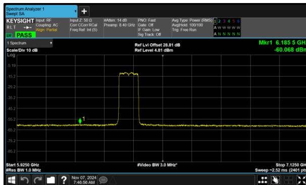
Figure 350 - A (Core 0) 802.11ax HE80 SU VLP 6385 MHz (CH87)
