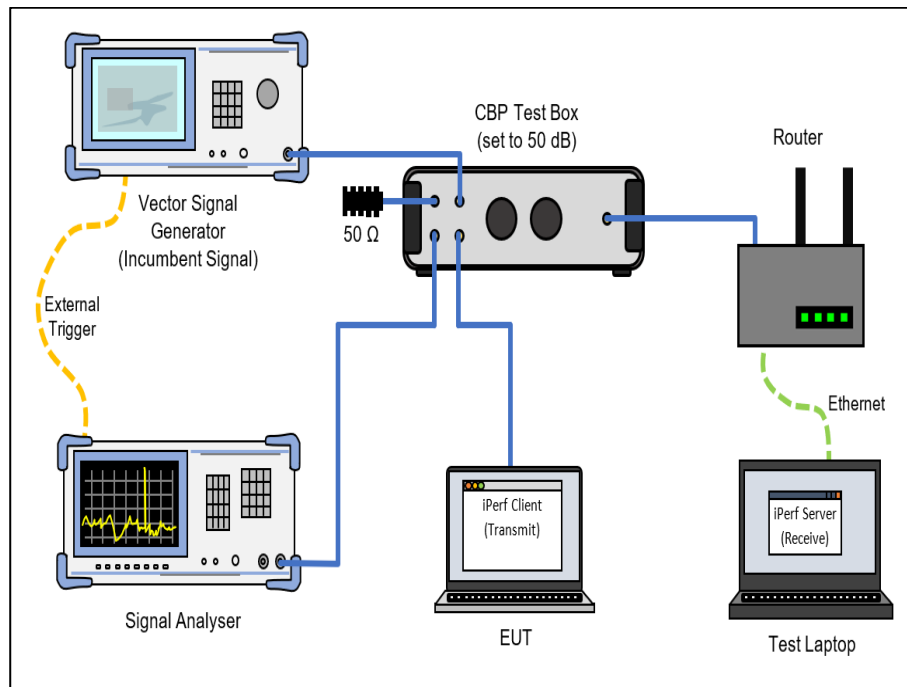
Figure 360 - Test Equipment Setup Diagram
