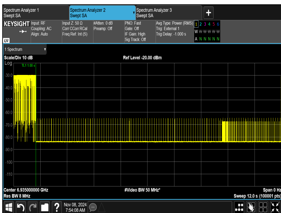
Figure 375 - U-NII-8, Maximum Bandwidth (AWGN Low)
