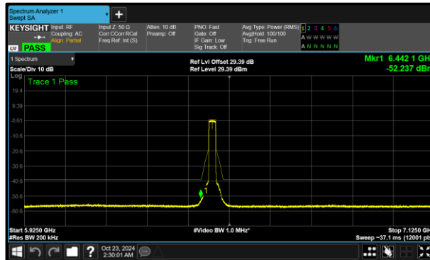
Figure 356 - A (Core 0) 802.11ax HE20 SU SP 6475 MHz (CH105)
