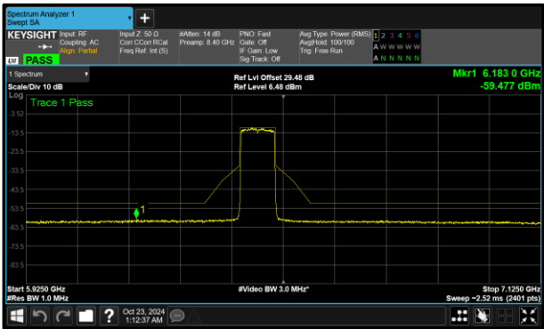
Figure 355 - A (Core 0) 802.11ax HE80 SU LPI 6465 MHz (CH103)
