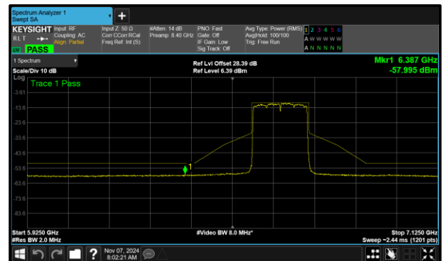
Figure 351 - B (Core 1) 802.11ax HE160 SU VLP 6665 MHz (CH143)
