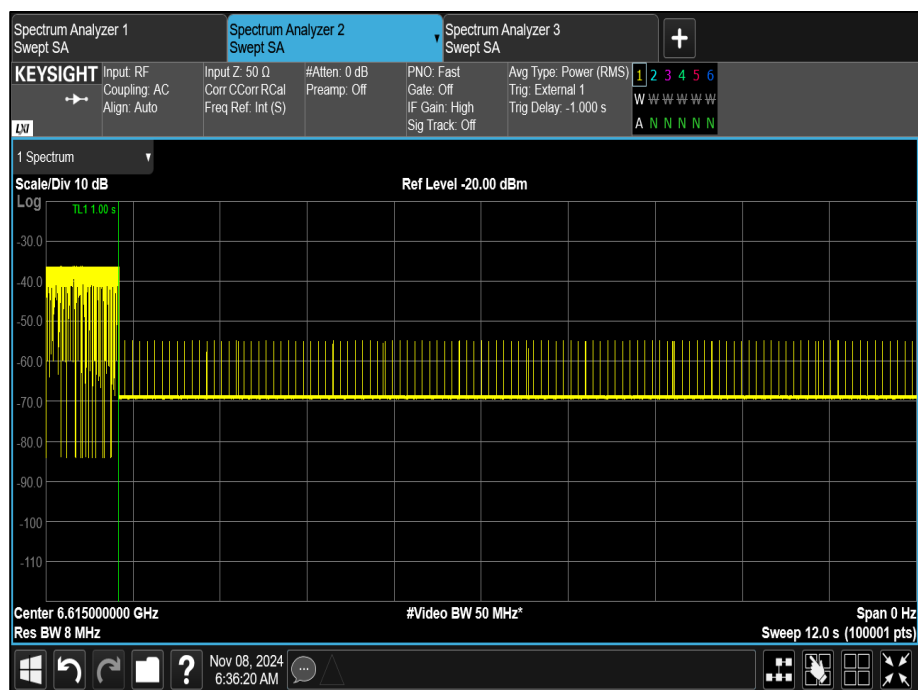
Figure 370 - U-NII-7, Minimum Bandwidth
