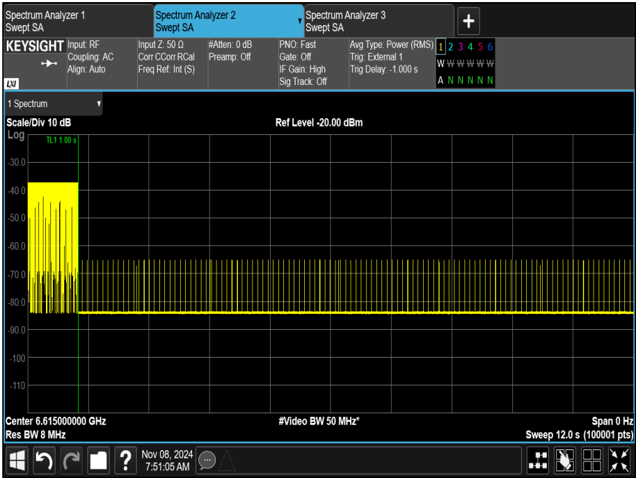
Figure 373 - U-NII-7, Maximum Bandwidth (AWGN High)
