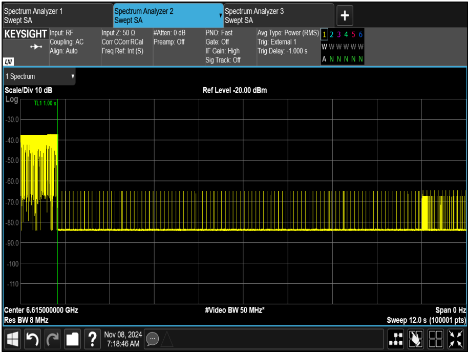
Figure 372 - U-NII-7, Maximum Bandwidth (AWGN Mid)
