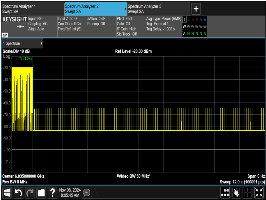
Figure 377 - U-NII-8, Maximum Bandwidth (AWGN High)
