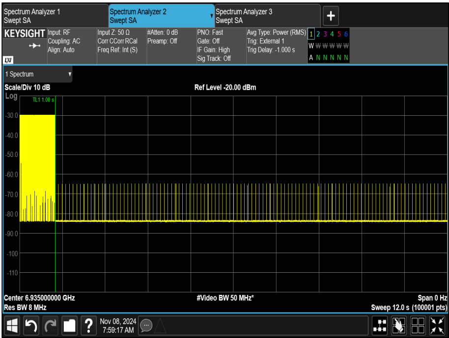
Figure 376 - U-NII-8, Maximum Bandwidth (AWGN Mid)
