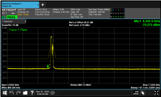
Figure 352 - A (Core 0) 802.11ax HE20 RU106 VLP 6275 MHz (CH65)
