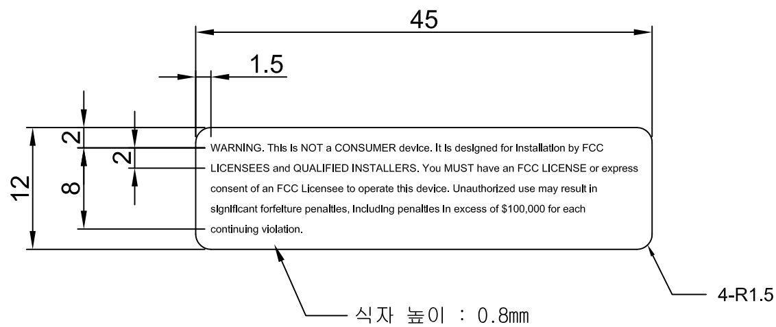
[ HRDU용 WARNING Label ] [ 4304-001062 ]
