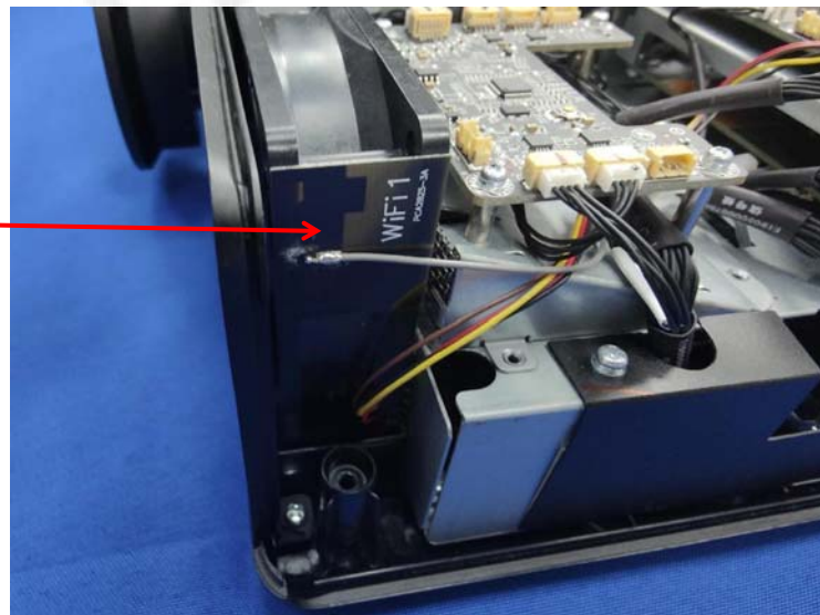
WIFI 1 Antenna
