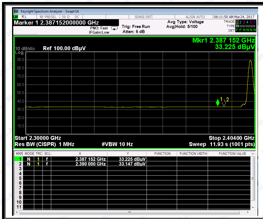
(Plot A2: Channel = 0 AVG)
