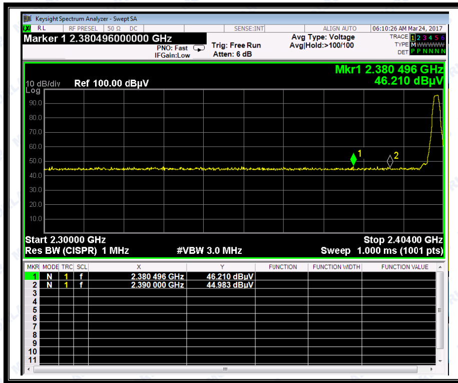
(Plot A1: Channel = 0 PEAK)
