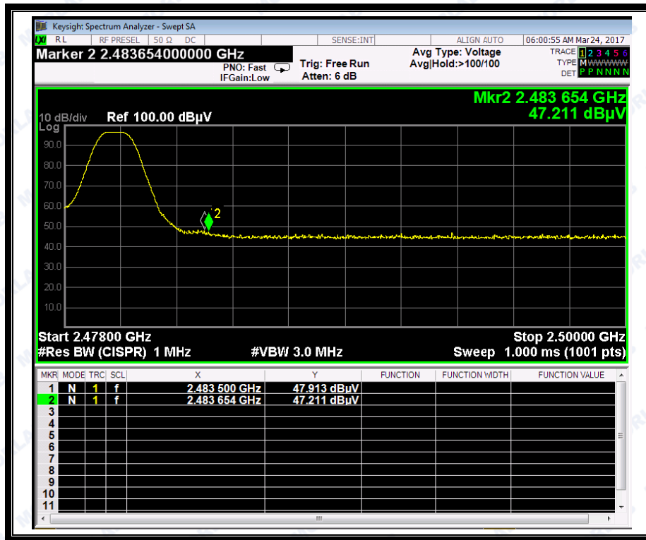
(Plot B1: Channel = 39 PEAK)
