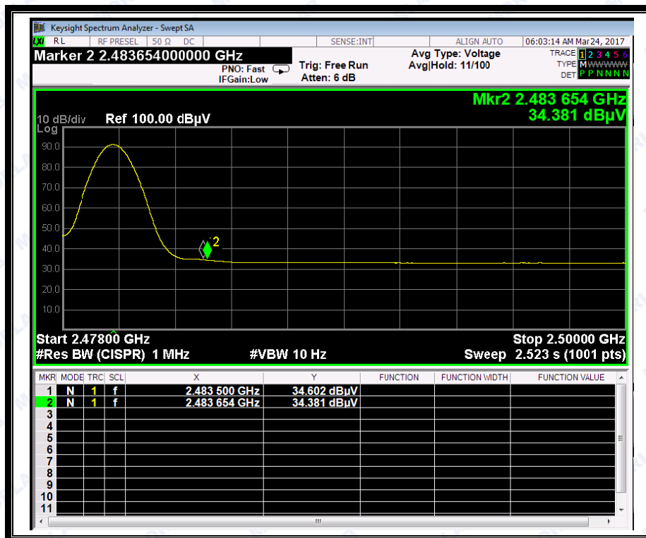
(Plot B2: Channel = 39 AVG)
