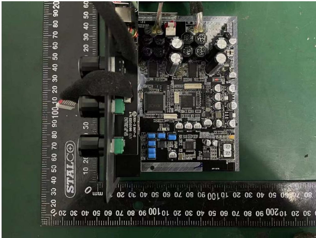
Internal photos M/N: EDF100042
