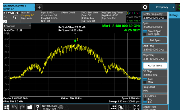
CH39 (2480MHz) LE(1Mbps)
