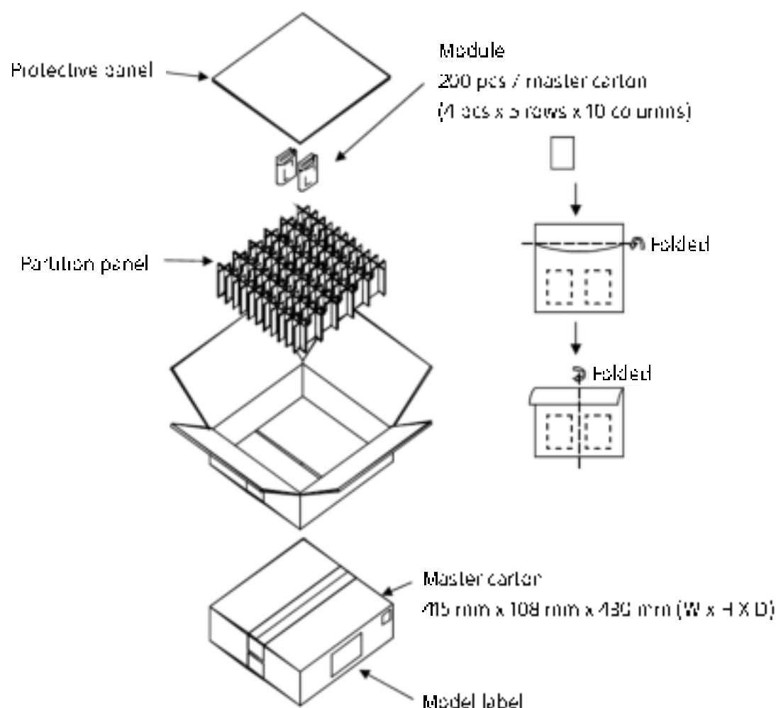
Figure 5-1: Packing details
