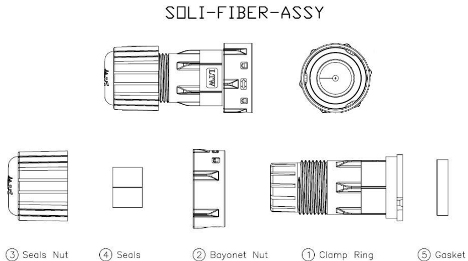
Figure 4.10 – Information of Optical Connector
