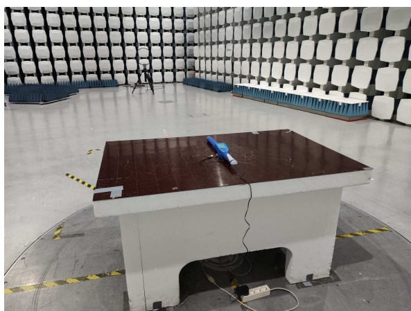
Radiated Emissions
