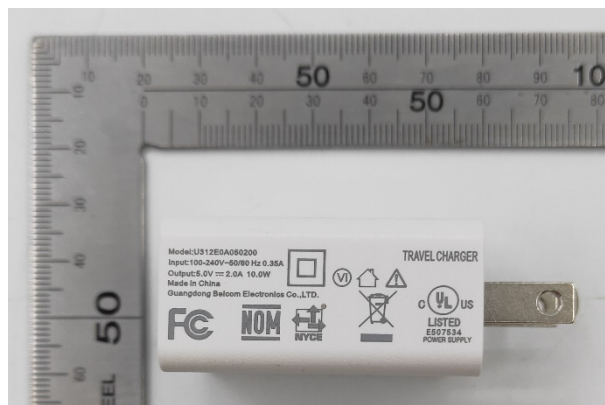
Charger View (Model: U312E0A050200 made by Guangdong Belcom Electronics Co.,LTD.)
