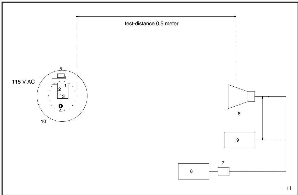
Figure 5: Measurement setup for radiated emission test above 18 GHz
