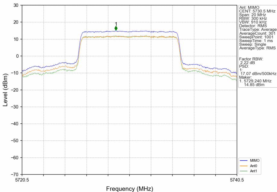
10M_LCH_5730.5MHz_MIMO_NTNV
