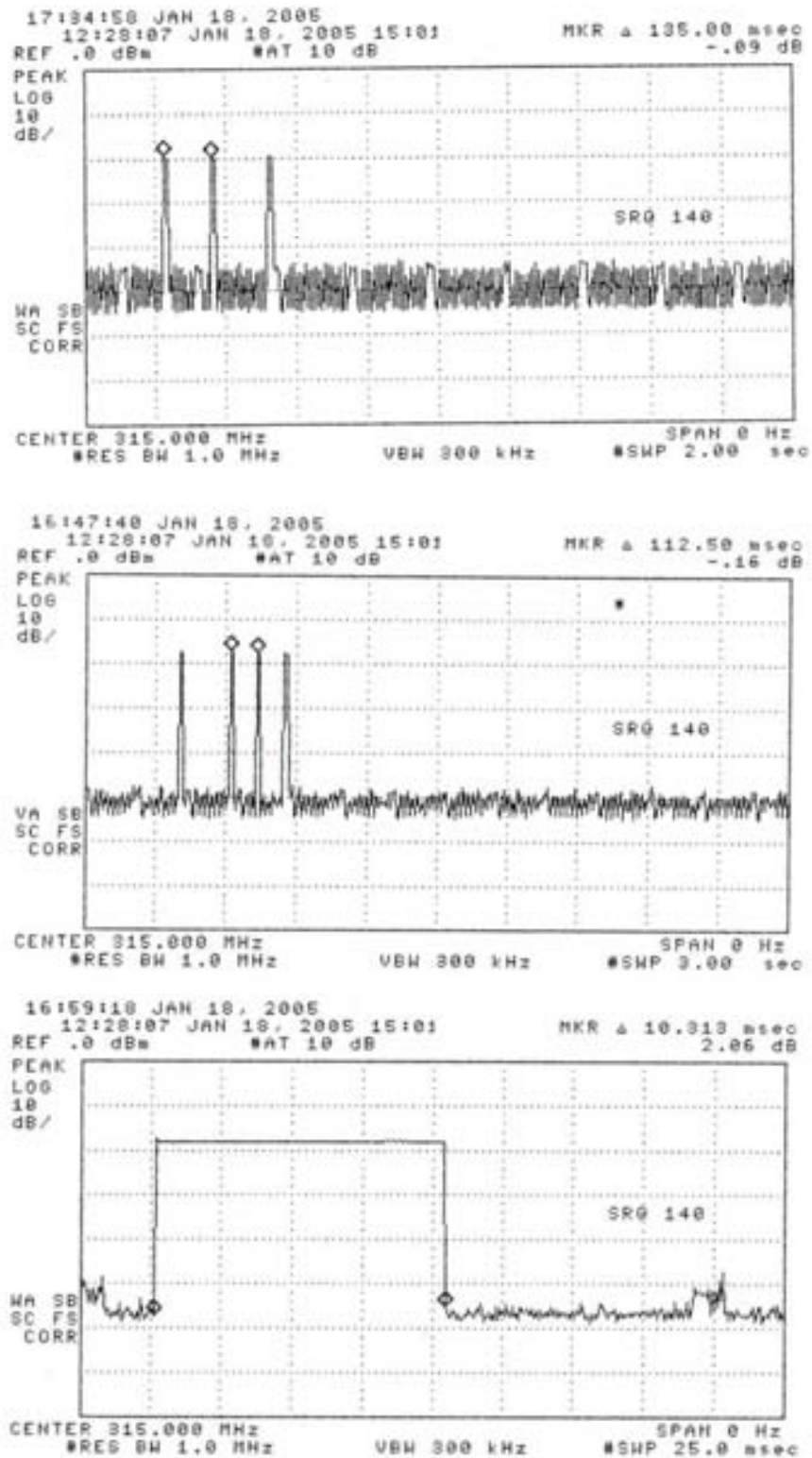
Figure 6.1. Transmissions modulation characteristics: (top) low line transmission, (center) high line, (bottom) expanded word (same for high and low line).
