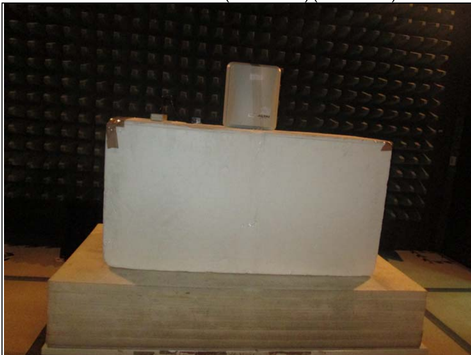
Radiated Emission Test (Above 1GHz) (Test Mode B)
