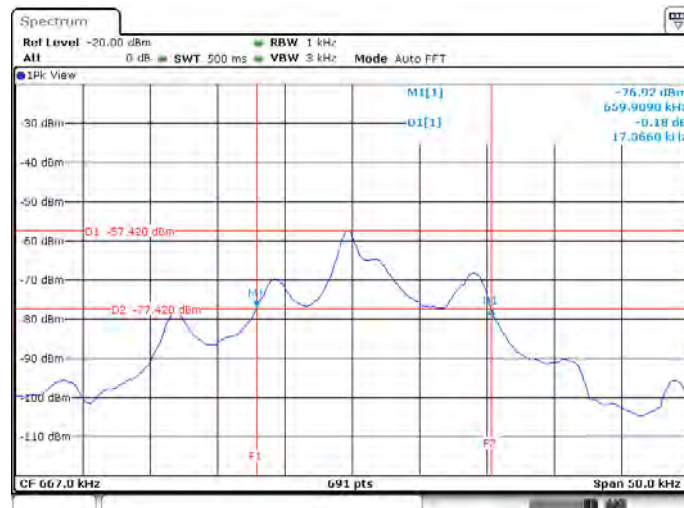
Emission Bandwidth Plot - 20dB Bandwidth
