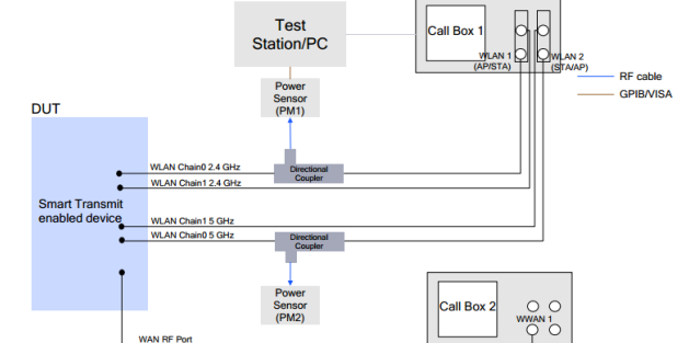
WLAN DBS Test setup - MIMO
