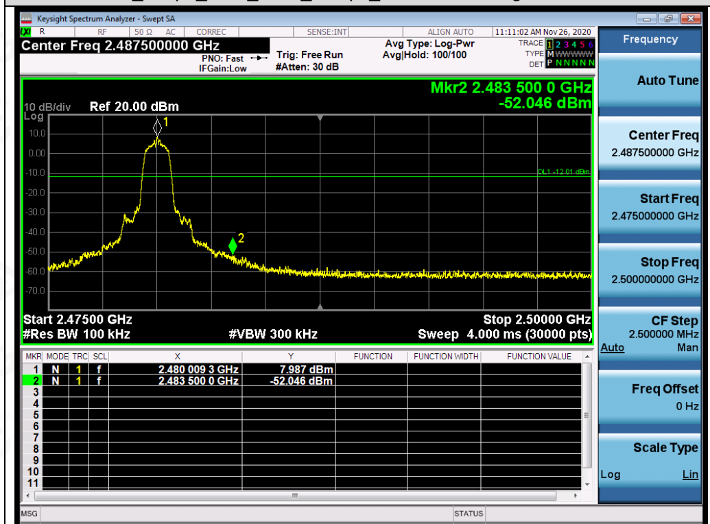
Test_Graph_EDR_2480_2Mbps_Higher Band Edge Emissions
