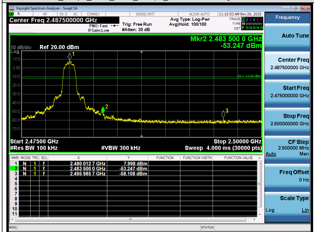
Test_Graph_EDR_2480_3Mbps_Higher Band Edge Emissions
