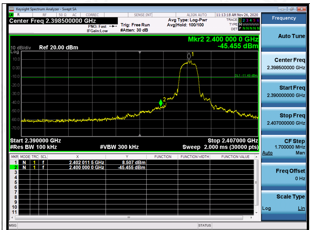
Test_Graph_EDR_2402_3Mbps_Lower Band Edge Emissions
