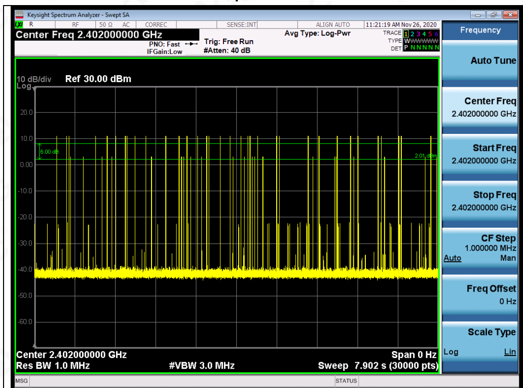
Test_Graph_BR_HOP_NA_1Mbps_2402_Number of Busrt
