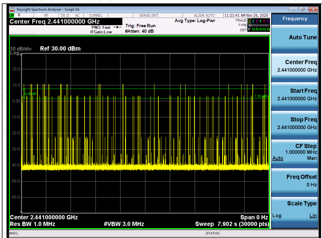
Test_Graph_BR_HOP_NA_1Mbps_2441_Number of Burst
