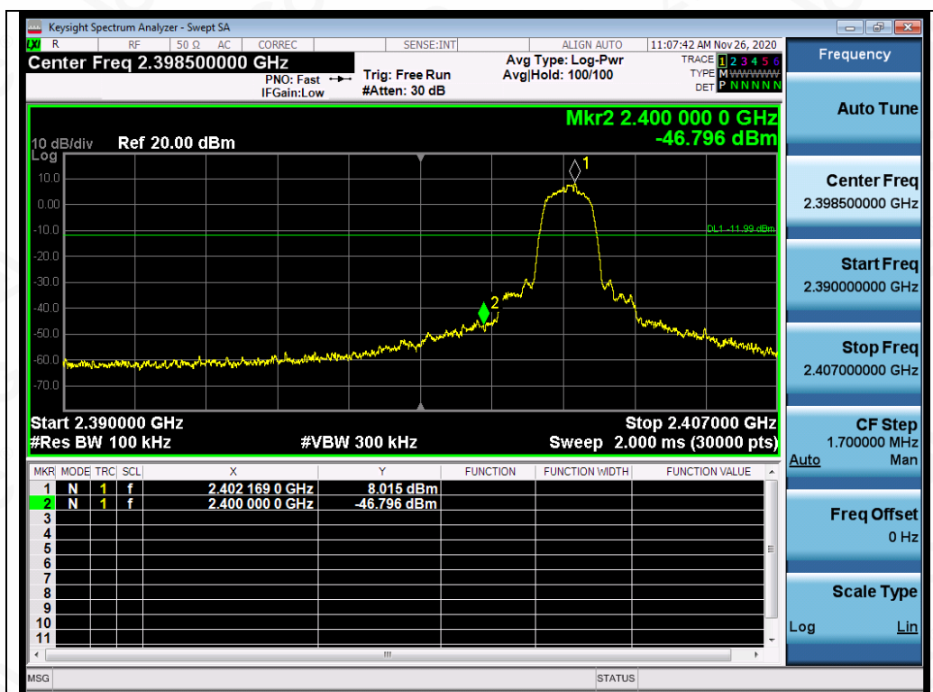
Test_Graph_EDR_2402_2Mbps_Lower Band Edge Emissions
