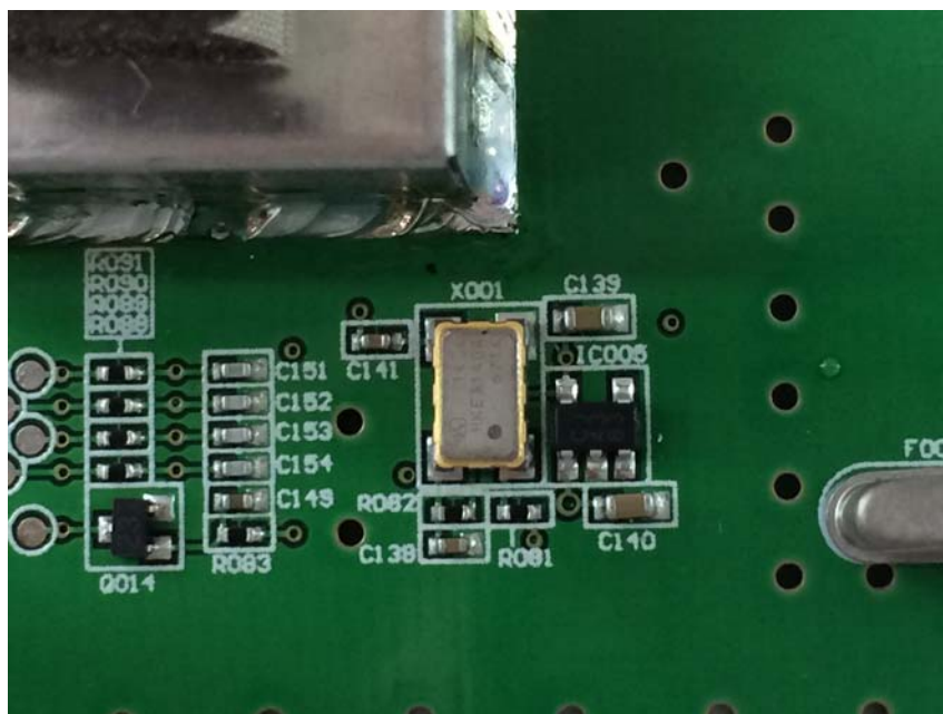
Oscillator view 4
