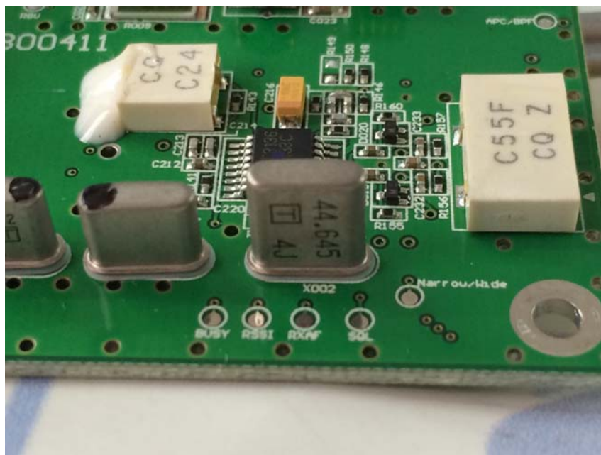
Oscillator view 2
