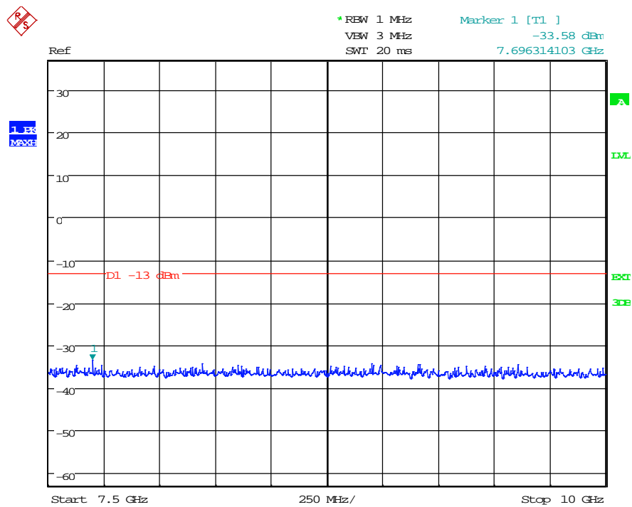
(Plot 4.6.2 D5: Idle @ WCDMA Band V)
