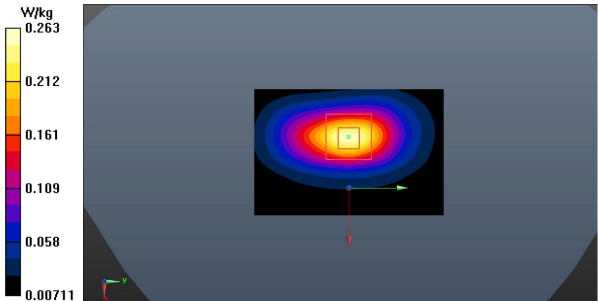
Fig.4 GSM 1900 Body
