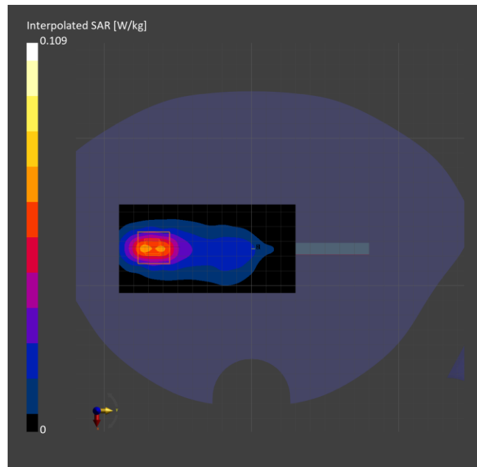
Fig.40 Bluetooth Body
