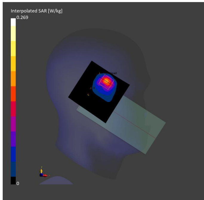
Fig.39 Bluetooth Head
