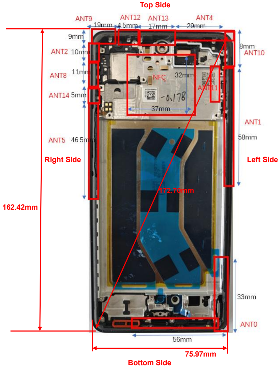
Picture 12.1 Antenna Locations (Back View)
