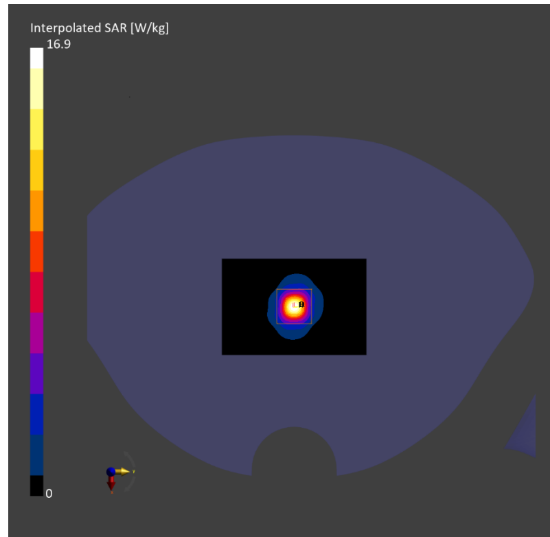
Fig.B.17. Validation 5750MHz 50mW
