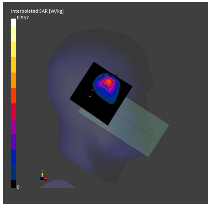
Fig.41 WLAN 2.4GHz Head
