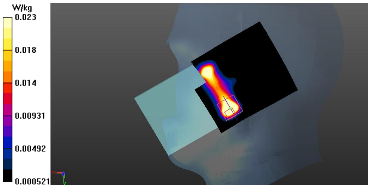
Fig.3 GSM 1900 Head
