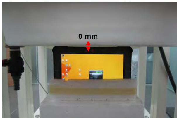
Fig.6 EUT Top side to flat phantom
