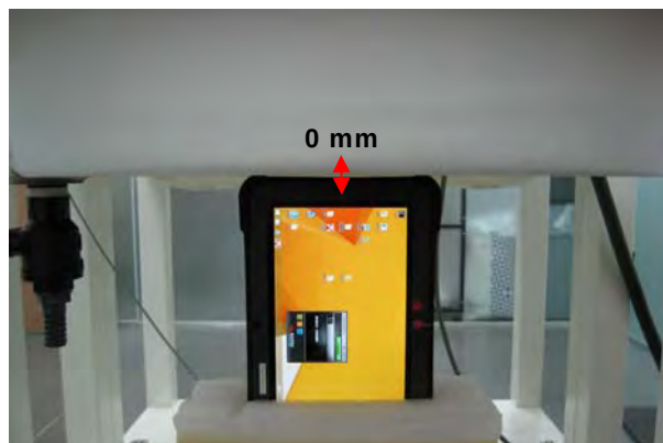
Fig.5 EUT Left side to flat phantom
