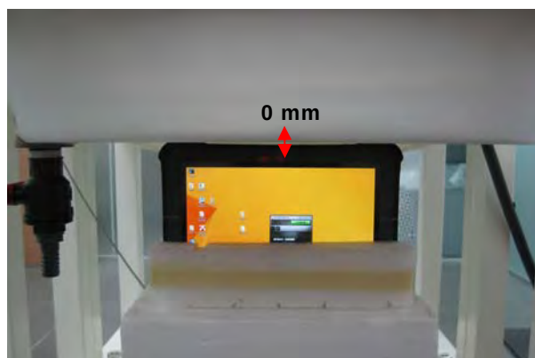
Fig.10 EUT with mobile battery top side to flat phantom
