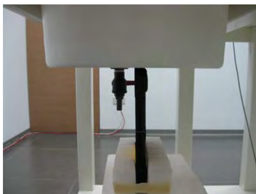
Fig.5 EUT Left side to flat phantom
