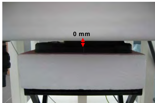
Fig.9 EUT with mobile battery back side to flat phantom
