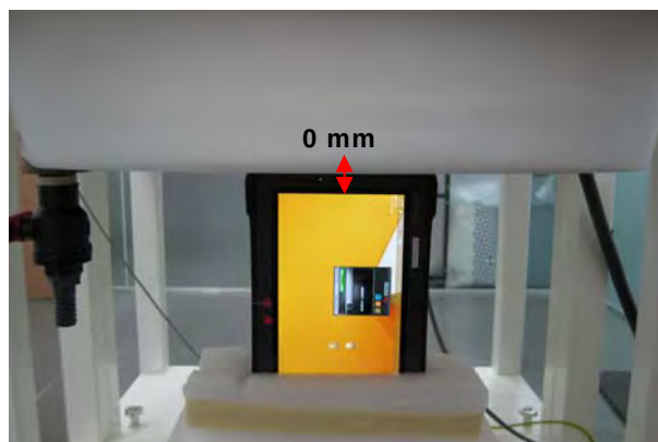
Fig.4 EUT Right side to flat phantom
