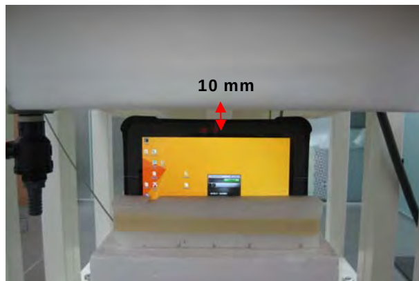
Fig.11 EUT with mobile battery top side to flat phantom
