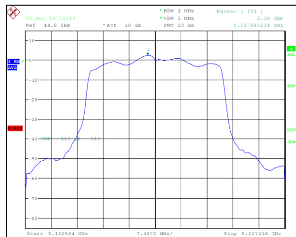
Channel Frequency:5190MHz
