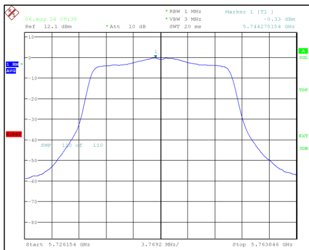
Chain :-1
