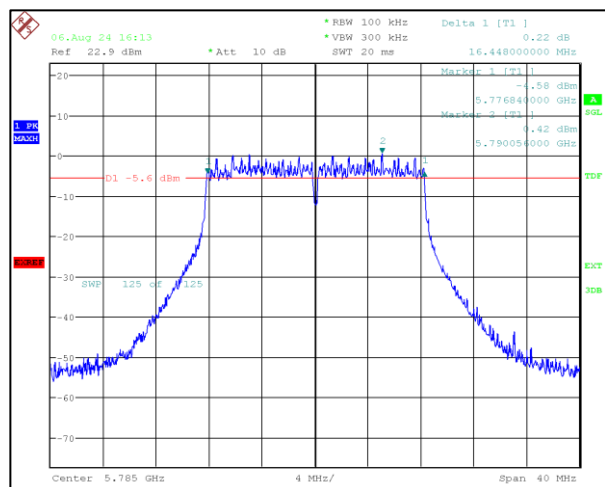
Channel Frequency:5785MHz
