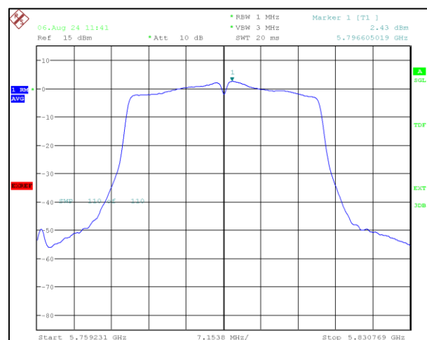
Channel Frequency:5795MHz
