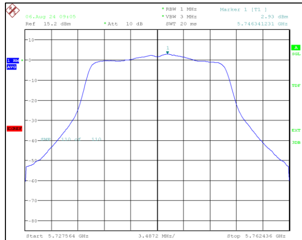
Chain :-2
