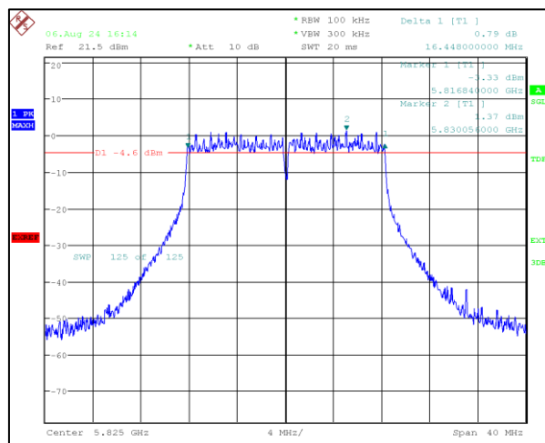
Channel Frequency:5825MHz
