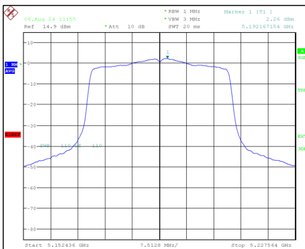
Channel Frequency:5190MHz
