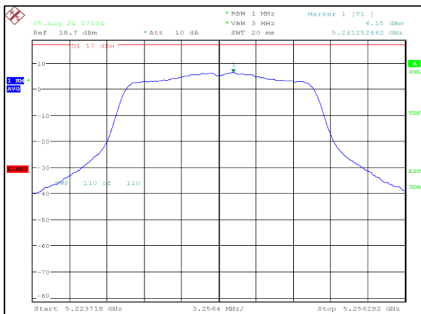
Channel Frequency:5240MHz
