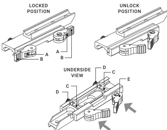
FIGURE 2-5. MOUNT
