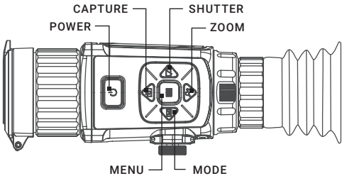
FIGURE 2-2. CONTROL BUTTONS
