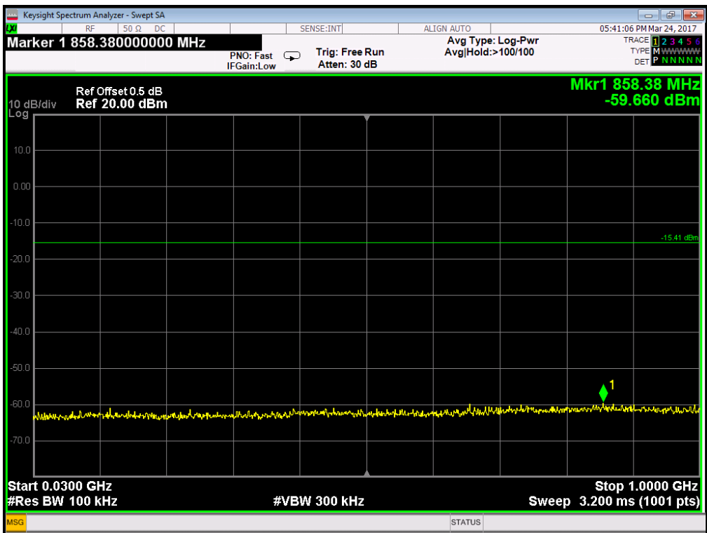
Conducted Spurious Emission Plot on Bluetooth LE 1Mbps
