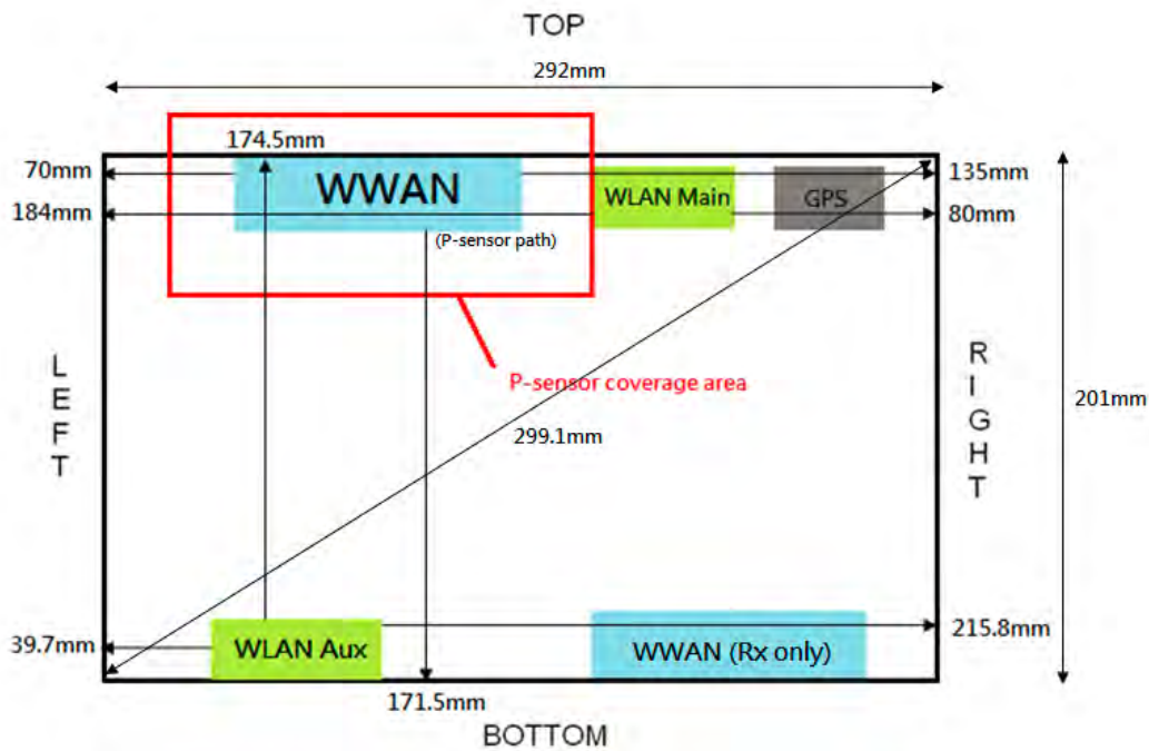
Fig.16 Antenna position of EUT (Front view)
