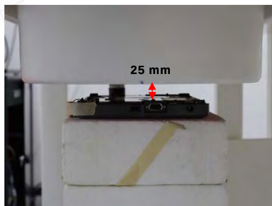
Fig.4 EUT Back side (25mm) to flat phantom
