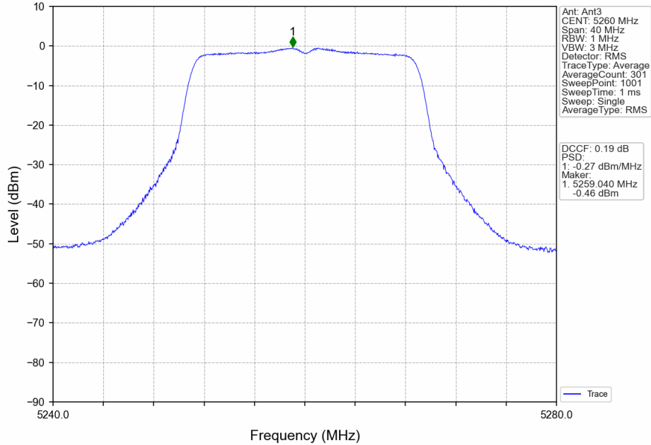
802.11n(HT20)_LCH_5260MHz_MIMO_NTNV
