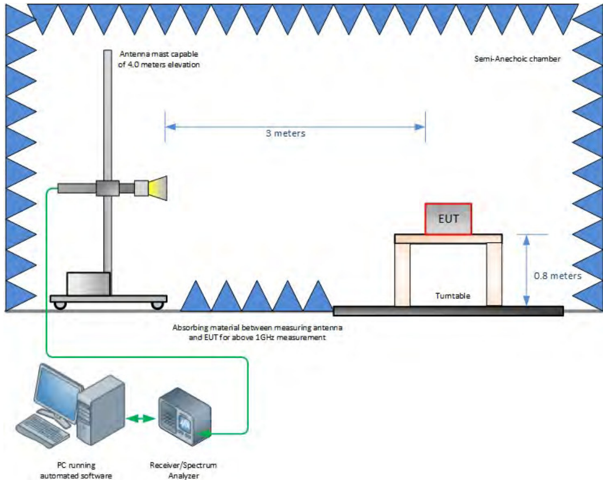
Radiated Emission Test Setup (Above 1GHz) (if applicable)
