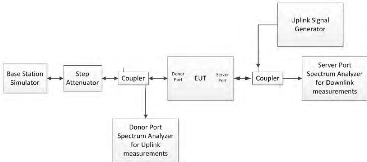
Figure 1: Test Configuration in Normal Mode
