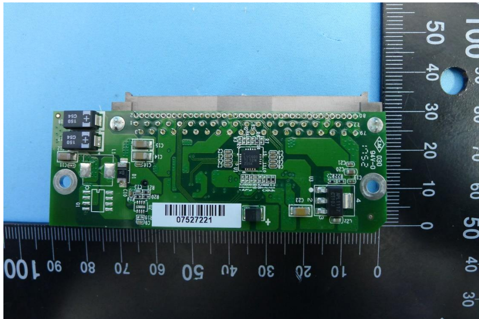
(35) EUT Photo
