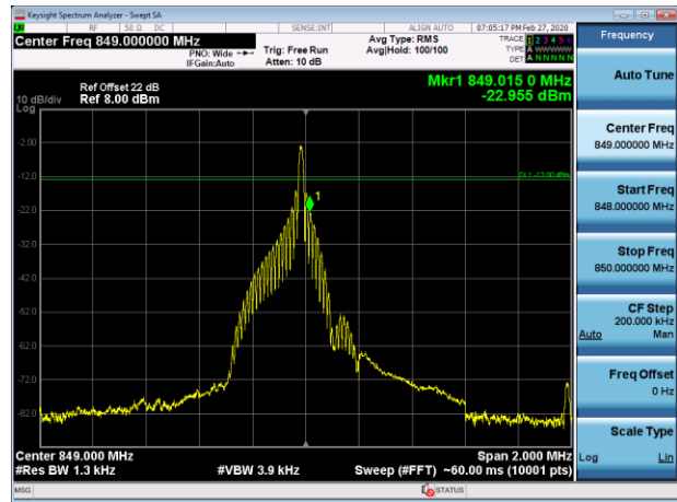
Channel 20649-1 tone offset 11, BW 15kHz, BPSK
