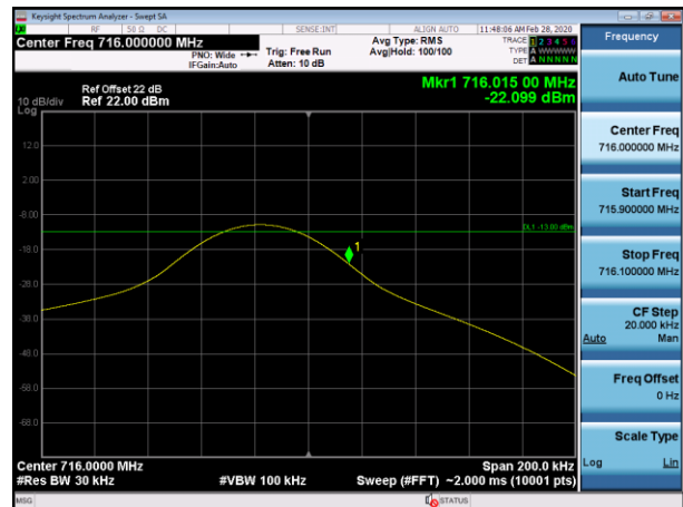
Channel 23849-1 tone offset 11, BW 15kHz, QPSK
