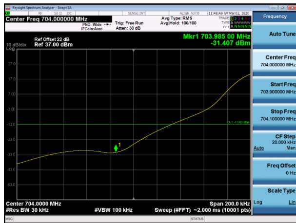
Channel 23732-1 tone offset 0, BW 3.75kHz, BPSK
