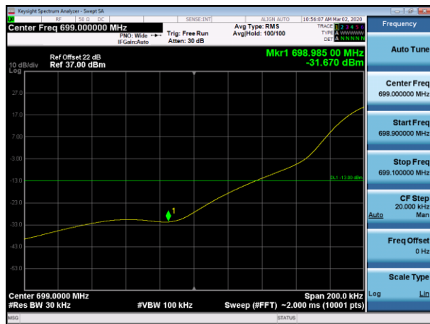
Channel 23012-1 tone offset 0, BW 3.75kHz, BPSK
