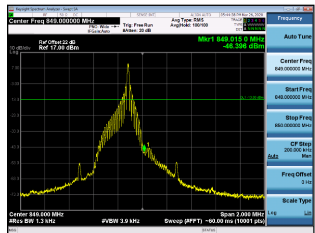
Channel 20648-1 tone offset 11, BW 15kHz, BPSK
