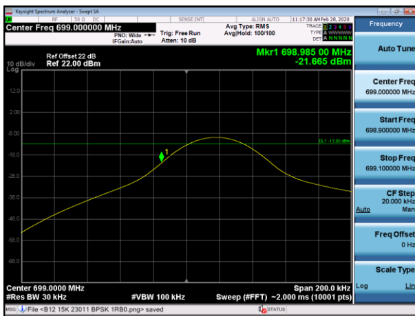
Channel 23011-1 tone offset 0, BW 15kHz, BPSK
