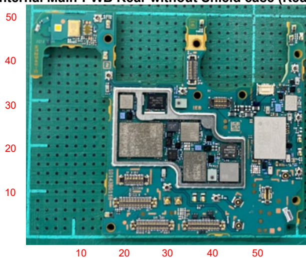
Internal Main-PWB Rear without Shield case (Rear-side)
