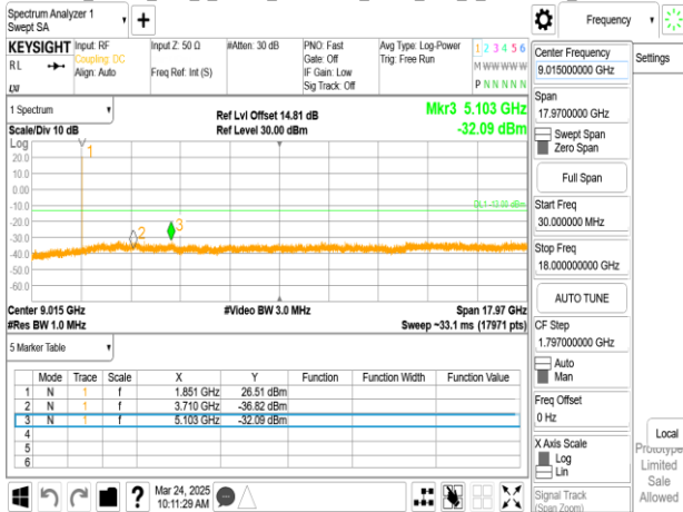
Band2_10MHz_DFT_s_OFDM_SCS15kHz_BPSK_RB1_1_CH371000upper 18G
