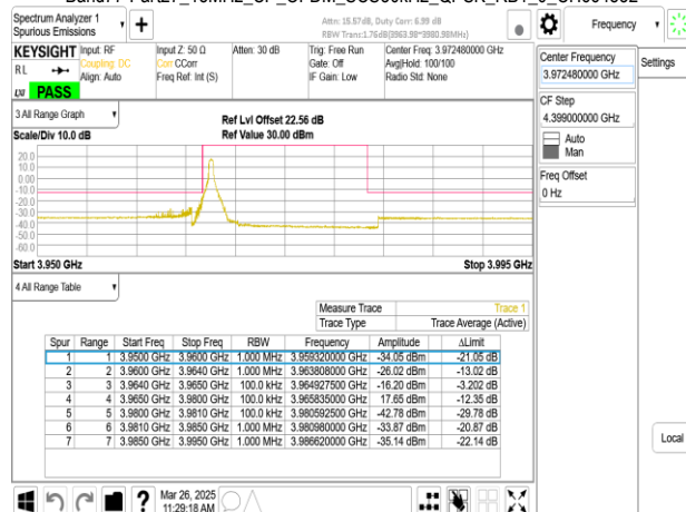
Band77-Part27_15MHz_CP_OFDM_SCS30kHz_QPSK_RB1_37_CH664832
