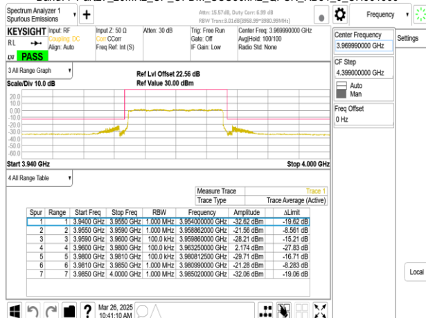
Band77-Part27_20MHz_CP_OFDM_SCS30kHz_QPSK_RB51_0_CH664666
