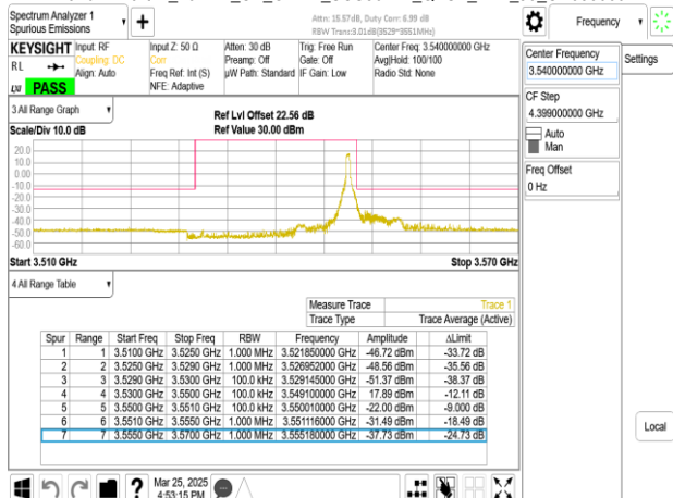
Band77-Part27_20MHz_CP_OFDM_SCS30kHz_QPSK_RB51_0_CH636000
