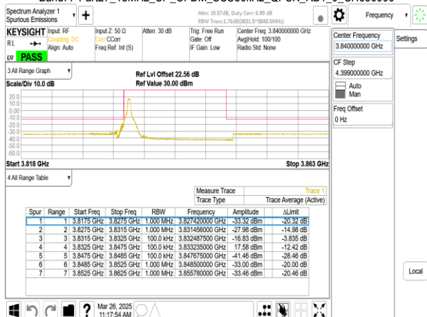
Band77-Part27_15MHz_CP_OFDM_SCS30kHz_QPSK_RB1_37_CH656000
