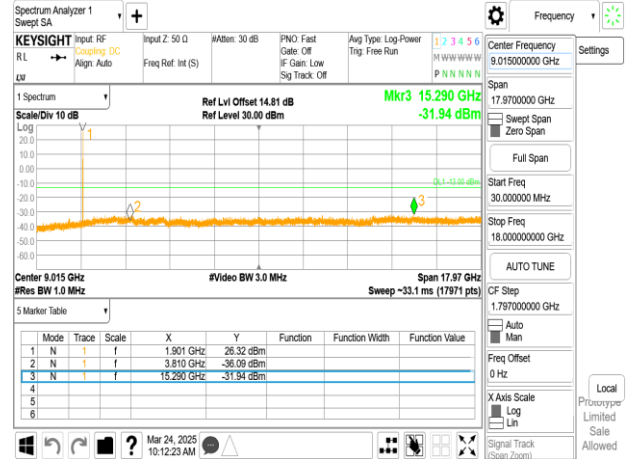
Band2_10MHz_DFT_s_OFDM_SCS15kHz_BPSK_RB1_1_CH381000upper 18G
