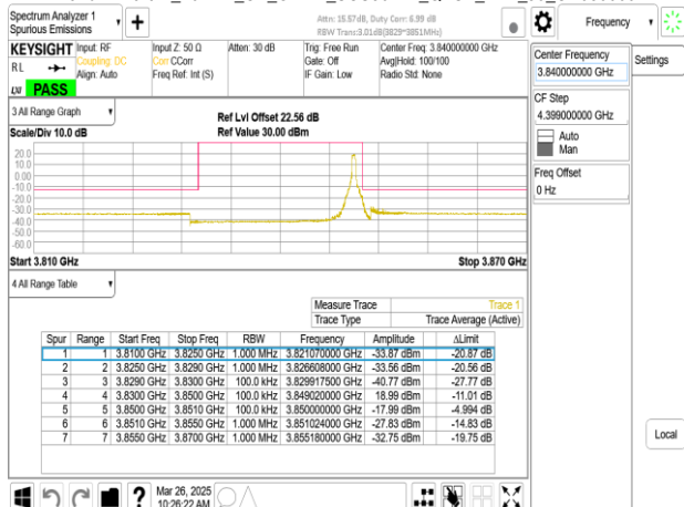
Band77-Part27_20MHz_CP_OFDM_SCS30kHz_QPSK_RB51_0_CH656000
