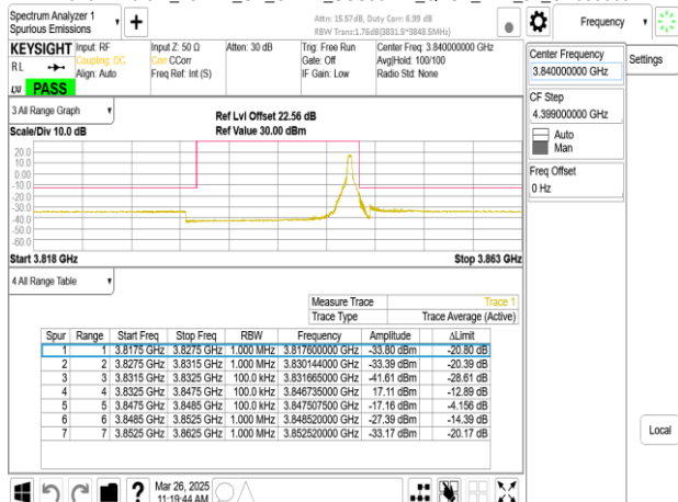
Band77-Part27_15MHz_CP_OFDM_SCS30kHz_QPSK_RB38_0_CH656000
