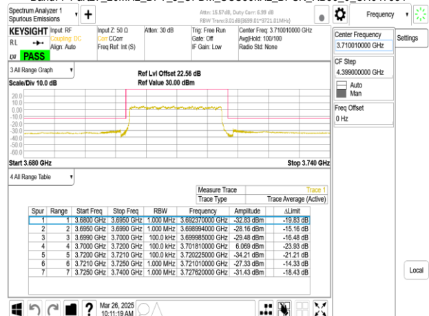
Band77-Part27_20MHz_DFT_s_OFDM_SCS30kHz_BPSK_RB50_0_CH647334
