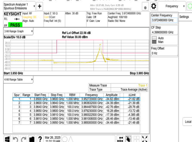
Band77-Part27_15MHz_CP_OFDM_SCS30kHz_QPSK_RB38_0_CH664832
