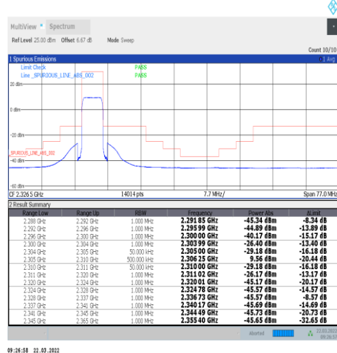
1-N30-15-5-L-6-CP-QPSK-Outer_Full-25@0-Ant1-PASS-see graph
