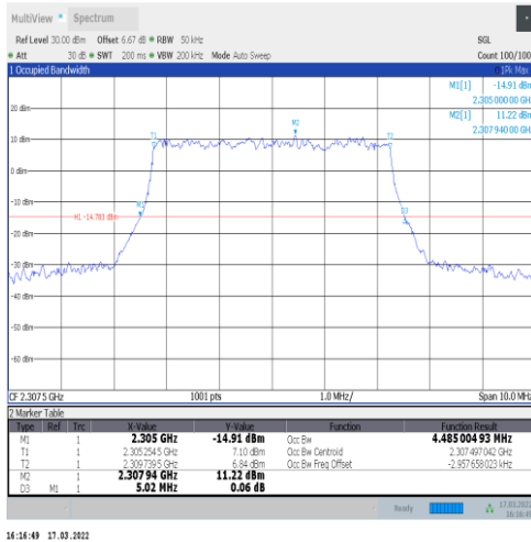
1-N30-15-5-L-3-DFT-16QAM-Outer_Full-25@0-Ant1- 4.485-5.020-≤5-PASS
