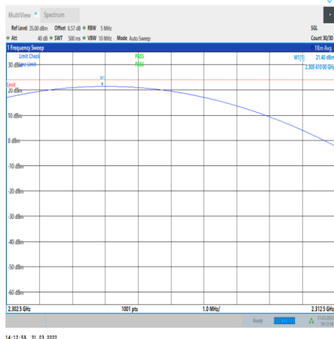
1-N30-PC3-15-5-L-1-DFT-PI2BPSK-Inner_1RB_Left -1@1-2302.5-2312.5-Ant1-21.40-23.98-PASS
