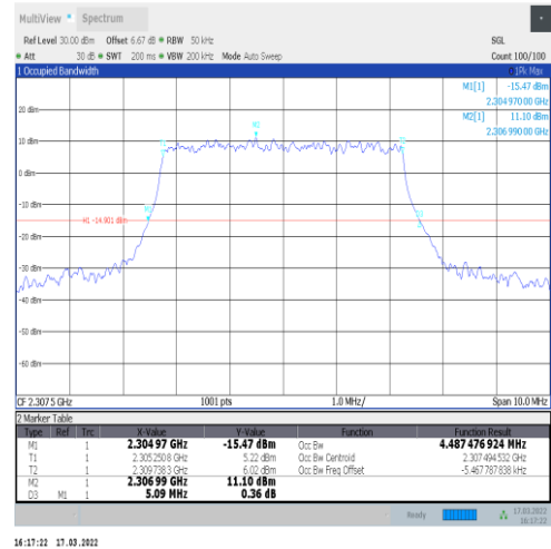
1-N30-15-5-L-4-DFT-64QAM-Outer_Full-25@0-Ant1 -4.487-5.090-≤5-PASS
