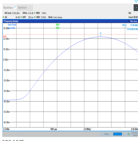
1-N30-PC3-15-10-M-2-DFT-PI2BPSK-Inner_1RB_Ri ght-1@50-2300-2320-Ant1-21.69-23.98-PASS
