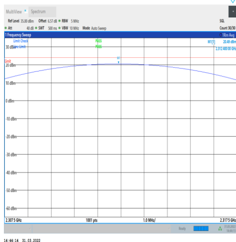
1-N30-PC3-15-5-H-3-DFT-PI2BPSK-Outer_Full-25 @0-2307.5-2317.5-Ant1-20.49-23.98-PASS
