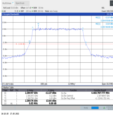
1-N30-15-5-L-1-DFT-QPSK-Outer_Full-25@0-Ant1-4 .483-5.030-≤5-PASS
