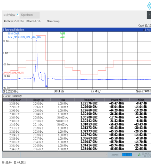
1-N30-15-5-L-1-DFT-PI2BPSK-Edge_1RB_Left-1@0-Ant1-PASS-see graph
