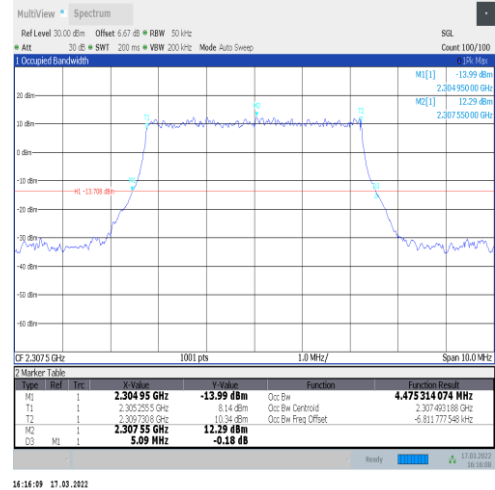
1-N30-15-5-L-2-DFT-PI2BPSK-Outer_Full-25@0-Ant 1-4.475-5.090-≤5-PASS
