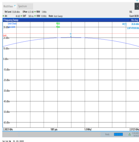
1-N30-PC3-15-5-L-3-DFT-PI2BPSK-Outer_Full-25 @0-2302.5-2312.5-Ant1-20.26-23.98-PASS
