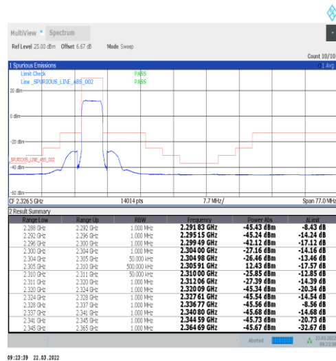
1-N30-15-5-L-3-DFT-PI2BPSK-Outer_Full-25@0-Ant1-PASS-see graph
