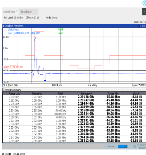
1-N30-15-5-L-4-CP-QPSK-Edge_1RB_Left-1@0-Ant1-PASS-see graph
