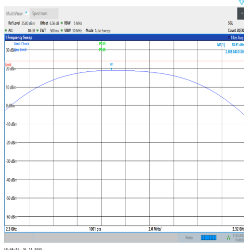
1-N30-PC3-15-10-M-3-DFT-PI2BPSK-Outer_Full-50 @0-2300-2320-Ant1-18.91-23.98-PASS
