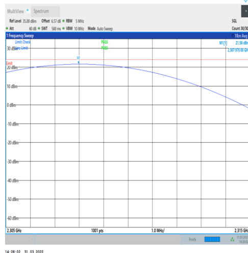
1-N30-PC3-15-5-M-1-DFT-PI2BPSK-Inner_1RB_Left- 1@1-2305-2315-Ant1-21.58-23.98-PASS
