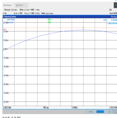
1-N30-PC3-15-5-L-2-DFT-PI2BPSK-Inner_1RB_Right t-1@23-2302.5-2312.5-Ant1-21.40-23.98-PASS
