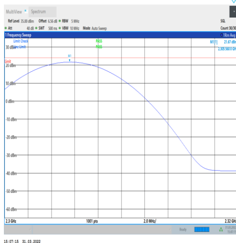
1-N30-PC3-15-10-M-1-DFT-PI2BPSK-Inner_1RB_Lef t-1@1-2300-2320-Ant1-21.67-23.98-PASS
