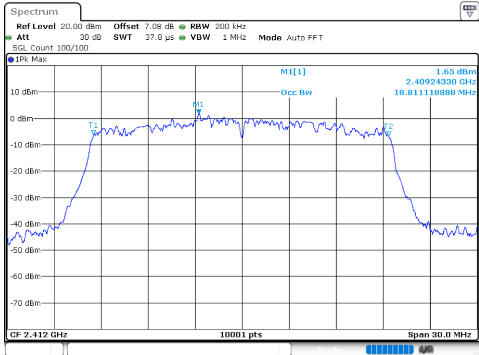
OBW NVNT ax20 2412MHz Ant 1
