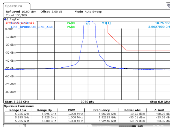
BE-NR-HIGH, SISO-B, 802.11ax20-MCS0, Ch173
