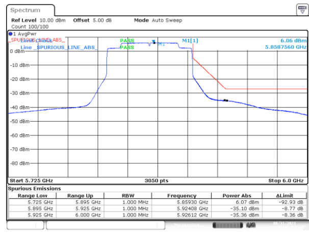
BE-NR-HIGH, MIMO-B, 802.11ax80-MCS0, Ch171
