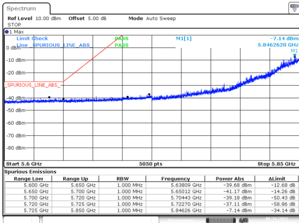
BE-NR-LOW, SISO-B, 802.11ax40-MCS0, Ch175
