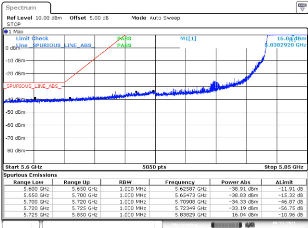
BE-NR-LOW, MIMO-B, 802.11ac80-VHT0, Ch171
