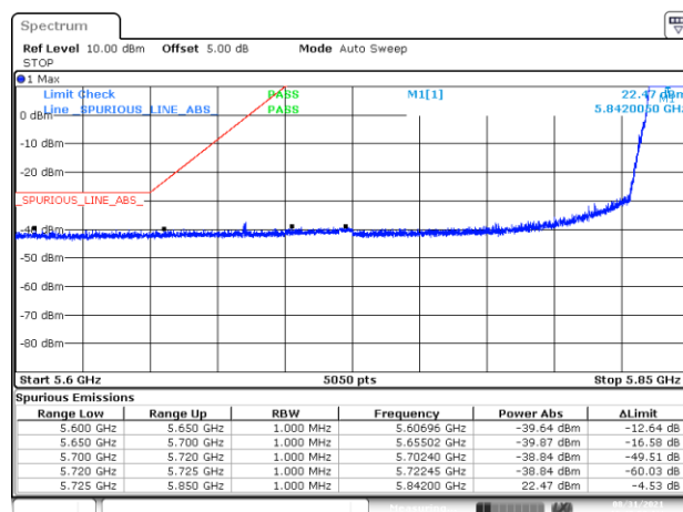
BE-NR-LOW, SISO-B, 802.11ax20-MCS0, Ch169
