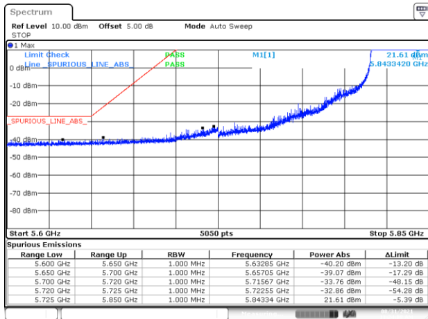
BE-NR-LOW, MIMO-B, 802.11ax40-MCS0, Ch167
