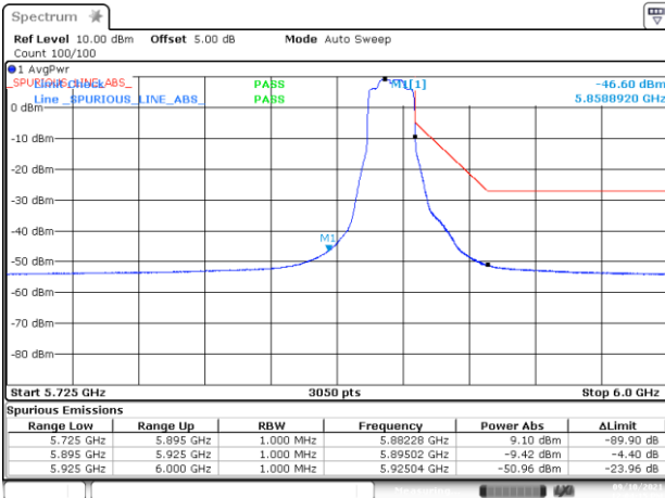
BE-NR-HIGH, MIMO-B, 802.11ax20-MCS0, Ch177
