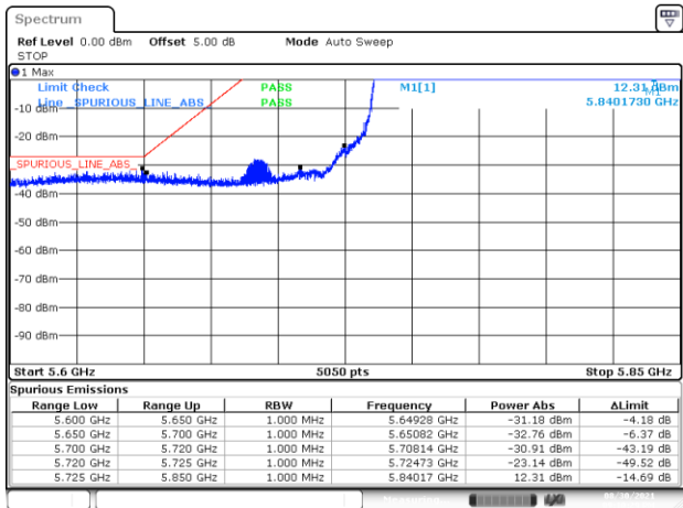
BE-NR-LOW, SISO-A, 802.11ax160-MCS0, Ch163
