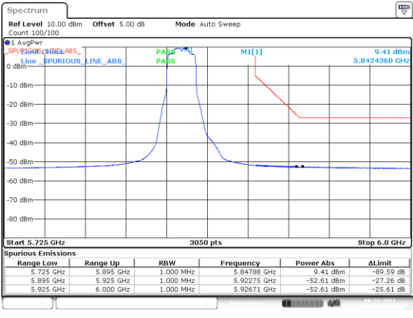
BE-NR-HIGH, MIMO-B, 802.11ax20-MCS0, Ch169
