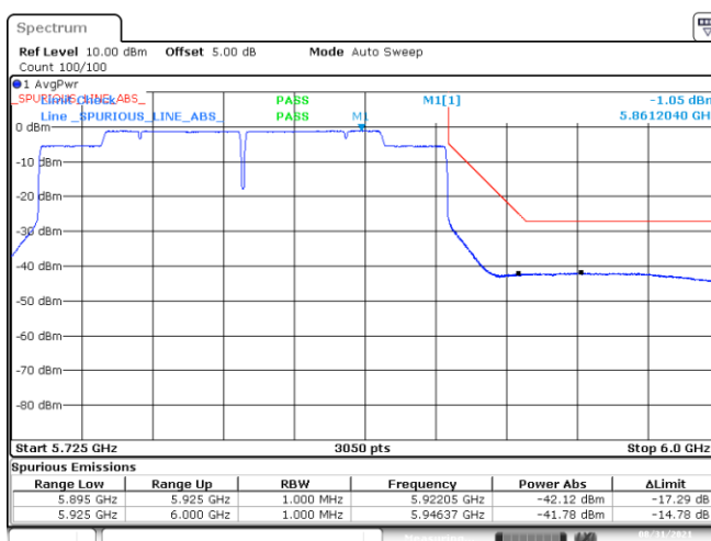
BE-NR-HIGH, MIMO-A, 802.11ax160-MCS0, Ch163
