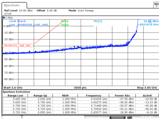
BE-NR-LOW, MIMO-B, 802.11ax80-MCS0, Ch171
