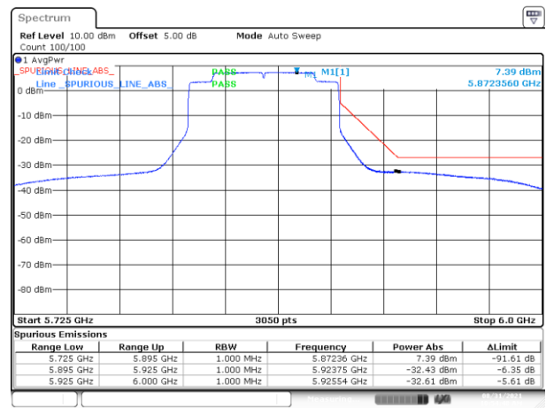
BE-NR-HIGH, SISO-B, 802.11ax80-MCS0, Ch171
