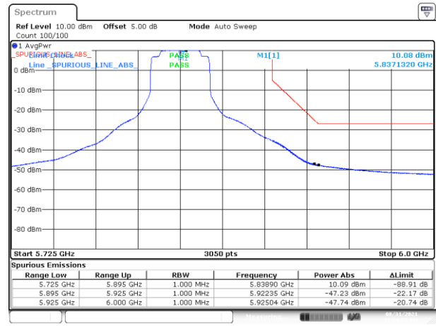
BE-NR-HIGH, MIMO-B, 802.11ax40-MCS0, Ch167
