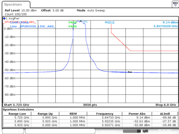
BE-NR-HIGH, MIMO-A, 802.11ax20-MCS0, Ch169
