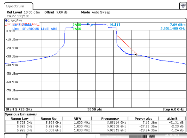
BE-NR-HIGH, SISO-A, 802.11ax80-MCS0, Ch171
