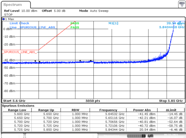
BE-NR-LOW, MIMO-B, 802.11ax20-MCS0, Ch169
