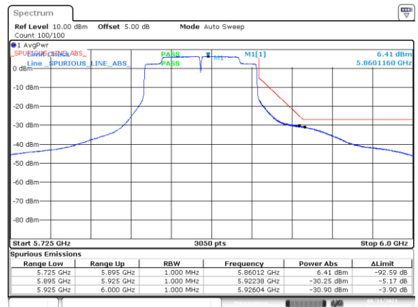
BE-NR-HIGH, MIMO-A, 802.11ac80-VHT0, Ch171
