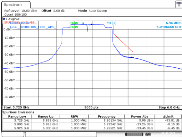
BE-NR-HIGH, MIMO-B, 802.11ac80-VHT0, Ch171
