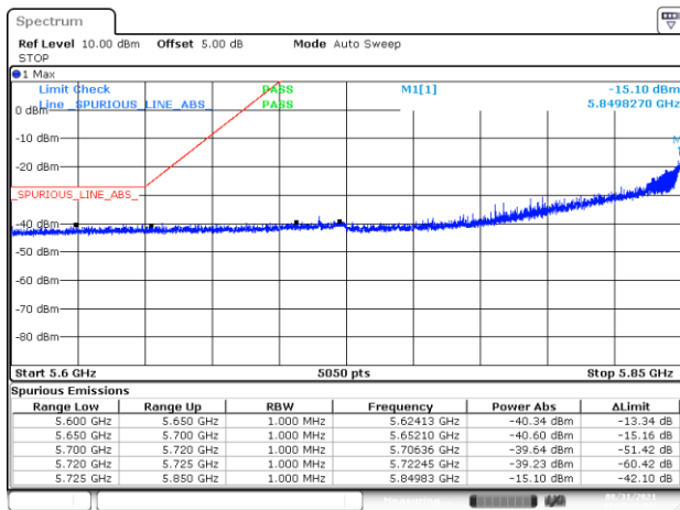
BE-NR-LOW, MIMO-B, 802.11ax40-MCS0, Ch175
