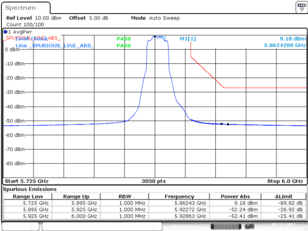
BE-NR-HIGH, MIMO-B, 802.11ax20-MCS0, Ch173
