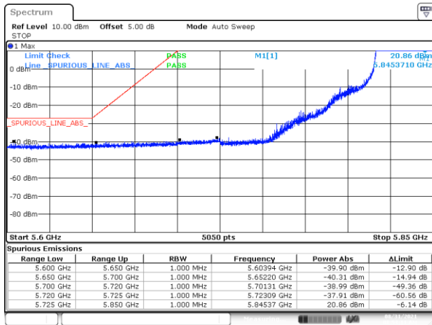
BE-NR-LOW, MIMO-A, 802.11n40-HT0, Ch167
