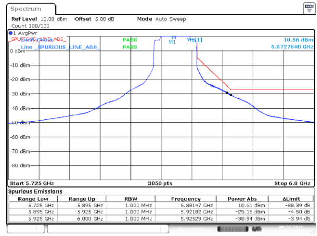
BE-NR-HIGH, SISO-B, 802.11ax40-MCS0, Ch175
