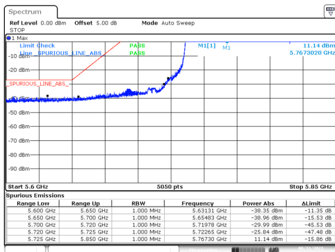
BE-NR-LOW, MIMO-A, 802.11ax160-MCS0, Ch163
