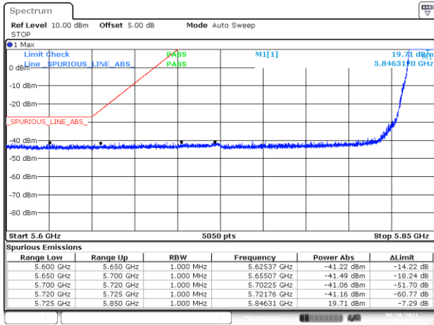
BE-NR-LOW, MIMO-A, 802.11ax20-MCS0, Ch169
