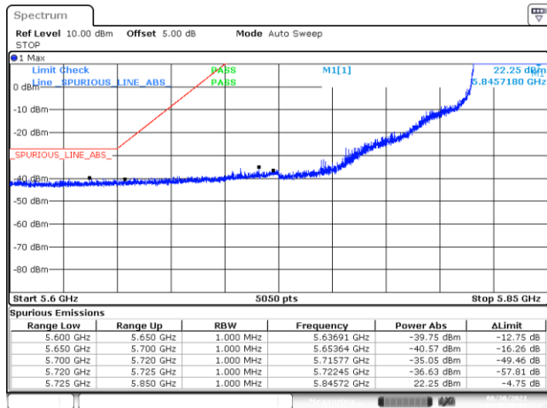
BE-NR-LOW, SISO-A, 802.11ax40-MCS0, Ch167
