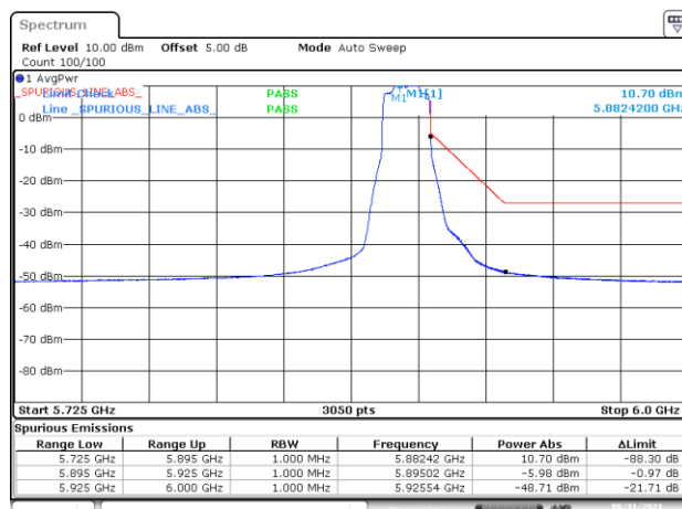
BE-NR-HIGH, SISO-B, 802.11ax20-MCS0, Ch177
