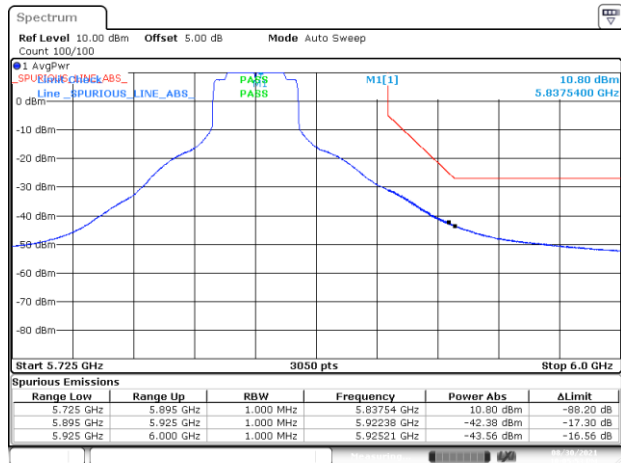
BE-NR-HIGH, MIMO-A, 802.11ax40-MCS0, Ch167
