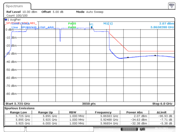
BE-NR-HIGH, SISO-B, 802.11ax160-MCS0, Ch163
