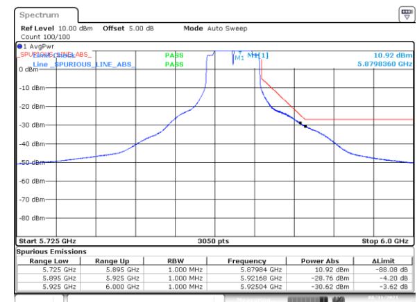
BE-NR-HIGH, SISO-B, 802.11n40-HT0, Ch175
