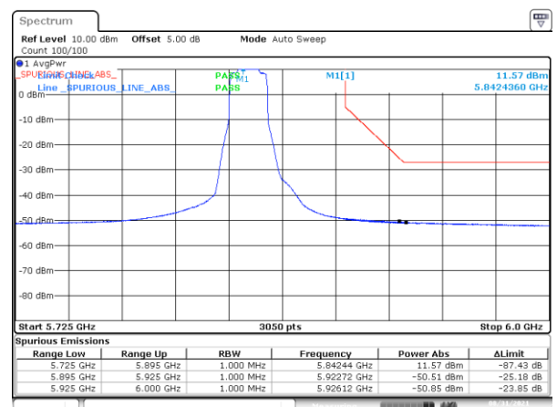
BE-NR-HIGH, SISO-B, 802.11ax20-MCS0, Ch169
