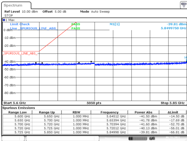
BE-NR-LOW, MIMO-A, 802.11ax20-MCS0, Ch177
