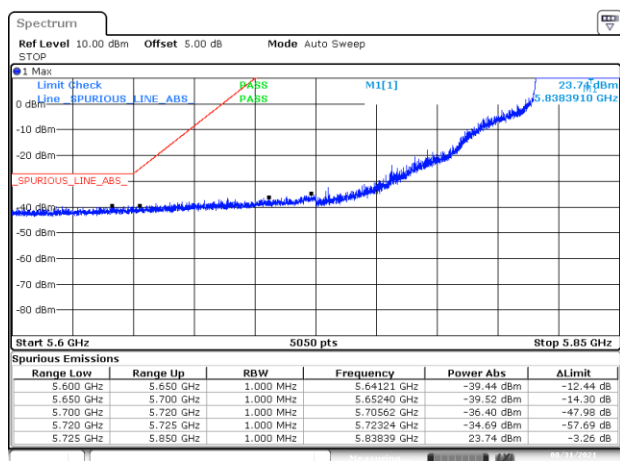
BE-NR-LOW, SISO-B, 802.11ax40-MCS0, Ch167
