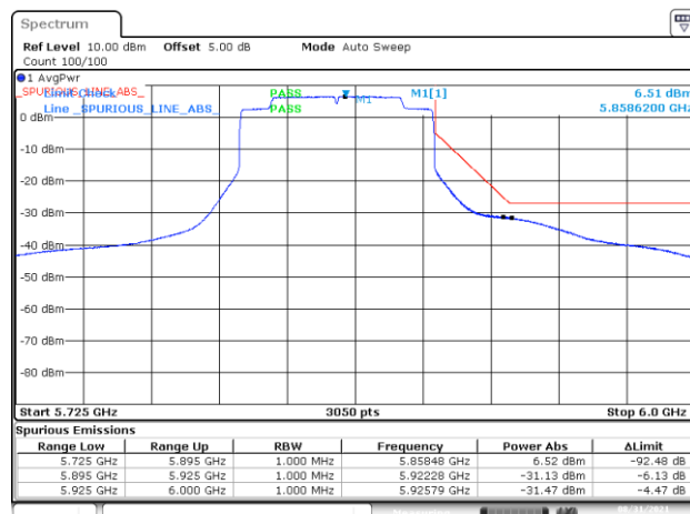
BE-NR-HIGH, MIMO-A, 802.11ax80-MCS0, Ch171
