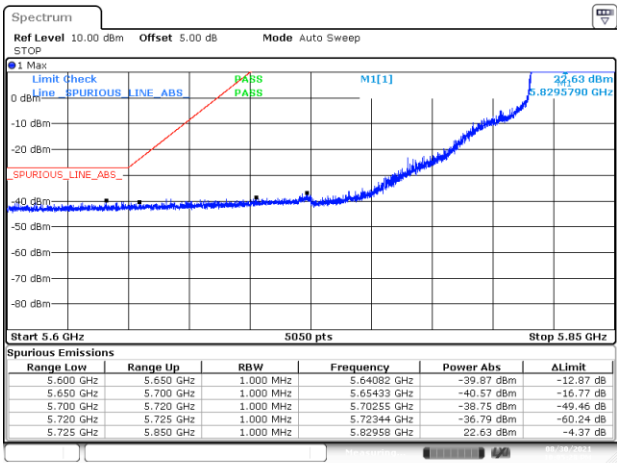
BE-NR-LOW, MIMO-A, 802.11ax40-MCS0, Ch167
