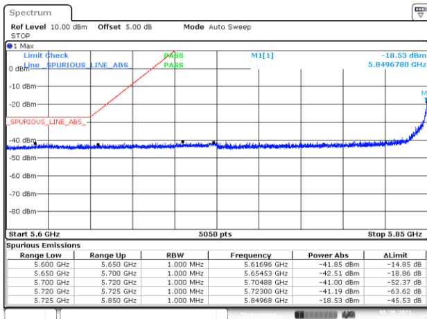
BE-NR-LOW, MIMO-A, 802.11ax20-MCS0, Ch173
