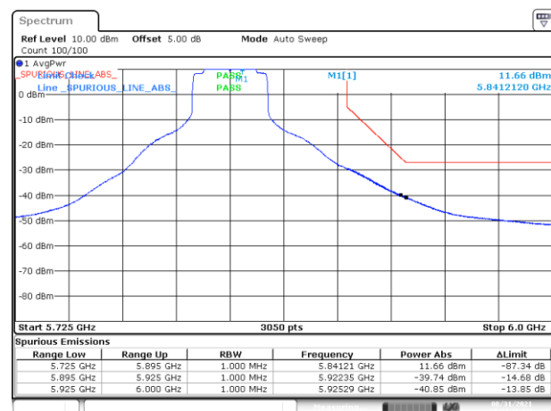
BE-NR-HIGH, SISO-B, 802.11ax40-MCS0, Ch167
