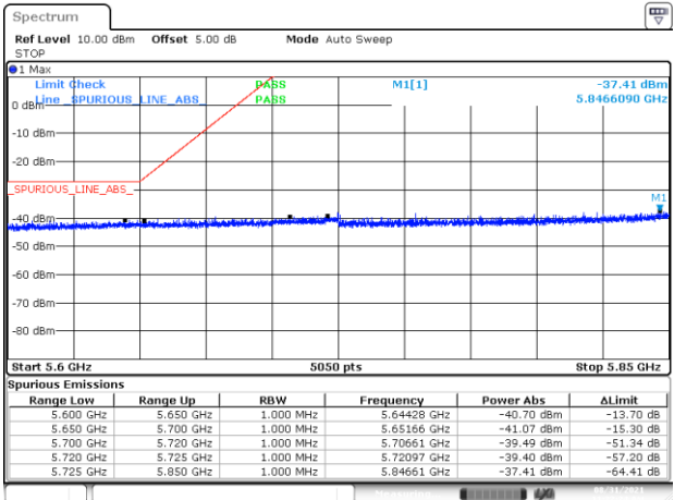
BE-NR-LOW, MIMO-B, 802.11ax20-MCS0, Ch177
