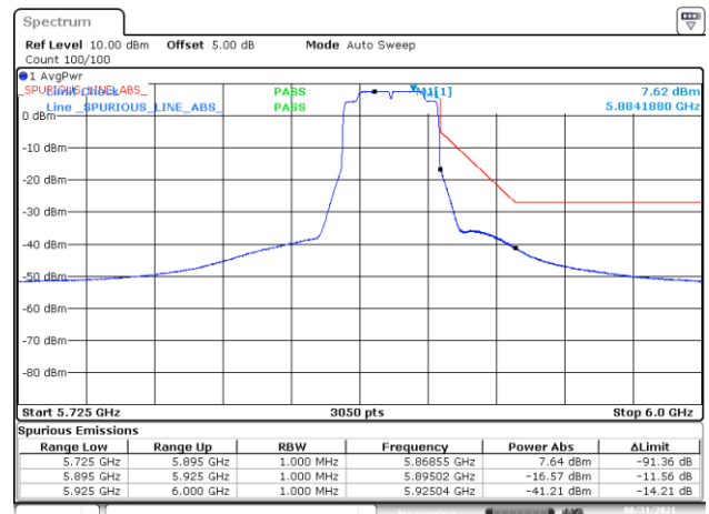
BE-NR-HIGH, MIMO-B, 802.11ax40-MCS0, Ch175
