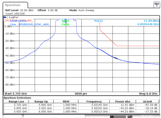
BE-NR-HIGH, SISO-B, 802.11n40-HT0, Ch167
