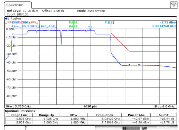
BE-NR-HIGH, MIMO-A, 802.11n20-HT0, Ch169
