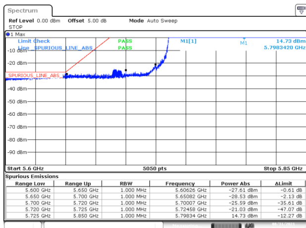
BE-NR-LOW, SISO-B, 802.11ax160-MCS0, Ch163
