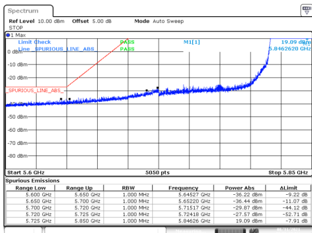
BE-NR-LOW, MIMO-A, 802.11ax80-MCS0, Ch171
