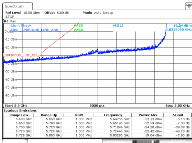
BE-NR-LOW, SISO-B, 802.11ax80-MCS0, Ch171
