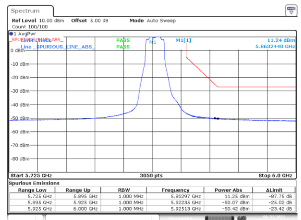
BE-NR-HIGH, SISO-B, 802.11n20-HT0, Ch173
