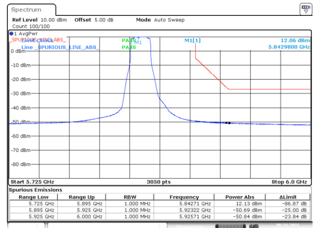
BE-NR-HIGH, SISO-B, 802.11n20-HT0, Ch169
