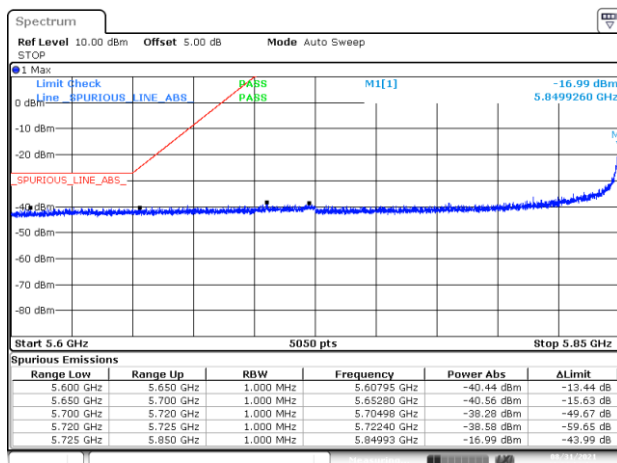
BE-NR-LOW, SISO-B, 802.11ax20-MCS0, Ch173
