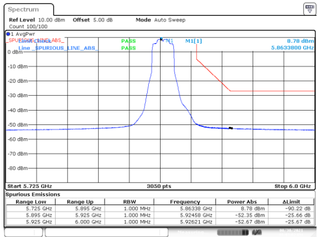
BE-NR-HIGH, MIMO-A, 802.11ax20-MCS0, Ch173
