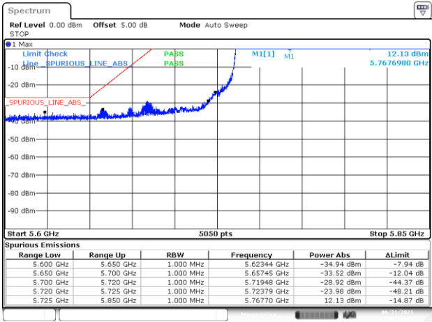
BE-NR-LOW, MIMO-B, 802.11ax160-MCS0, Ch163
