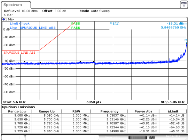
BE-NR-LOW, MIMO-B, 802.11ax20-MCS0, Ch173
