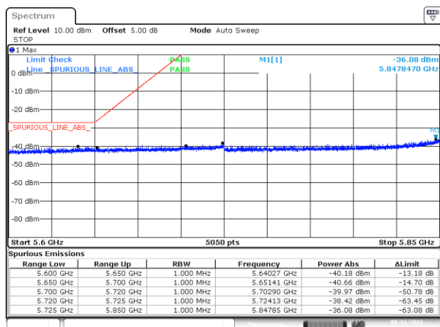
BE-NR-LOW, SISO-B, 802.11ax20-MCS0, Ch177
