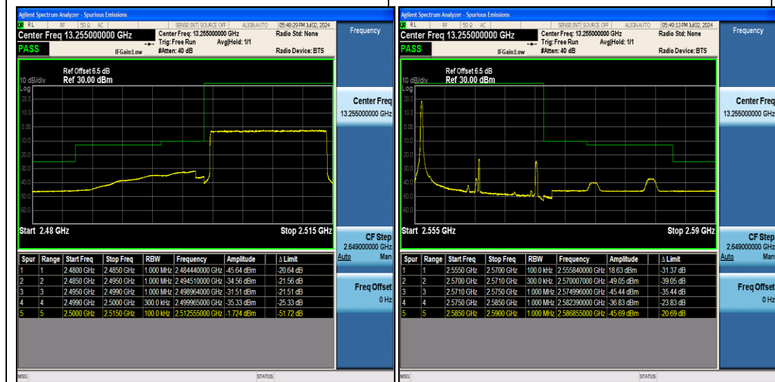
Band7_15MHz_QPSK_20825_75RB#0
