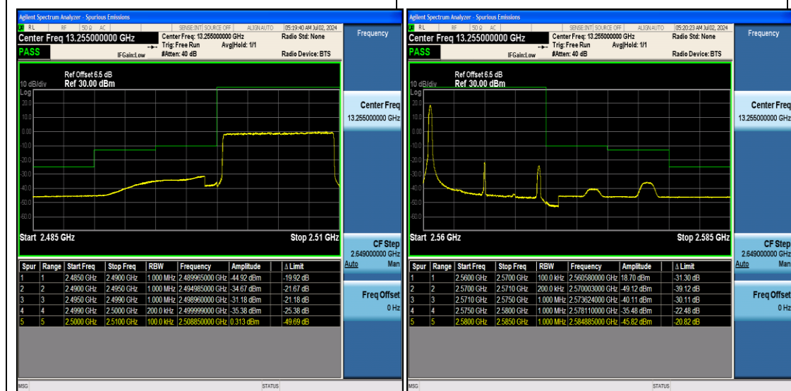
Band7_10MHz_QPSK_20800_1RB#0
