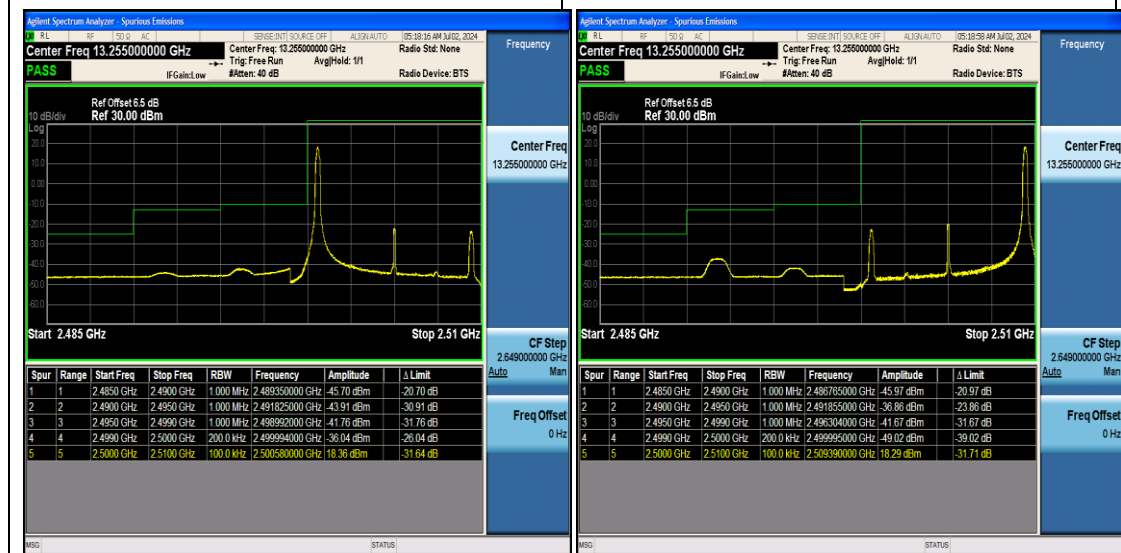
Band7_10MHz_QPSK_20800_1RB#0
