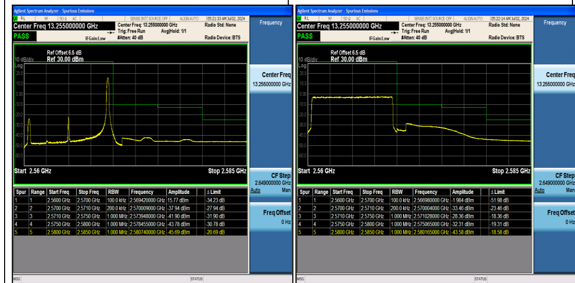
Band7_10MHz_64QAM_21400_1RB#49
