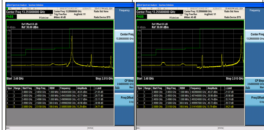
Band7_15MHz_16QAM_20825_1RB#0
