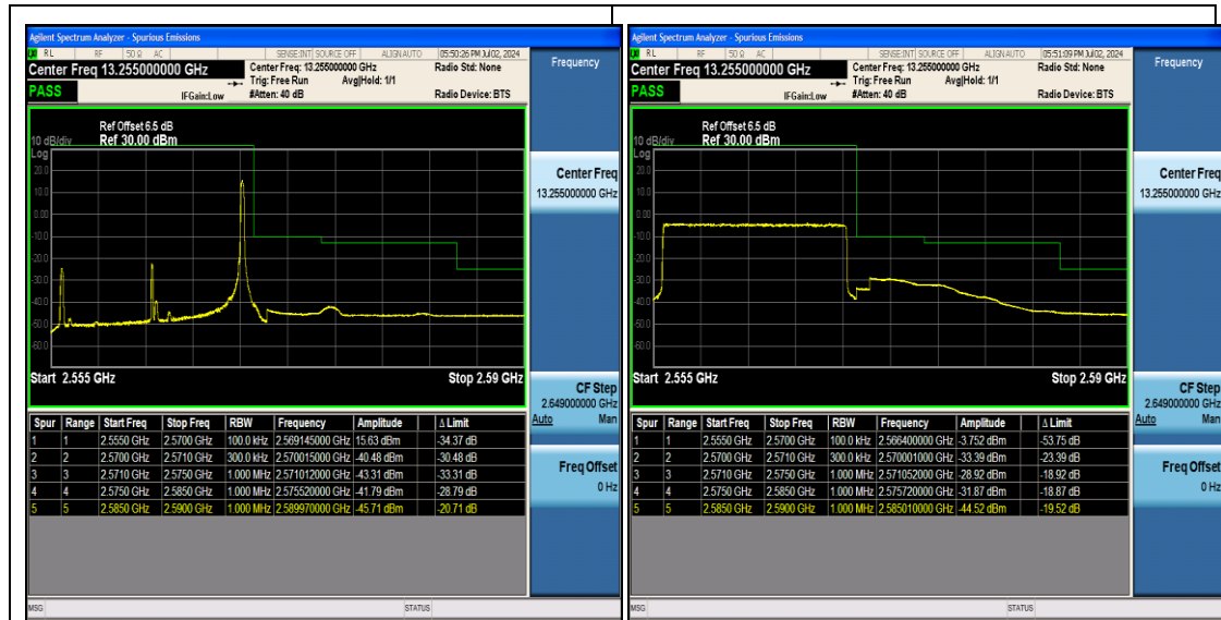
Band7_15MHz_64QAM_21375_1RB#74
