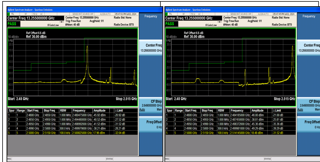
Band7_15MHz_QPSK_20825_1RB#0
