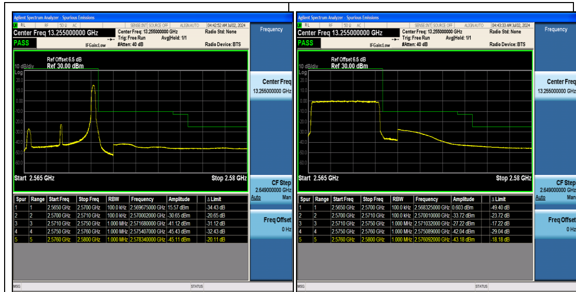
Band7_5MHz_16QAM_21425_1RB#24
