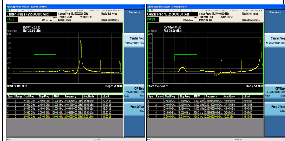
Band7_10MHz_64QAM_21400_1RB#49
