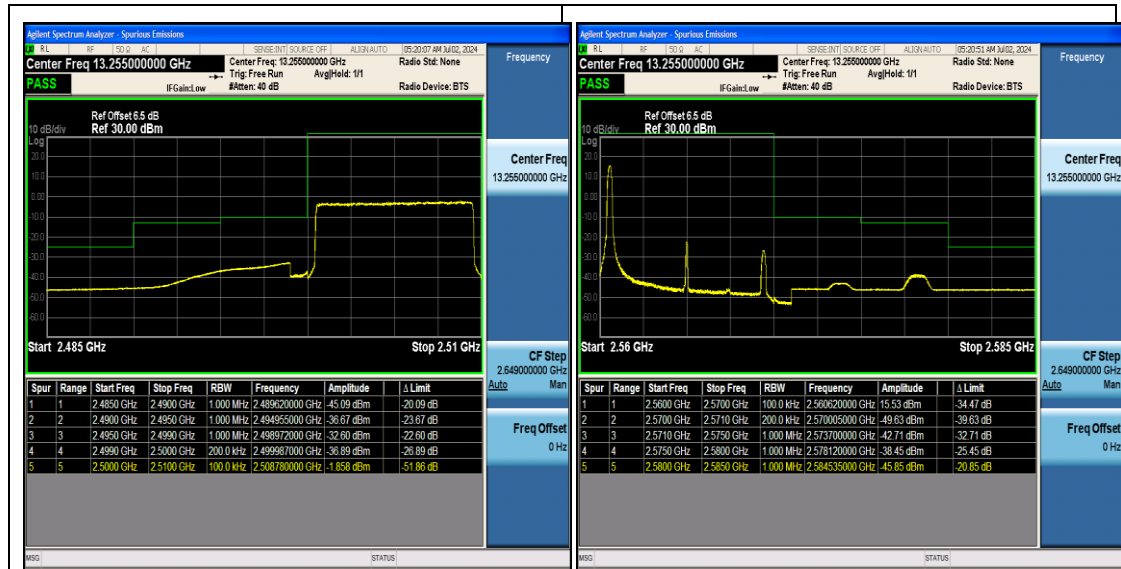
Band7_10MHz_64QAM_20800_50RB#0
