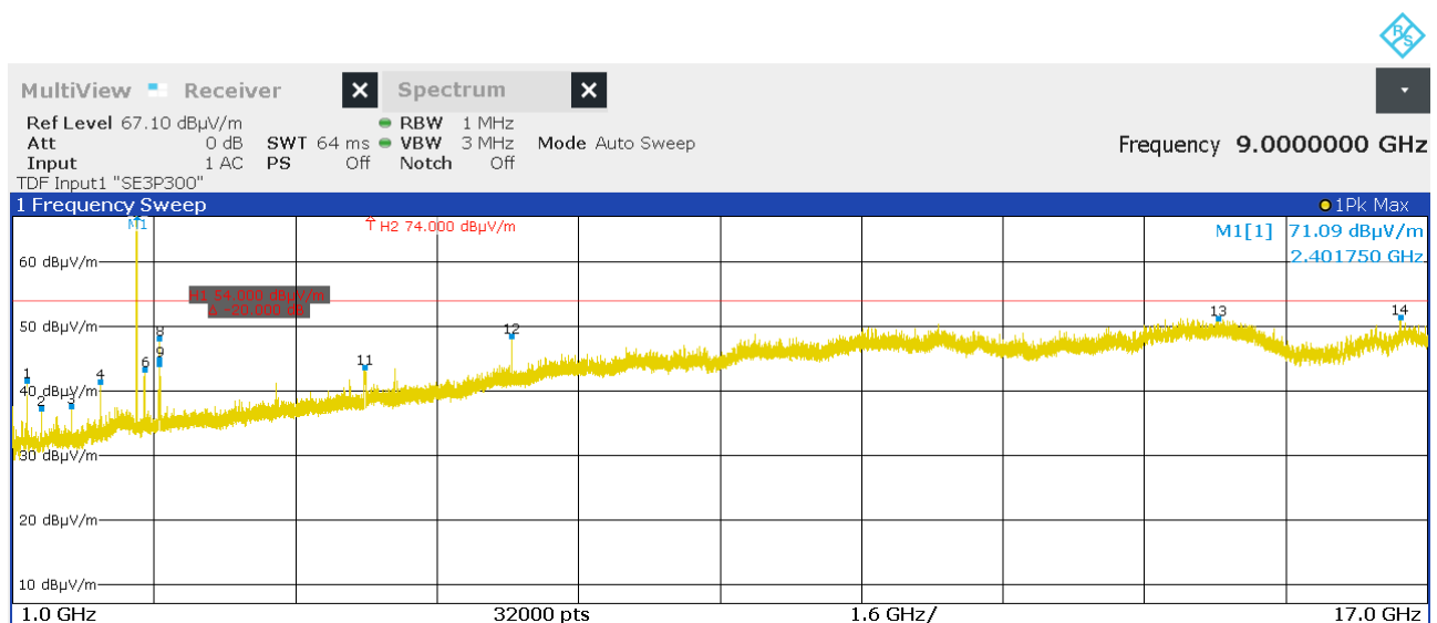
Figure 35: Chart of radiated emissions pre-measurement from 1 GHz to 17 GHz on lowest channel, EUT position Y, antenna polarization vertical
