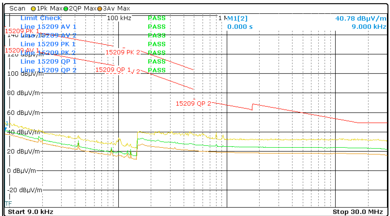
Figure 33: Chart of emissions test below 30 MHz on lowest channel, EUT position X, antenna parallel
