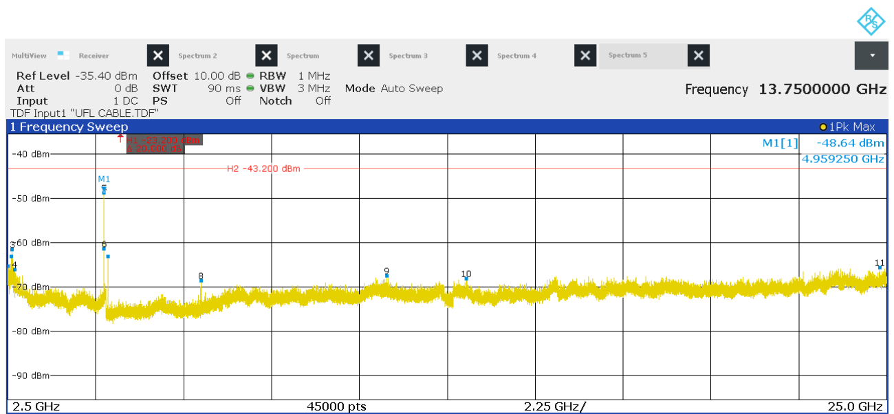
Figure 32: Chart of emissions test from 2.5 GHz to 25 GHz on highest channel, Pk
