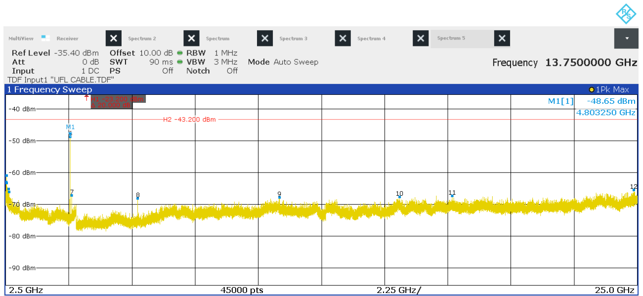
Figure 26: Chart of emissions test from 2.5 GHz to 25 GHz on lowest channel, Pk
