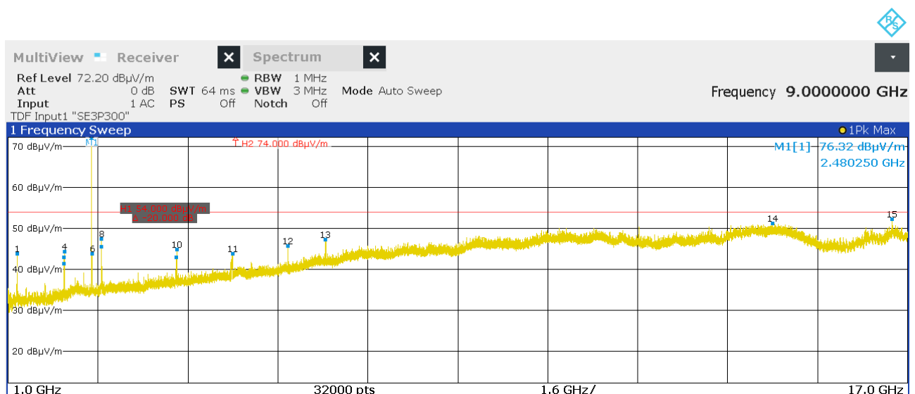
Figure 39: Chart of emissions test from 1 GHz to 17 GHz on highest channel, EUT position Y, antenna polarization vertical
