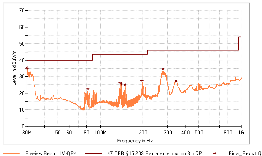
Figure 34: Chart of radiated emissions test from 30 MHz to 1 GHz on middle channel, EUT position Y, antenna polarization vertical
