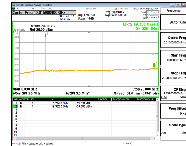
n78(3700-3800MHz) (30MHz-20GHz) 50M DFT-s-OFDM QPSK Inner_1RB_Right Mid
