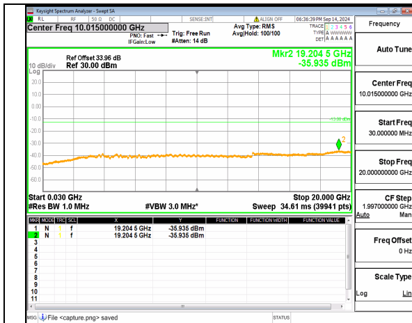
n78(3700-3800MHz) (30MHz-20GHz) 80M DFT-s-OFDM QPSK Inner_1RB_Right Mid
