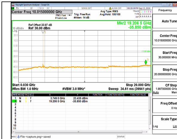
n78(3700-3800MHz) (30MHz-20GHz) 50M DFT-s-OFDM QPSK Inner_1RB_Right Low
