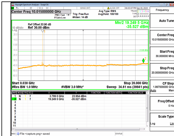
n78(3700-3800MHz) (30MHz-20GHz) 90M DFT-s-OFDM QPSK Inner_1RB_Right_High
