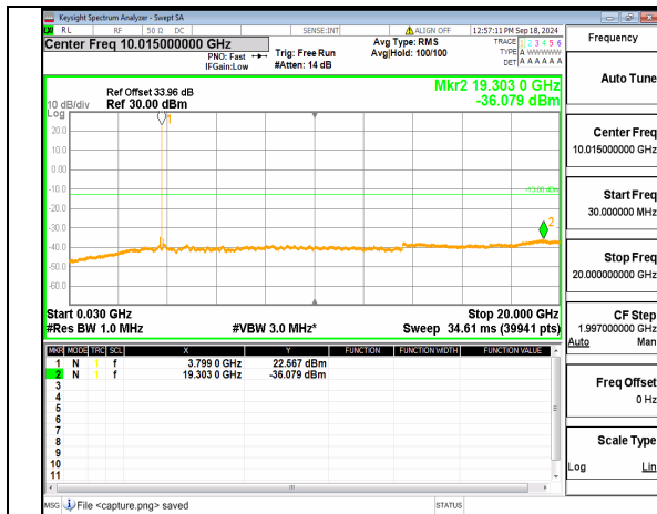
n78(3700-3800MHz) (30MHz-20GHz) 80M DFT-s-OFDM QPSK Inner_1RB_Right_High
