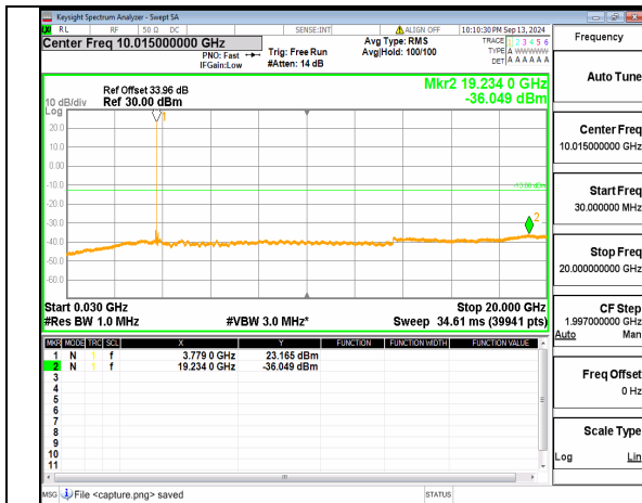
n78(3700-3800MHz) (30MHz-20GHz) 60M DFT-s-OFDM QPSK Inner_1RB_Right Mid
