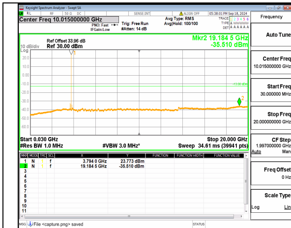
n78(3700-3800MHz) (30MHz-20GHz) 90M DFT-s-OFDM BPSK Inner_1RB_Right Mid
