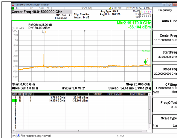
n78(3700-3800MHz) (30MHz-20GHz) 70M DFT-s-OFDM QPSK Inner_1RB_Right Mid
