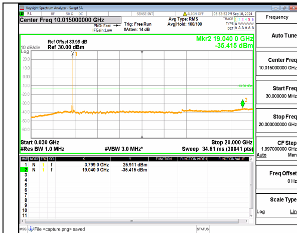
n78(3700-3800MHz) (30MHz-20GHz) 90M DFT-s-OFDM BPSK Inner_1RB_Right High
