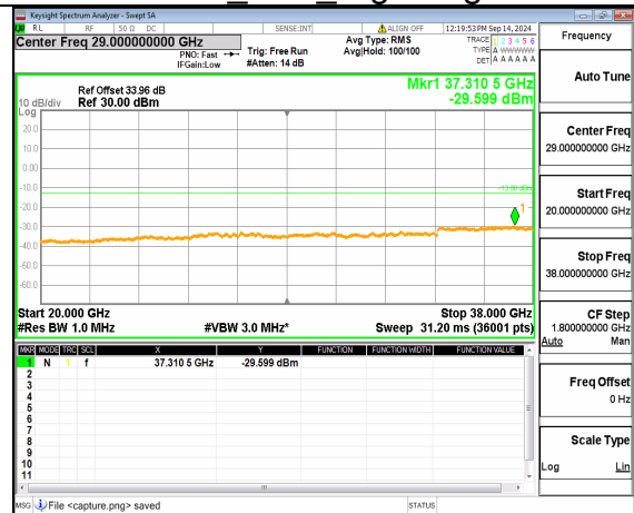
n78(3700-3800MHz) (20GHz-38GHz) 70M DFT-s-OFDM QPSK Inner_1RB_Left High
