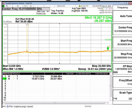
n78(3700-3800MHz) (30MHz-20GHz) 70M DFT-s-OFDM QPSK Inner_1RB_Left High
