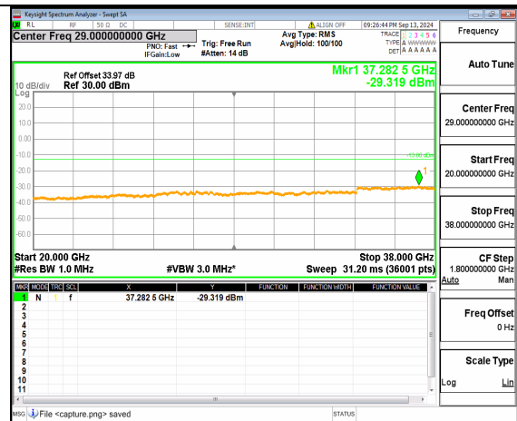
n78(3700-3800MHz) (20GHz-38GHz) 60M DFT-s-OFDM BPSK Inner_1RB_Right Low
