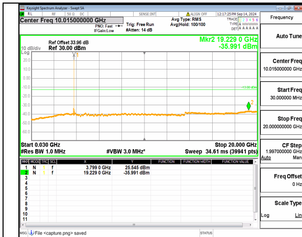
n78(3700-3800MHz) (30MHz-20GHz) 70M DFT-s-OFDM BPSK Inner_1RB_Right High
