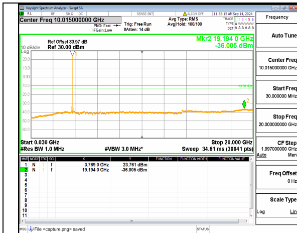
n78(3700-3800MHz) (30MHz-20GHz) 70M DFT-s-OFDM BPSK Inner_1RB_Right Low
