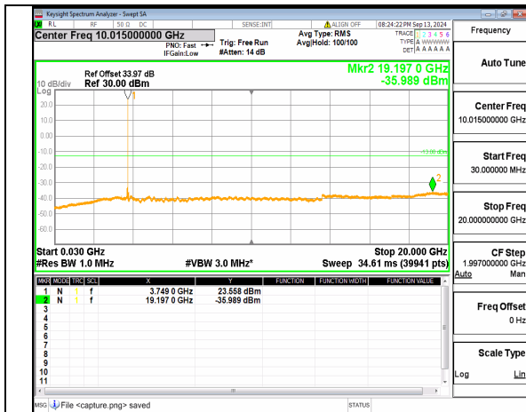
n78(3700-3800MHz) (30MHz-20GHz) 50M DFT-s-OFDM BPSK Inner_1RB_Right Low
