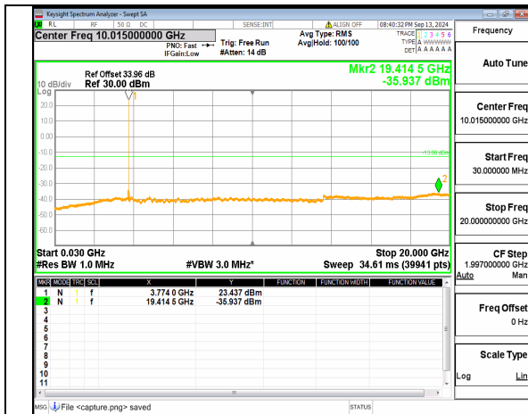
n78(3700-3800MHz) (30MHz-20GHz) 50M DFT-s-OFDM BPSK Inner_1RB_Right Mid
