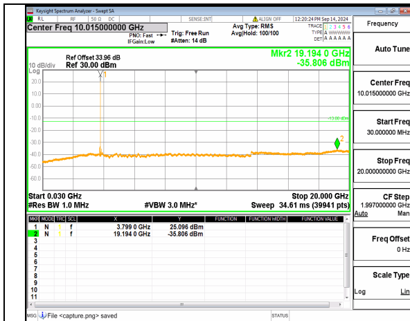
n78(3700-3800MHz) (30MHz-20GHz) 70M DFT-s-OFDM QPSK Inner_1RB_Right_High
