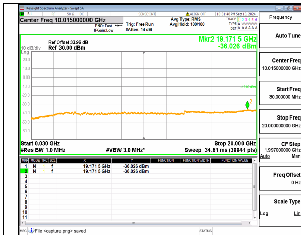
n78(3700-3800MHz) (30MHz-20GHz) 60M DFT-s-OFDM QPSK Inner_1RB_Right_High
