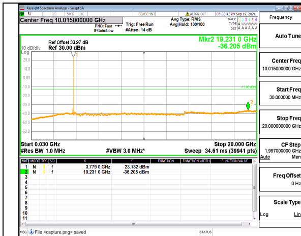
n78(3700-3800MHz) (30MHz-20GHz) 80M DFT-s-OFDM BPSK Inner_1RB_Right Low
