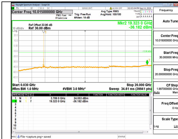
n78(3700-3800MHz) (30MHz-20GHz) 80M DFT-s-OFDM BPSK Inner_1RB_Right Mid
