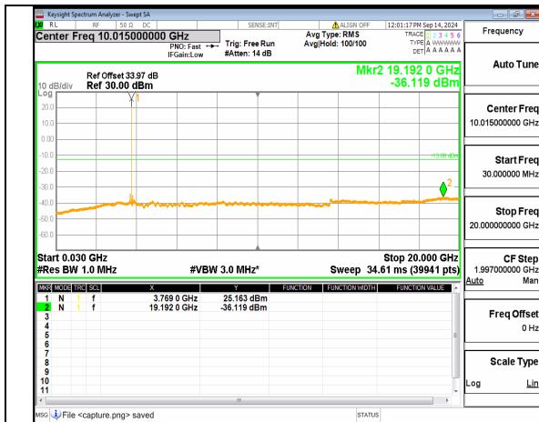
n78(3700-3800MHz) (30MHz-20GHz) 70M DFT-s-OFDM QPSK Inner_1RB_Right Low
