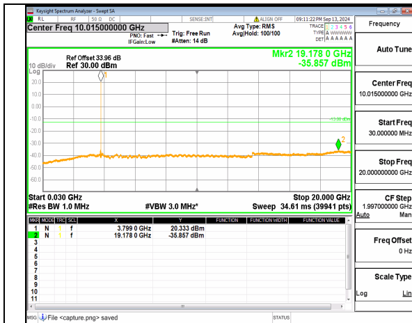
n78(3700-3800MHz) (30MHz-20GHz) 50M DFT-s-OFDM QPSK Inner_1RB_Right_High
