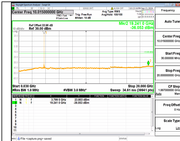
n78(3700-3800MHz) (30MHz-20GHz) 60M DFT-s-OFDM BPSK Inner_1RB_Right High
