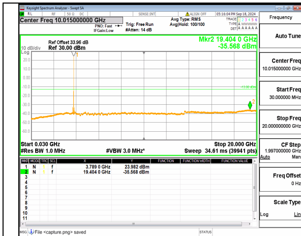
n78(3700-3800MHz) (30MHz-20GHz) 90M DFT-s-OFDM BPSK Inner_1RB_Right Low
