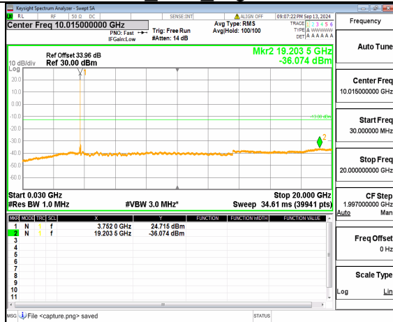
n78(3700-3800MHz) (30MHz-20GHz) 50M DFT-s-OFDM BPSK Inner_1RB_Left High
