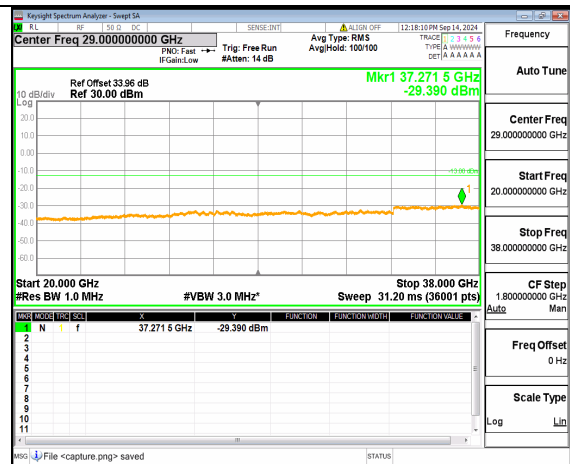
n78(3700-3800MHz) (20GHz-38GHz) 70M DFT-s-OFDM BPSK Inner_1RB_Right High
