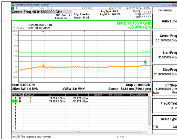
n78(3700-3800MHz) (30MHz-20GHz) 60M DFT-s-OFDM BPSK Inner_1RB_Right Low
