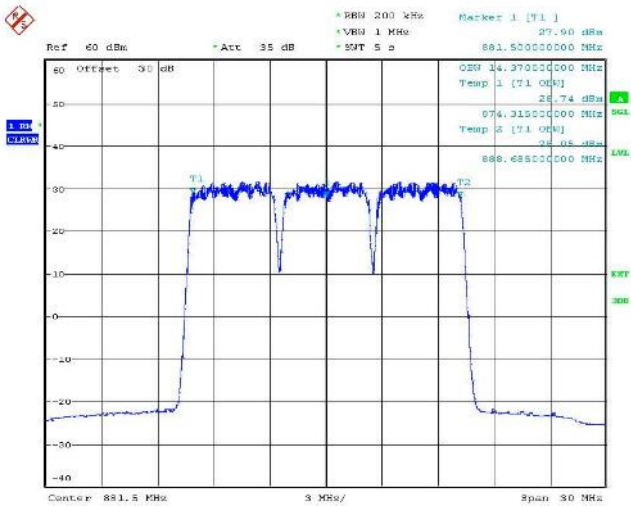
Figure 113 Occupied Bandwidth – QPSK (876.5/881.5/886.5 MHz) (5+5+5MHz Channel BW)
