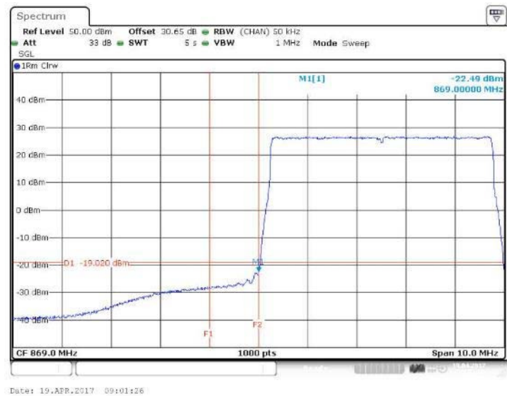
Figure 141 Spurious Emissions (Lower Band Edge) – 64QAM (871.5 MHz, 5 MHz Channel BW)
