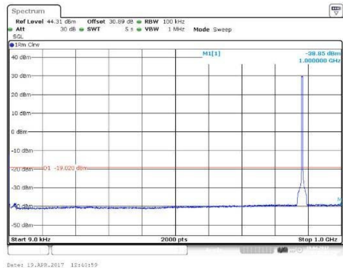
Figure 159 Spurious Emissions (9kHz – 1GHz) – 64QAM (881.5.0 MHz, 5 MHz Channel BW)
