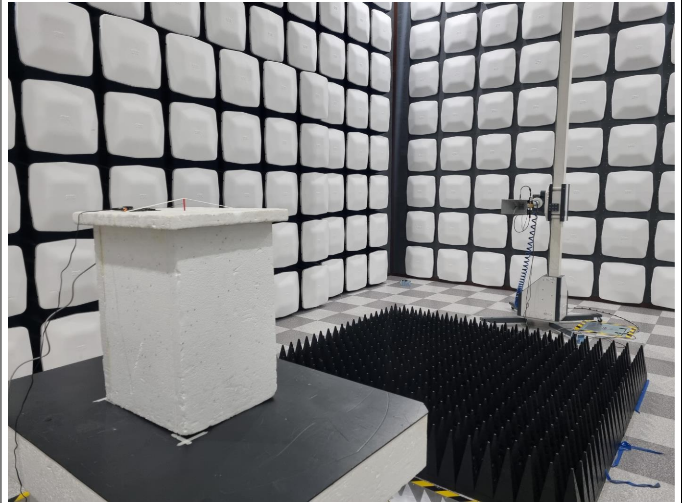
Above 1 GHz
