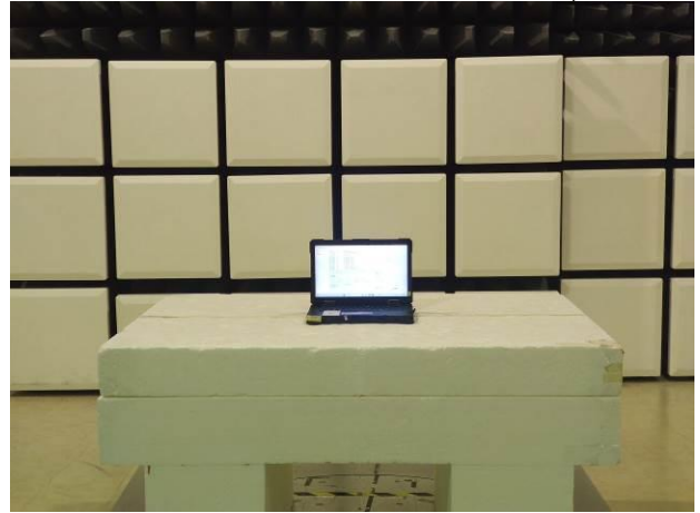
FCC_15_225+RSS_210_NFC_Radiated_Setup
