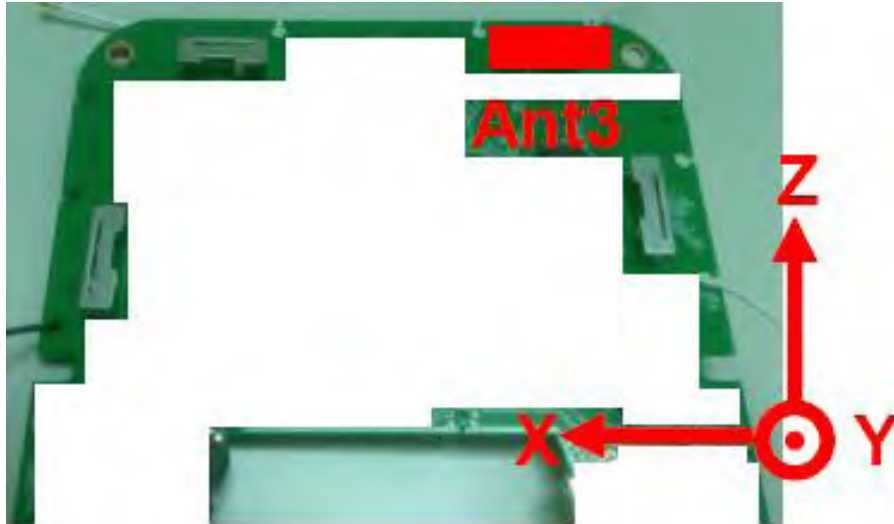
Antenna Configuration
