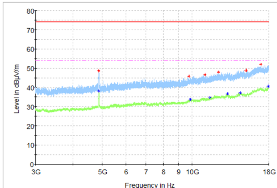
Fig.51 Radiated Spurious Emission (802.11g, CH6, 3GHz-18GHz)
