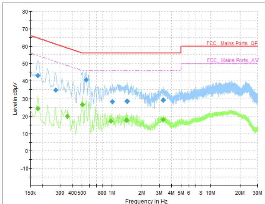
Fig.69 AC Power line Conducted Emission (Traffic, AE3, 120V)
