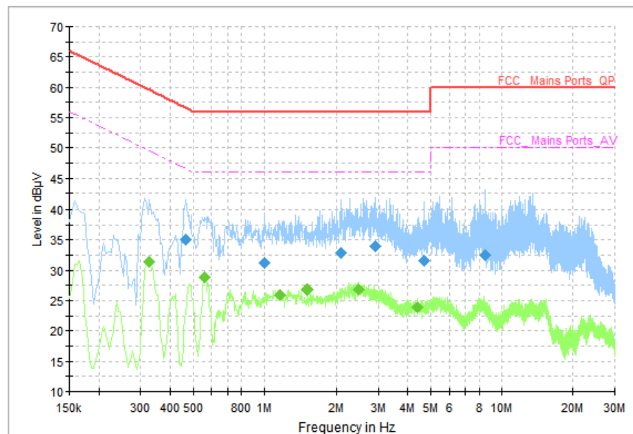
Fig.70 AC Power line Conducted Emission (Idle, AE3, 120V)
