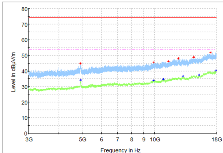
Fig.61 Radiated Spurious Emission (802.11n HT40, CH6, 3GHz-18GHz)
