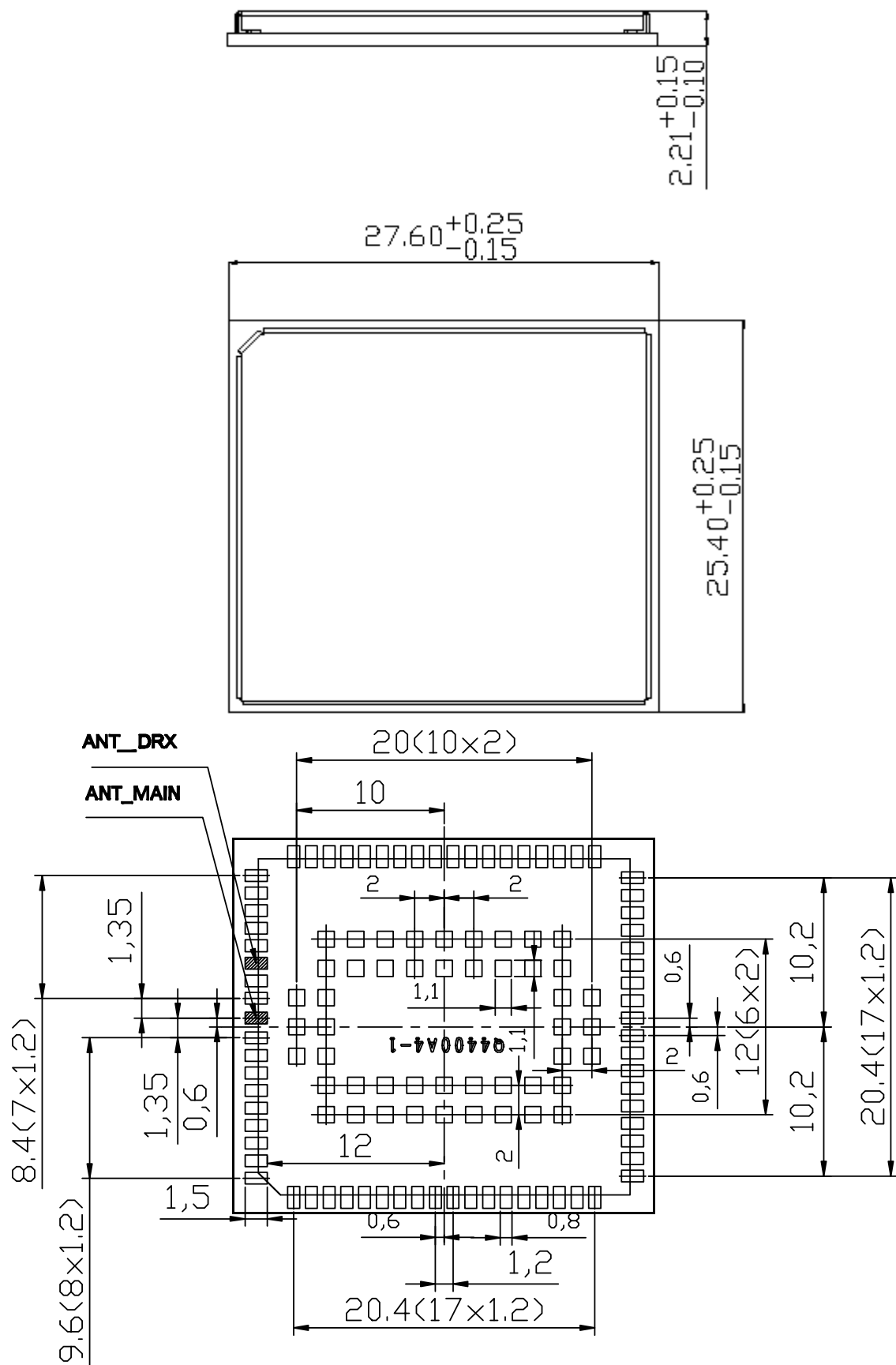
Figure 42: Dimensions of ELS61-AUS (all dimensions in mm)
