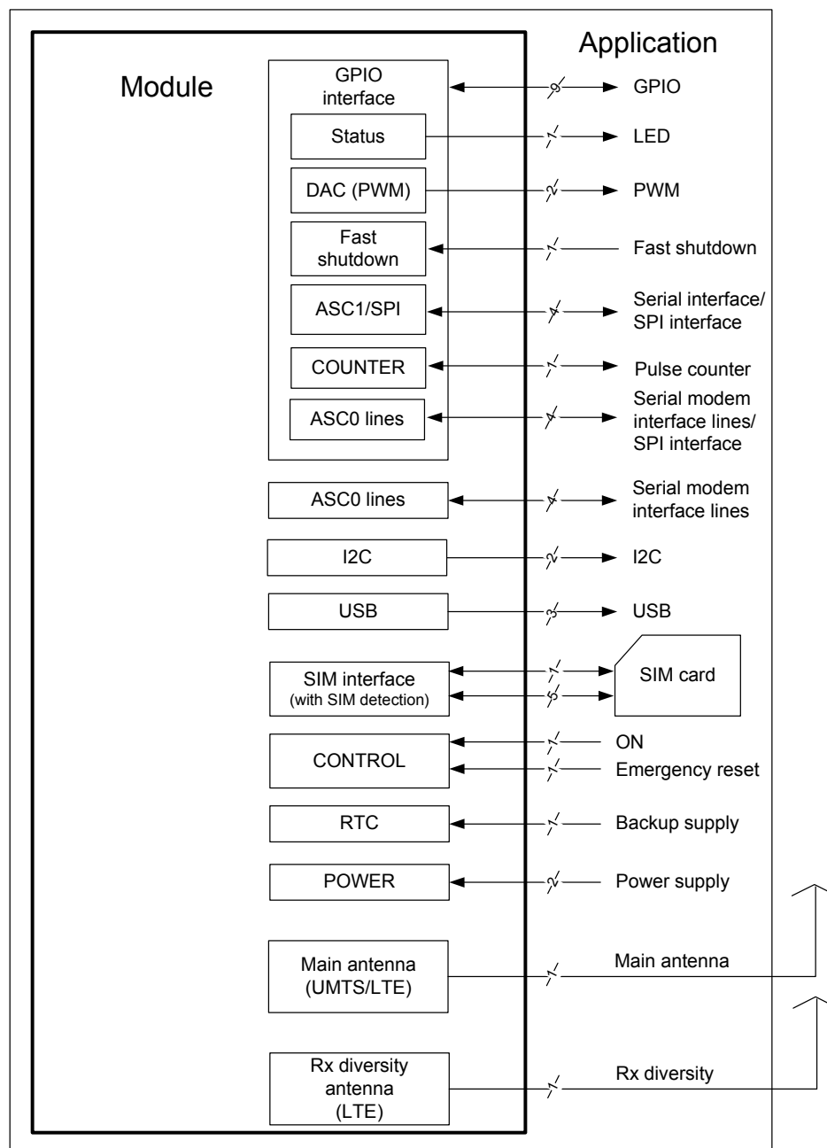
Figure 1: ELS61-AUS system overview
