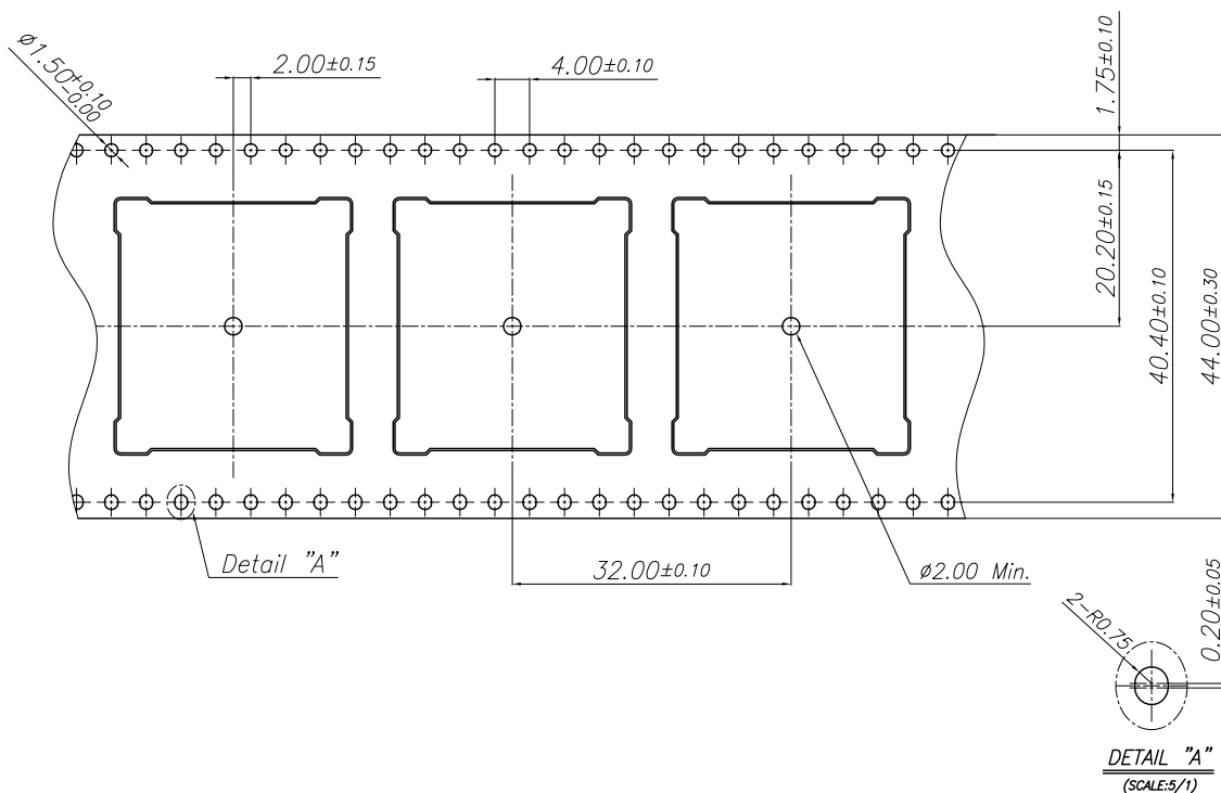
Figure 47: Carrier tape
