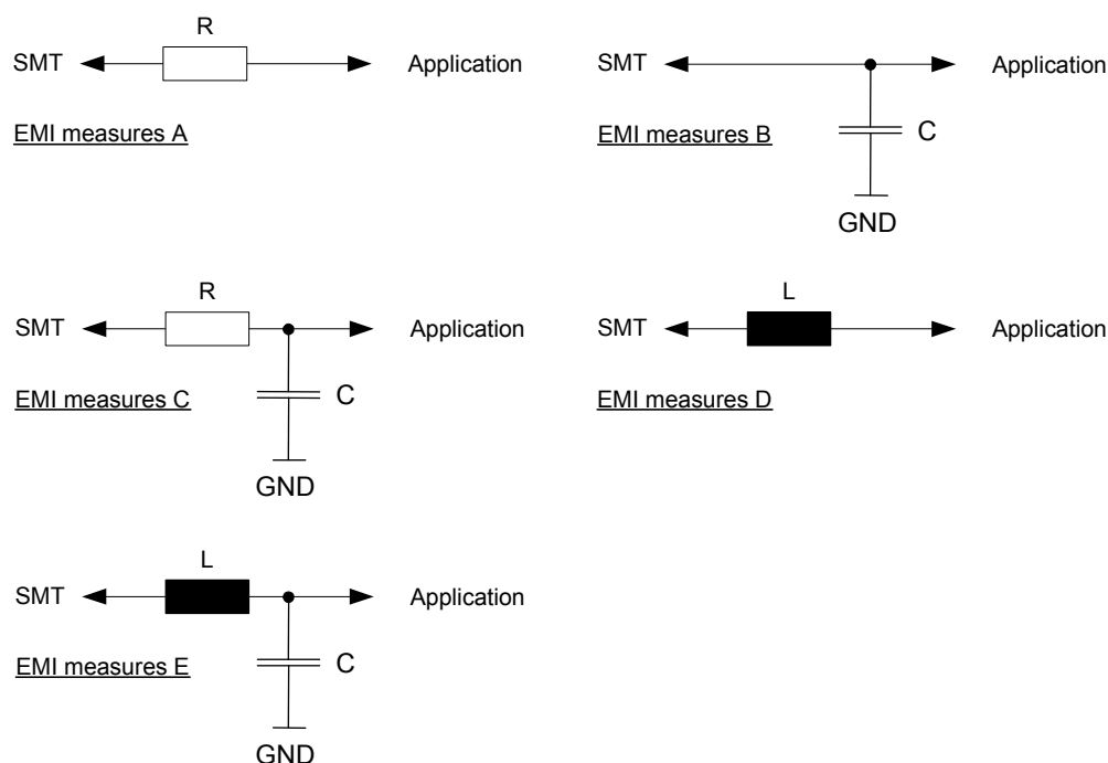
Figure 40: EMI circuits
