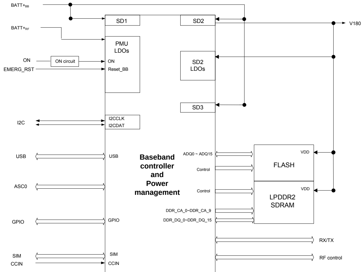
Figure 2: ELS61-AUS block diagram
