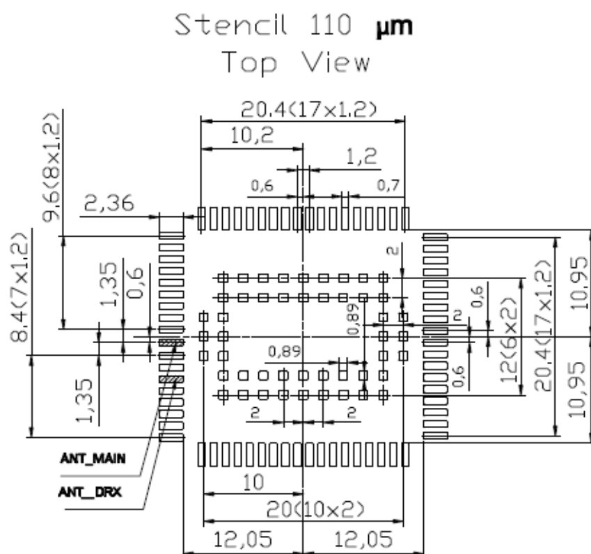
Figure 44: Recommended design for 110 \mu\text{m} micron thick stencil (top view)
