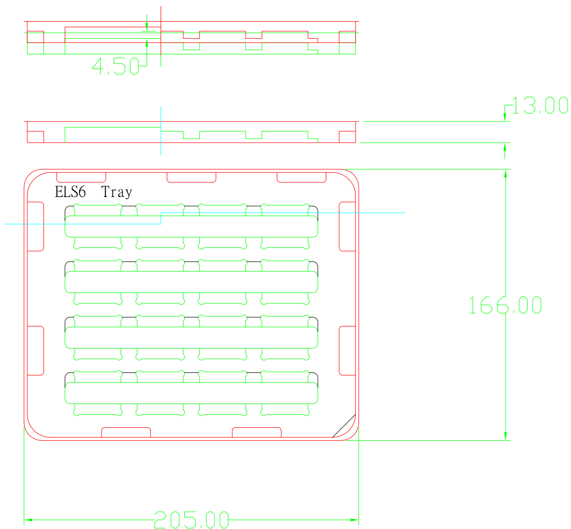
Figure 53: Tray dimensions
