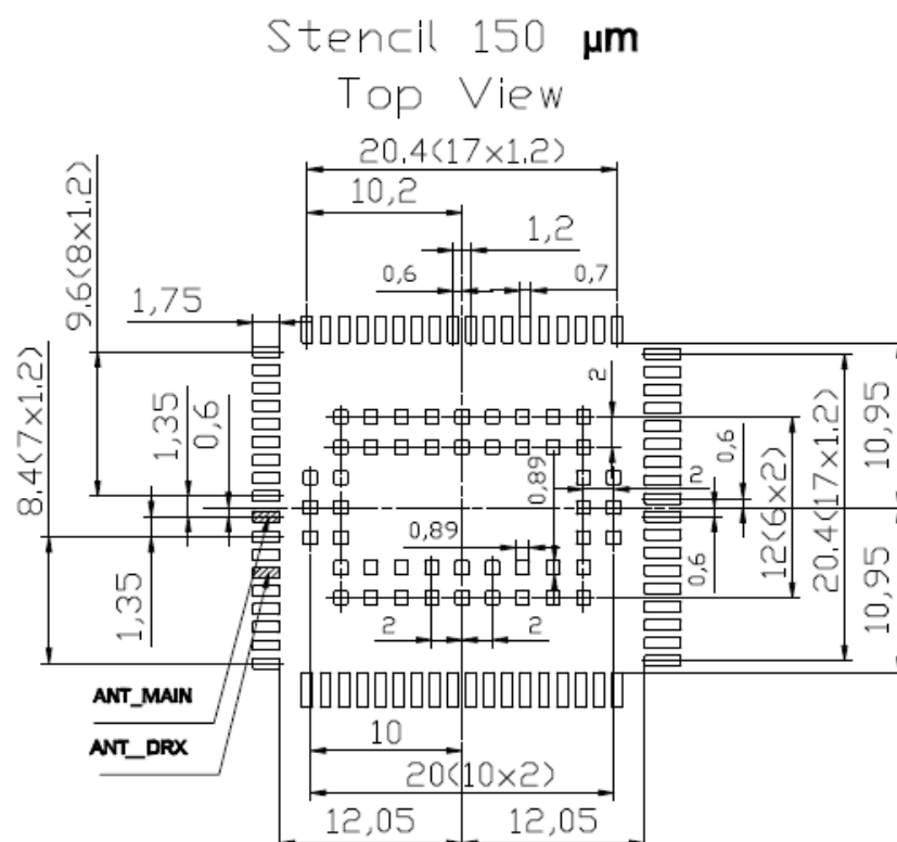
Figure 45: Recommended design for 150 \mu\text{m} micron thick stencil (top view)
