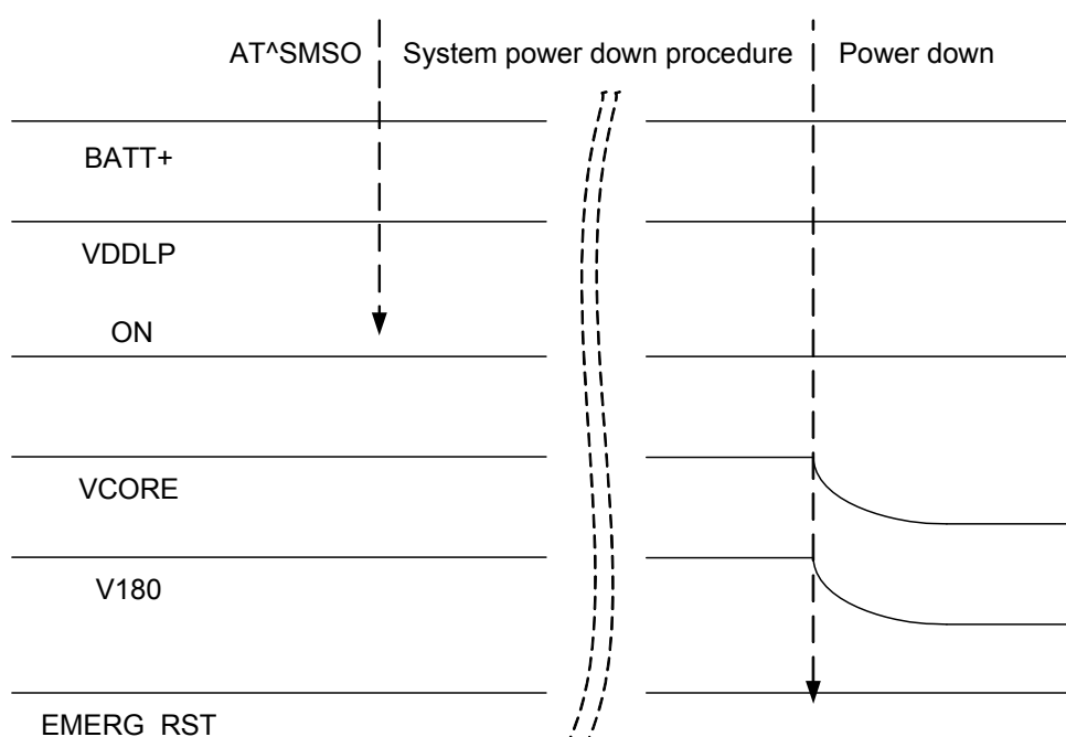
Figure 34: Switch off behavior
