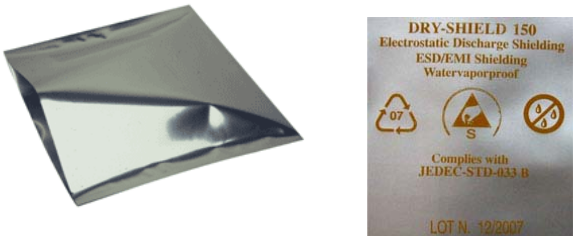
Figure 50: Moisture barrier bag (MBB) with imprint
