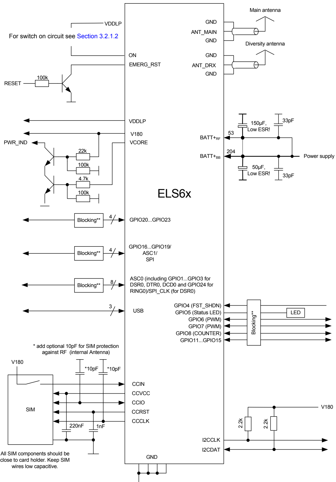
Figure 27: Schematic diagram of ELS61-AUS sample application
