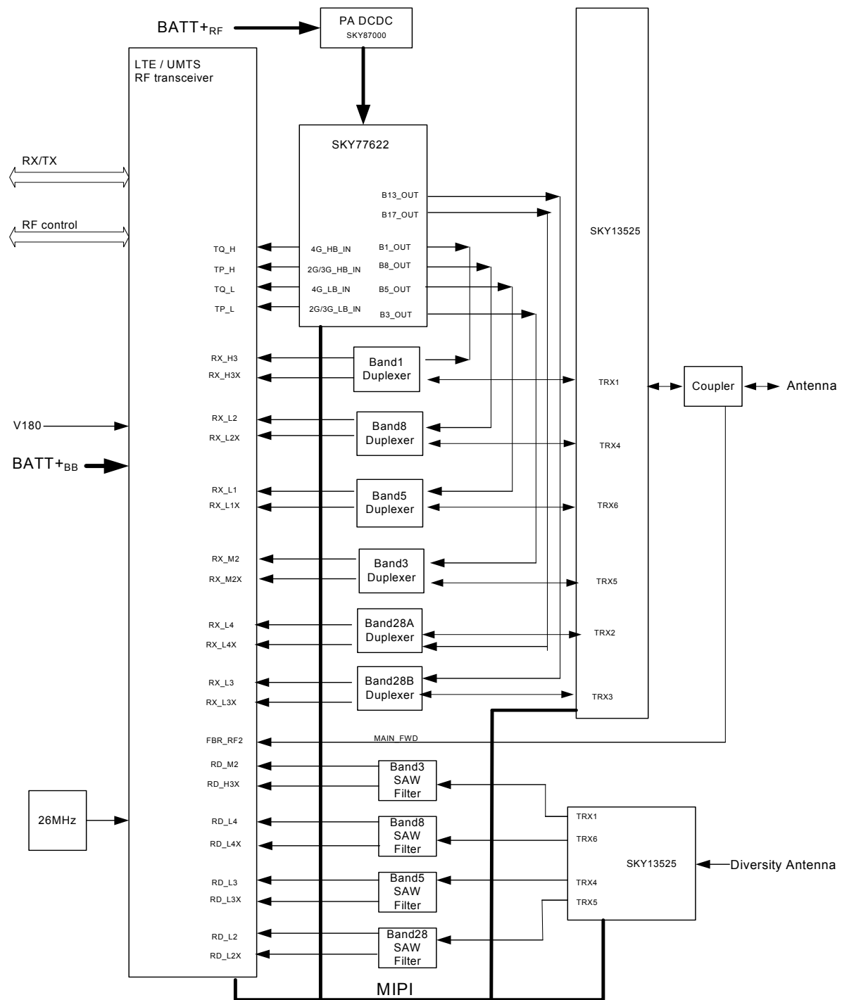
Figure 3: ELS61-AUS RF section block diagram
