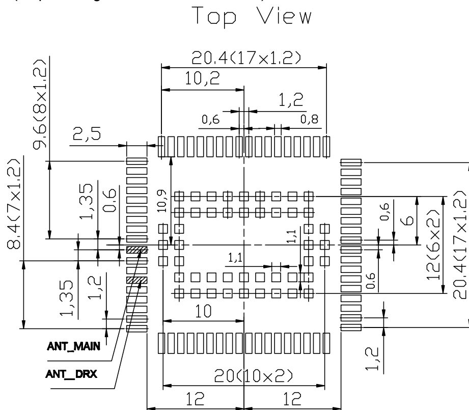
Figure 43: Land pattern (top view)
