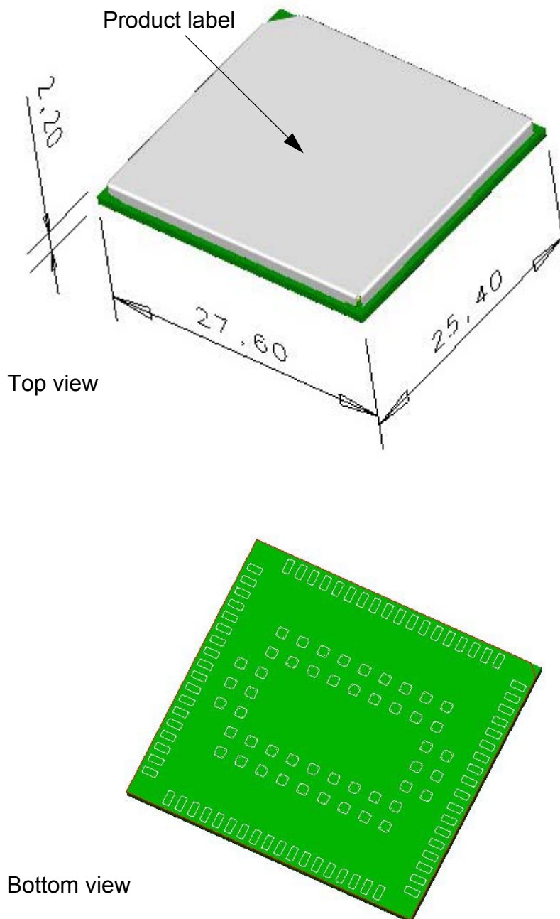
Figure 41: ELS61-AUS– top and bottom view
