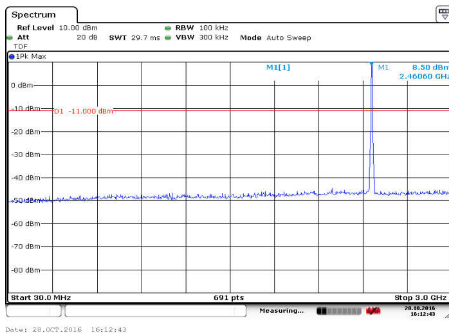
Fig.124 Conducted Spurious Emission (802.11b, Ch11, 30 MHz-3 GHz)
