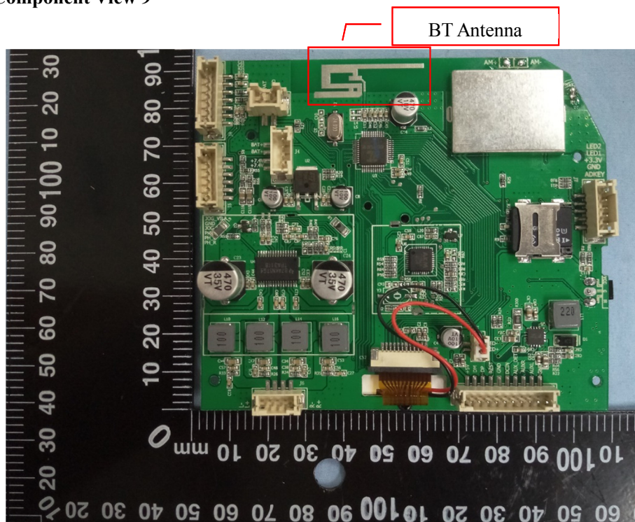
Solder Board-Component View 9
