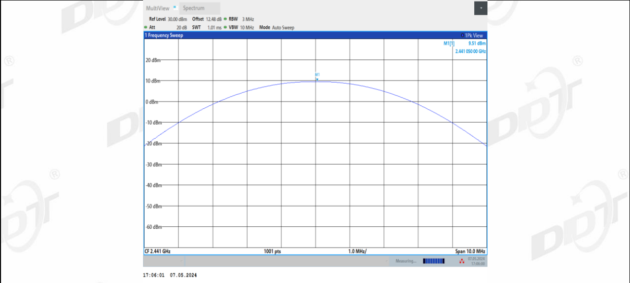
2DH5_Ant2_R_2441
