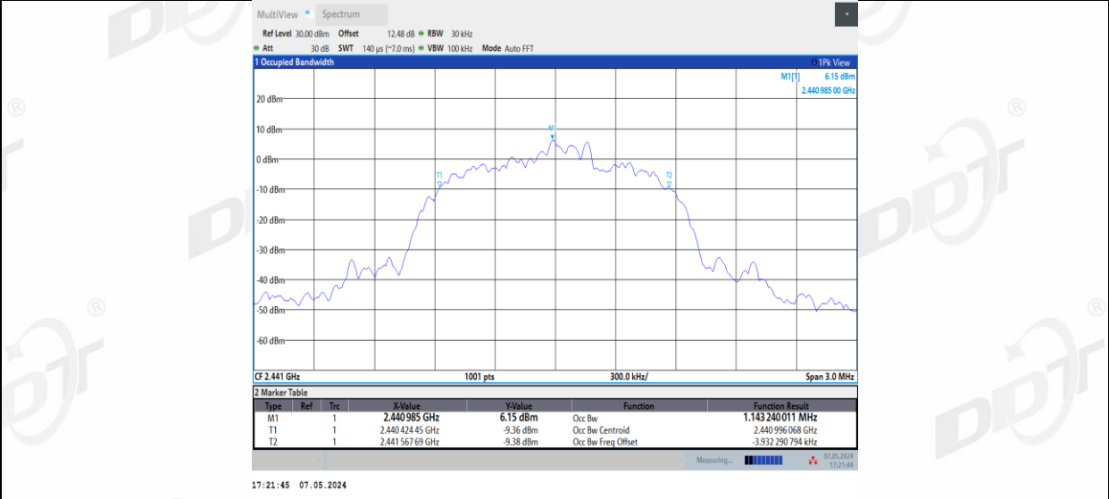
3DH5_Ant2_R_2441
