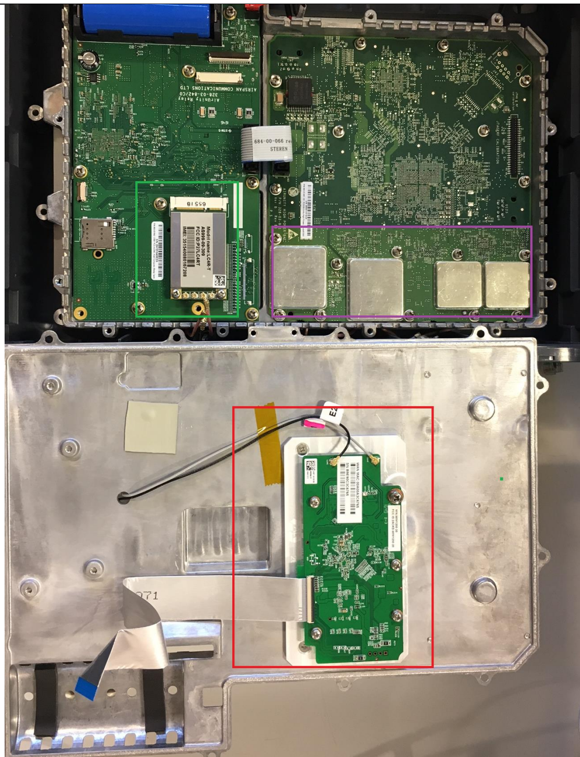
WiFi module mounted onto other side of metal plate
