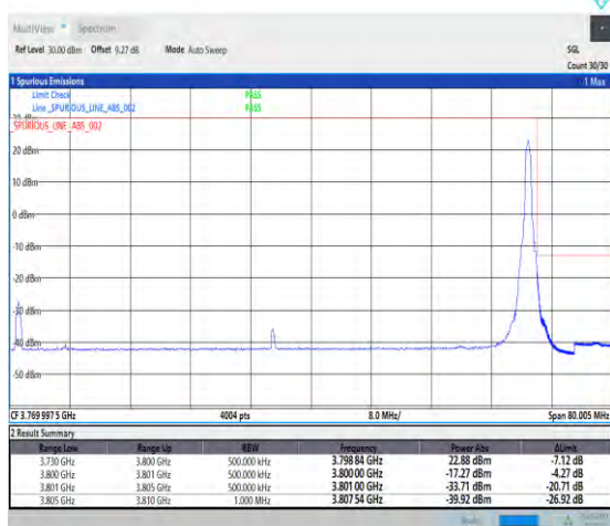
1-N78-3700-3800-PC1-30-70-H-5-CP-QPSK-Edge_1RB_Right-1@188-Ant0-1--PASS-see graph
