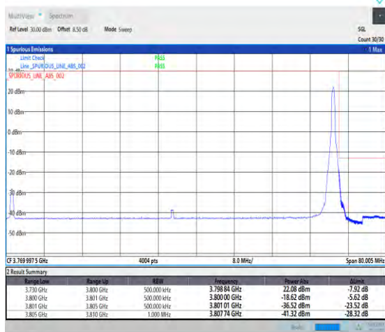
1-N78-3700-3800-PC1-30-70-H-2-DFT-PI2BPSK-Edge_1RB_Right-1@188-Ant0-1--PASS-see graph
