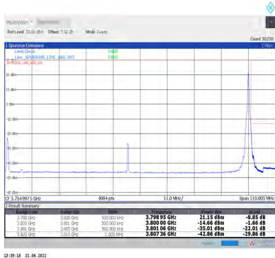
1-N78-3700-3800--30-100-H-5-CP-QPSK-Edge_1RB_Right-1@272-Ant0-PASS-see graph
