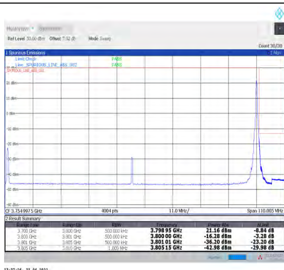
1-N78-3700-3800--30-100-H-2-DFT-PI2BPSK-Edge_1 RB_Right-1@272-Ant0-PASS-see graph
