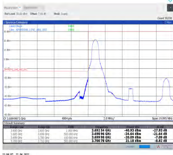
1-N78-3700-3800--30-10-L-1-DFT-PI2BPSK-Edge_1R B_Left-1@0-Ant0-PASS-see graph
