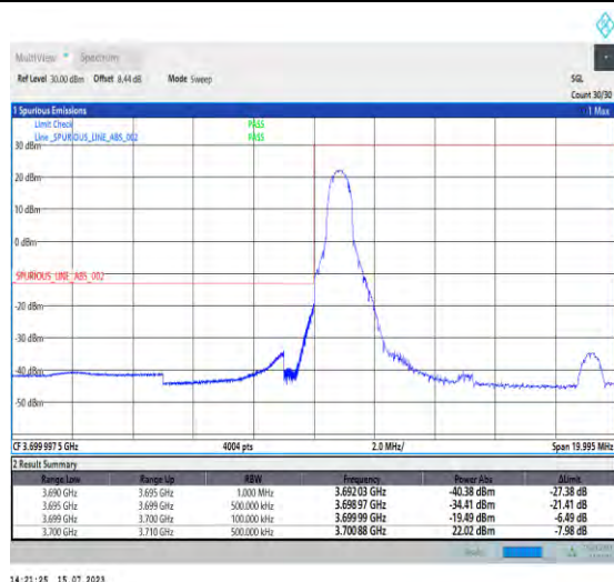
1-N78-3700-3800-PC1-30-10-L-1-DFT-PI2BPSK-Edge_1RB_Left-1@0-Ant0-1--PASS-see graph
