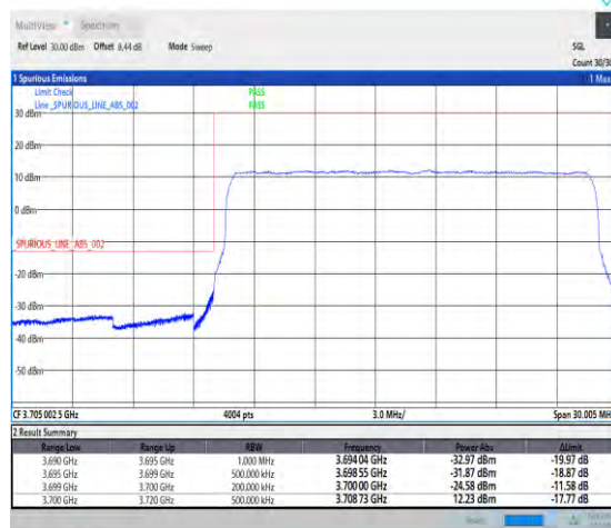
1-N78-3700-3800-PC1-30-20-L-3-DFT-PI2BPSK-Outer_Full-50@0-Ant0-1--PASS-see graph
