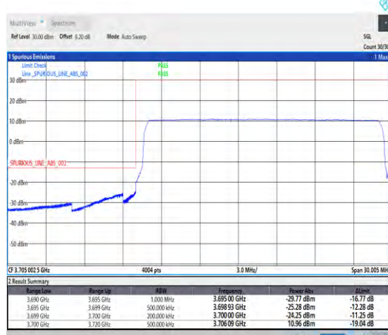
1-N78-3700-3800-PC1-30-20-L-6-CP-QPSK-Outer_Full-51@0-Ant0-1--PASS-see graph
