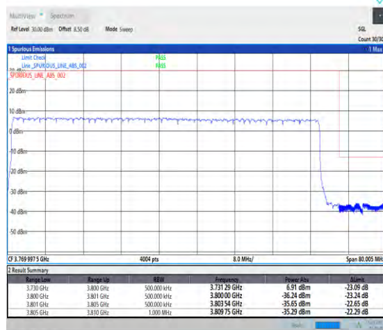
1-N78-3700-3800-PC1-30-70-H-3-DFT-PI2BPSK-Outer_Full-180@0-Ant0-1--PASS-see graph
