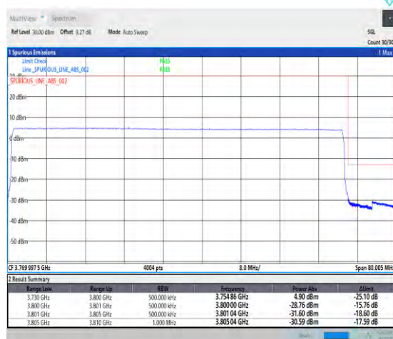
1-N78-3700-3800-PC1-30-70-H-6-CP-QPSK-Outer_Full-189@0-Ant0-1--PASS-see graph
