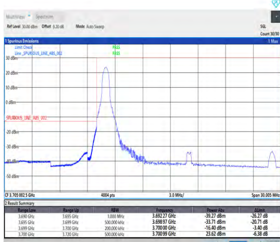
1-N78-3700-3800-PC1-30-20-L-4-CP-QPSK-Edge_1_RB_Left-1@0-Ant0-1--PASS-see graph
