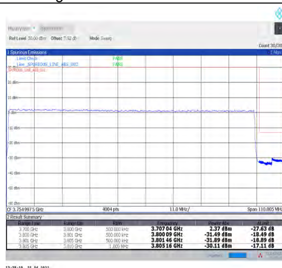
1-N78-3700-3800--30-100-H-3-DFT-PI2BPSK-Out er_Full-270@0-Ant0-PASS-see graph
