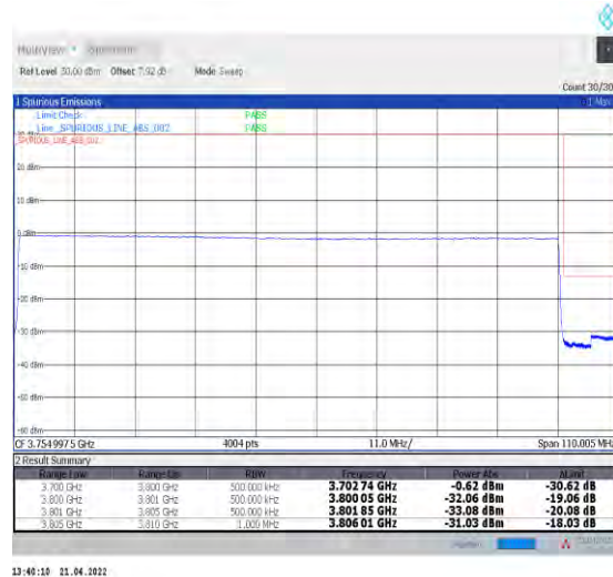
1-N78-3700-3800--30-100-H-6-CP-QPSK-Outer_Full-273@0-Ant0-PASS-see graph
