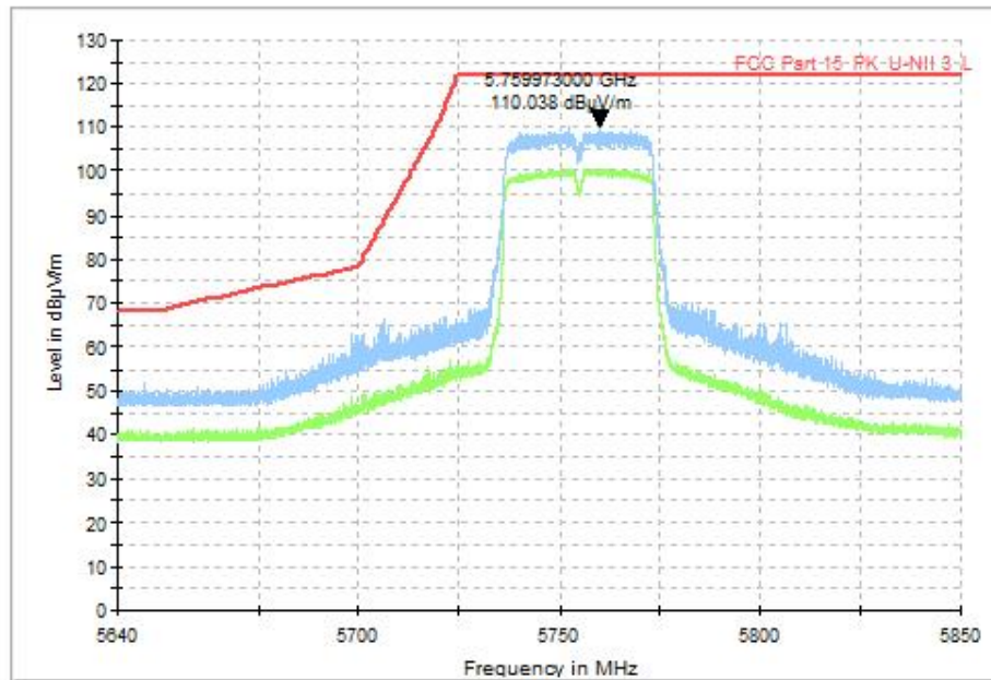
Fig. 45 Band Edges (802.11n-HT40, CH151 5755MHz), MIMO
