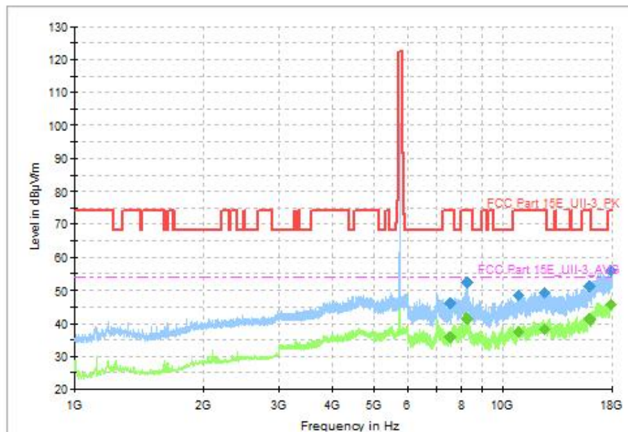
Fig. 77 Transmitter Spurious Emission (802.11ax-HE20, CH149 5745MHz, 1GHz-18GHz), MIMO
