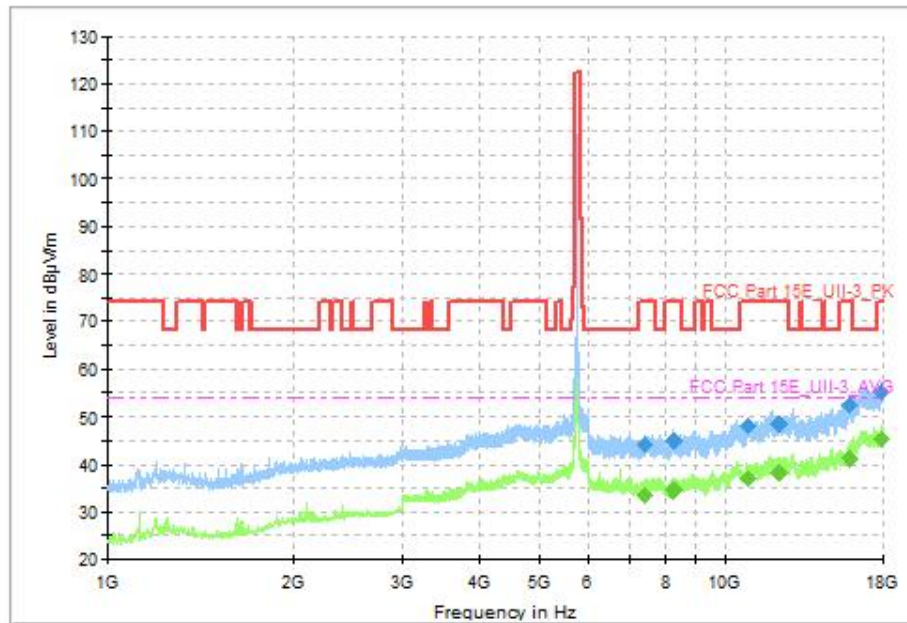
Fig. 61 Transmitter Spurious Emission (802.11n-HT40, CH151 5755MHz, 1GHz-18GHz)
