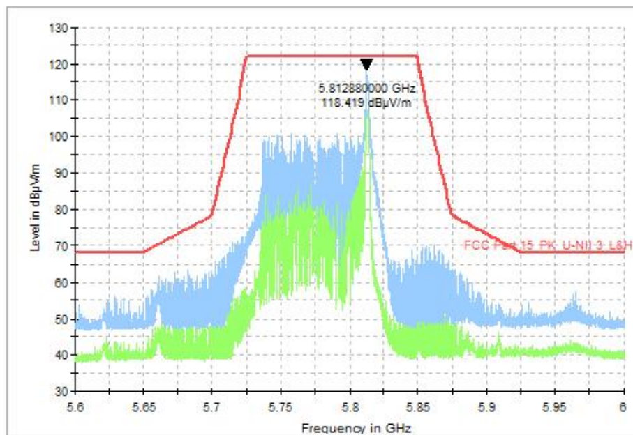
Fig. 40 Band Edges (802.11ax-HE80(RU26), CH155 5775MHz)
