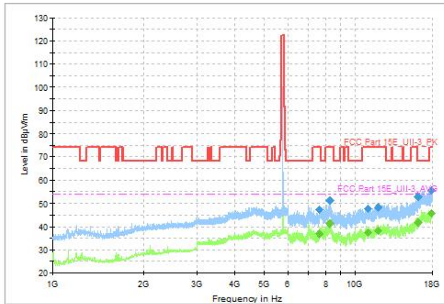
Fig. 53 Transmitter Spurious Emission (802.11ax-HE20, CH157 5785MHz, 1GHz-18GHz)
