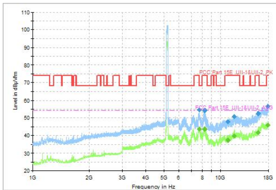
Fig. 84 Transmitter Spurious Emission (802.11ac-VHT80, CH42 5210MHz, 1GHz-18GHz), MIMO
