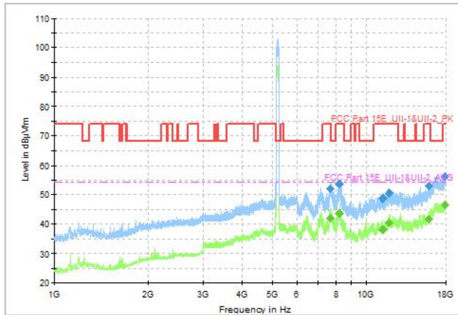
Fig. 67 Transmitter Spurious Emission (802.11ac-VHT80, CH42 5210MHz, 1GHz-18GHz)
