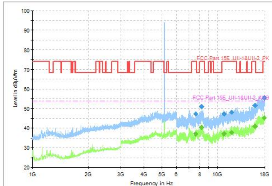
Fig. 49 Transmitter Spurious Emission (802.11ax-HE20, CH36 5180MHz, 1GHz-18GHz)
