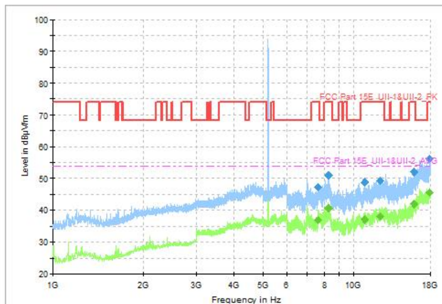
Fig. 50 Transmitter Spurious Emission (802.11ax-HE20, CH40 5200MHz, 1GHz-18GHz)
