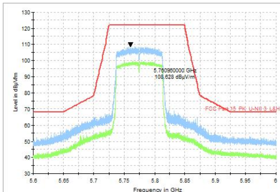
Fig. 48 Band Edges (802.11ac-VHT80, CH155 5775MHz), MIMO
