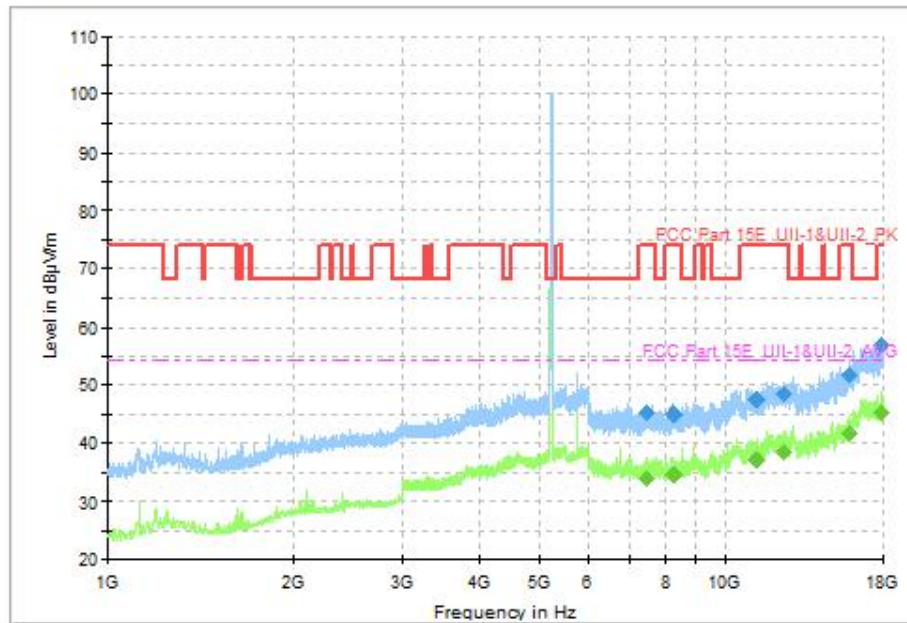
Fig. 81 Transmitter Spurious Emission (802.11n-HT40, CH46 5230MHz, 1GHz-18GHz), MIMO
