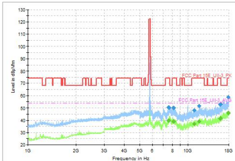
Fig. 70 Transmitter Spurious Emission (802.11ax-HE80(RU26), CH155 5775MHz, 1GHz-18GHz)
