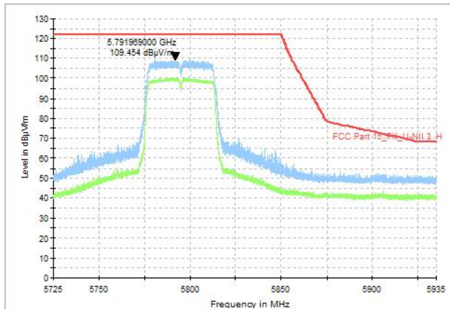
Fig. 46 Band Edges (802.11n-HT40, CH159 5795MHz), MIMO
