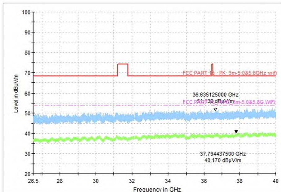
Fig. 88 Transmitter Spurious Emission (All channel, 26.5GHz~40GHz), MIMO
