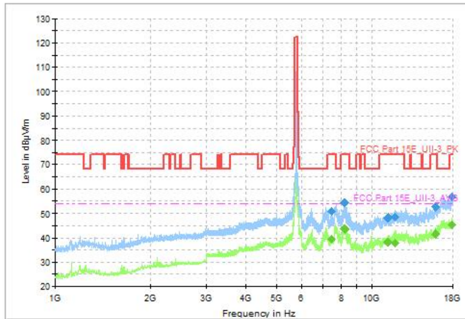
Fig. 85 Transmitter Spurious Emission (802.11ac-VHT80, CH155 5775MHz, 1GHz-18GHz), MIMO
