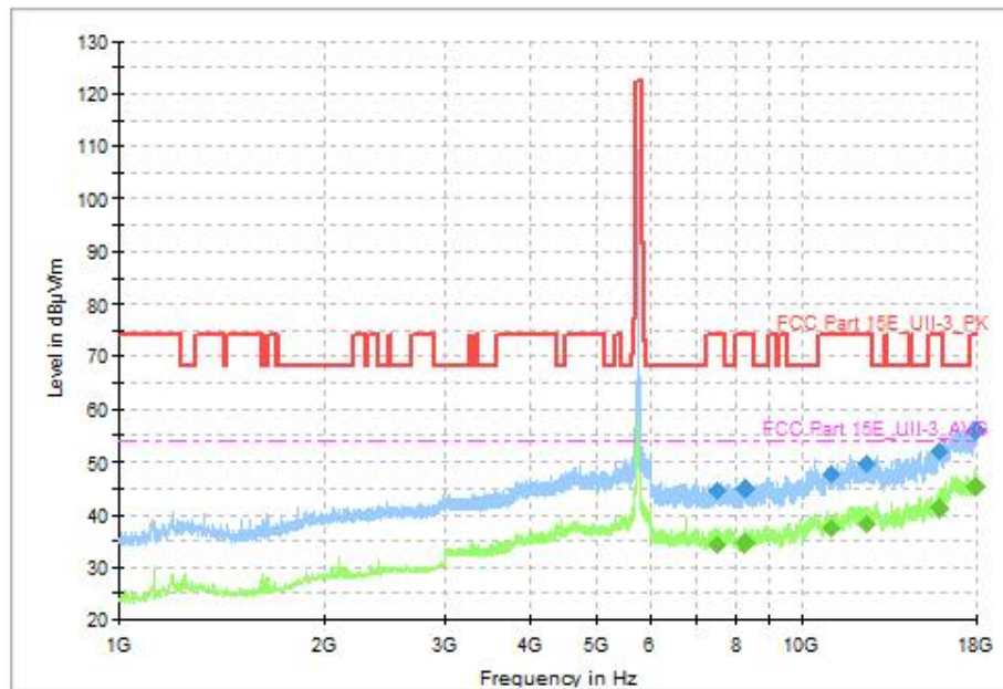
Fig. 82 Transmitter Spurious Emission (802.11n-HT40, CH151 5755MHz, 1GHz-18GHz), MIMO
