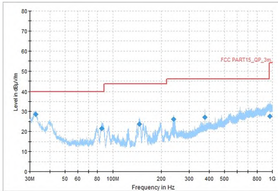
Fig. 71 Transmitter Spurious Emission (All channel, 30MHz~1GHz)
