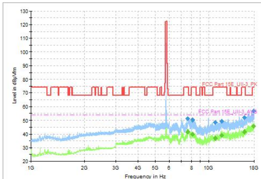
Fig. 65 Transmitter Spurious Emission (802.11ax-HE40(RU26), CH151 5755MHz, 1GHz-18GHz)
