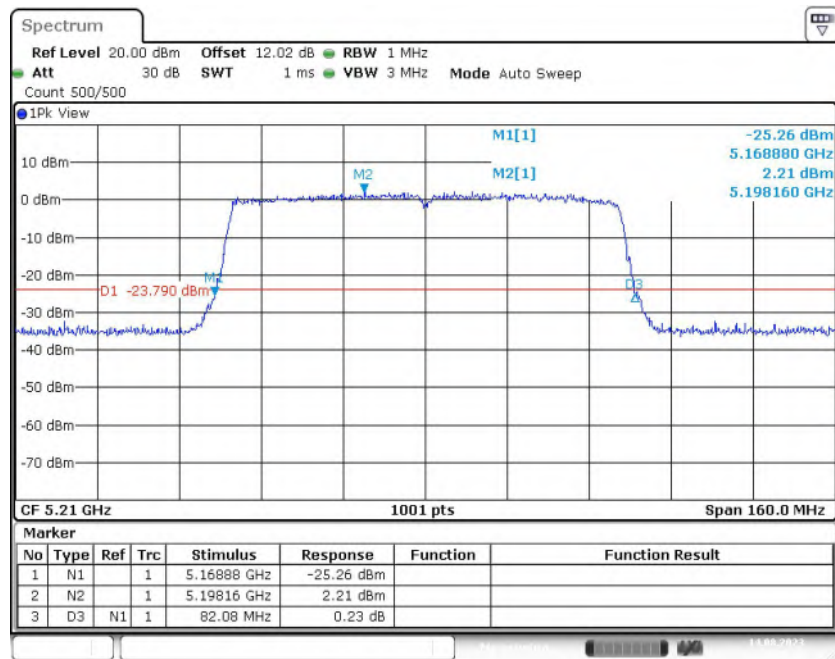
Fig. 6 Occupied 26dB Bandwidth (802.11ac-VHT80, 5210MHz)
