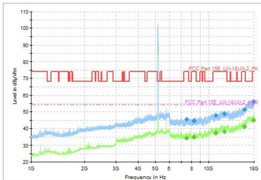
Fig. 80 Transmitter Spurious Emission (802.11n-HT40, CH38 5190MHz, 1GHz-18GHz), MIMO
