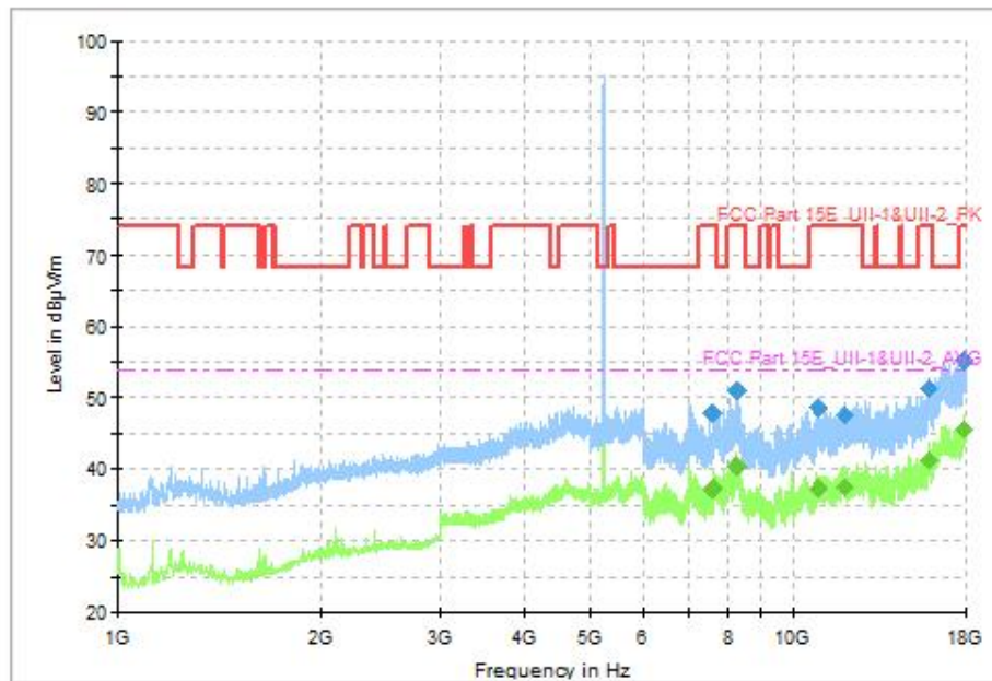
Fig. 76 Transmitter Spurious Emission (802.11ax-HE20, CH48 5240MHz, 1GHz-18GHz), MIMO
