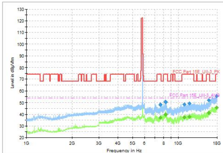
Fig. 54 Transmitter Spurious Emission (802.11ax-HE20, CH165 5825MHz, 1GHz-18GHz)
