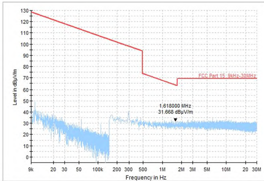
Fig. 93 Radiated Spurious Emission (All Channel, 9 kHz ~30 MHz)
