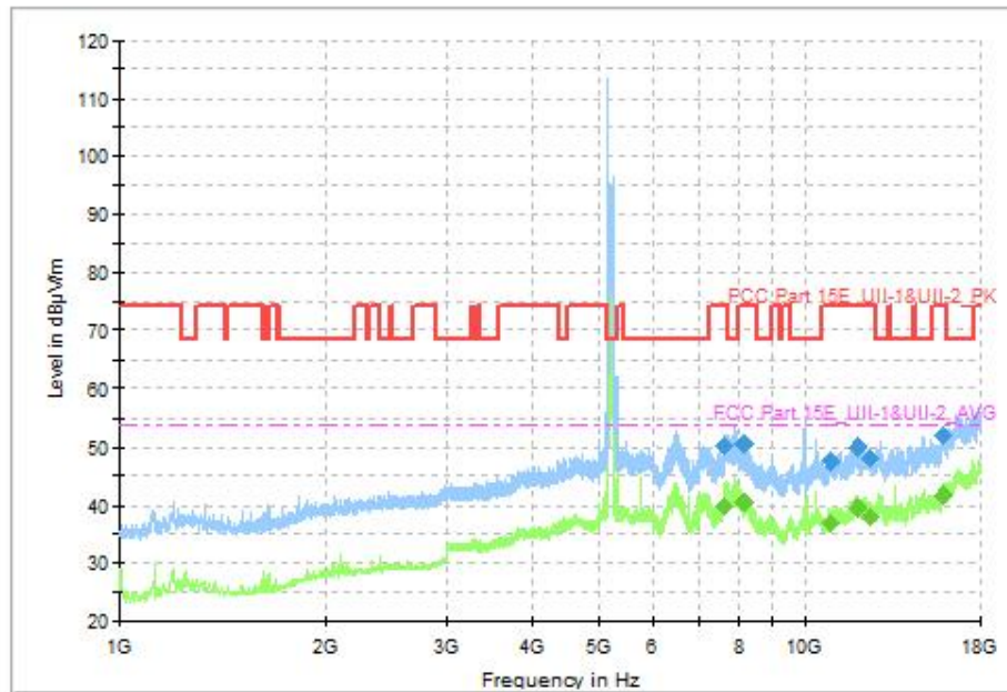
Fig. 69 Transmitter Spurious Emission (802.11ax-HE80(RU26), CH42 5210MHz, 1GHz-18GHz)
