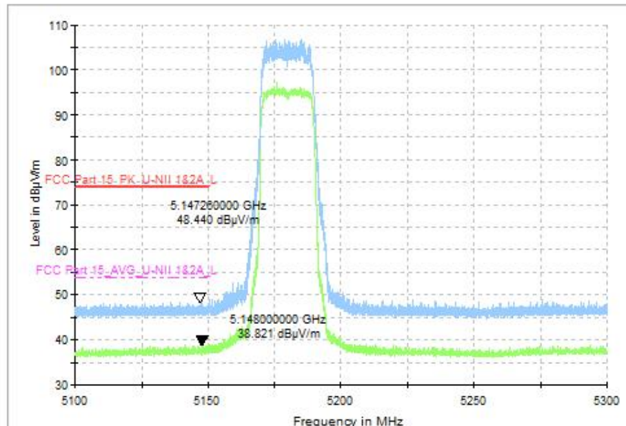
Fig. 25 Band Edges (802.11ax-HE20, CH36 5180MHz)
