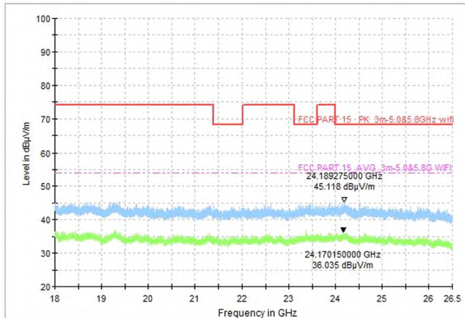
Fig. 91 Transmitter Spurious Emission (DH5 & 802.11ac-VHT80, CH0 2402MHz & CH42 5210MHz, 18GHz~26.5GHz)
