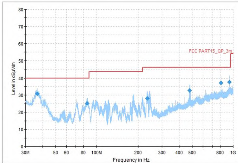
Fig. 89 Transmitter Spurious Emission (DH5 & 802.11ac-VHT80, CH0 2402MHz & CH42 5210MHz, 30MHz~1GHz)
