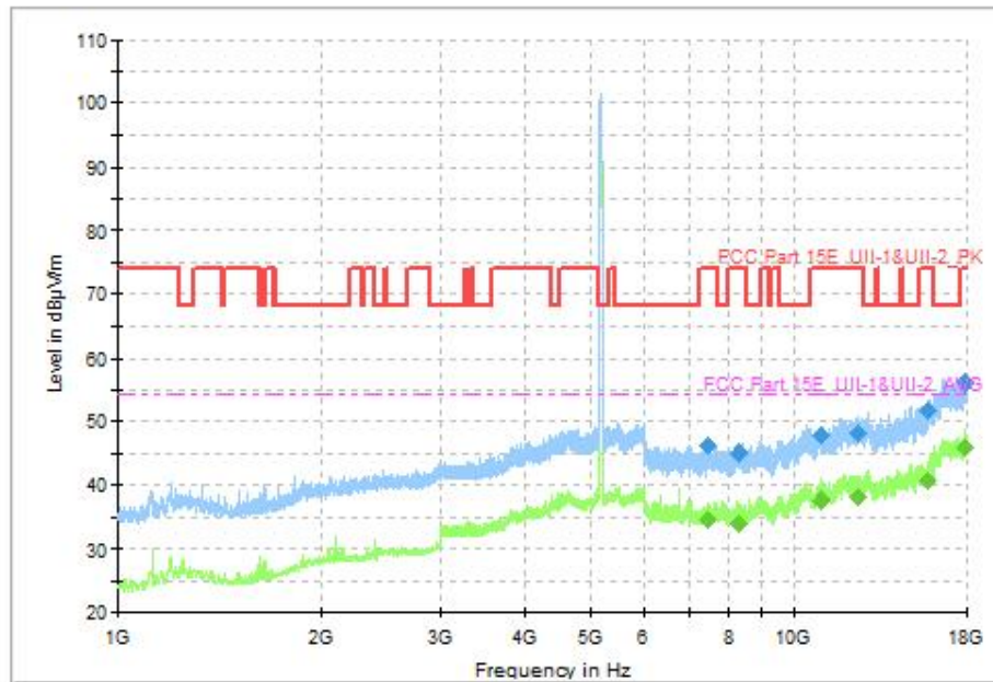
Fig. 59 Transmitter Spurious Emission (802.11n-HT40, CH38 5190MHz, 1GHz-18GHz)
