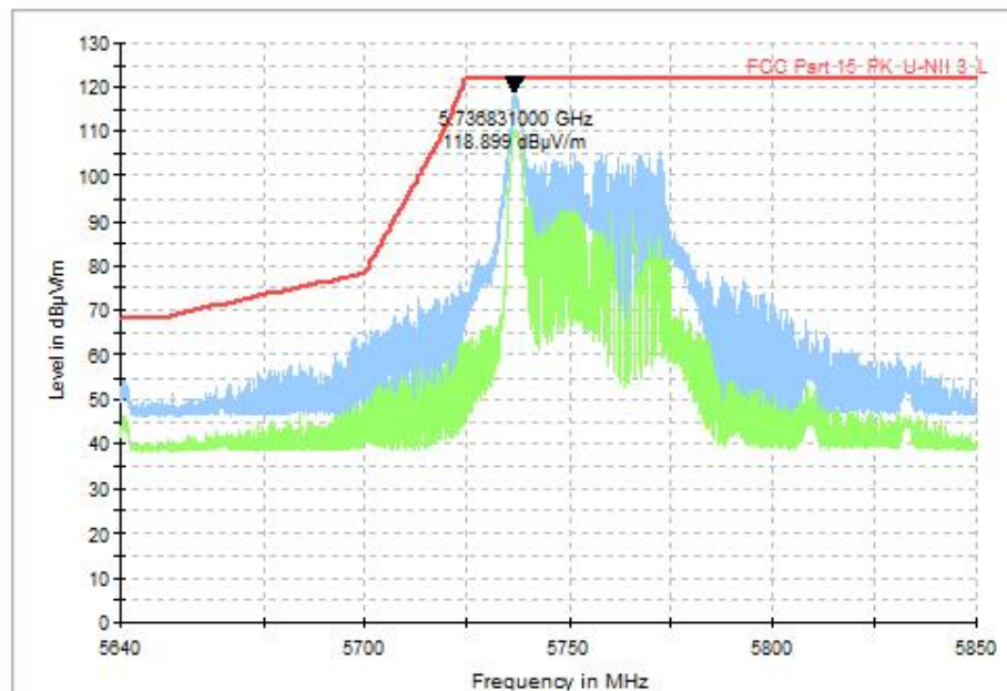
Fig. 35 Band Edges (802.11ax-HE40(RU26), CH151 5755MHz)
