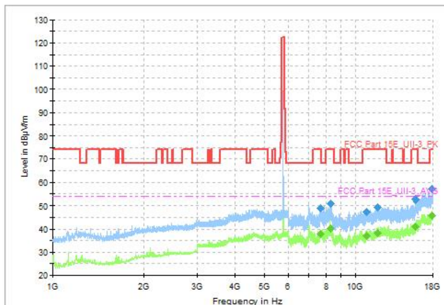
Fig. 78 Transmitter Spurious Emission (802.11ax-HE20, CH157 5785MHz, 1GHz-18GHz), MIMO
