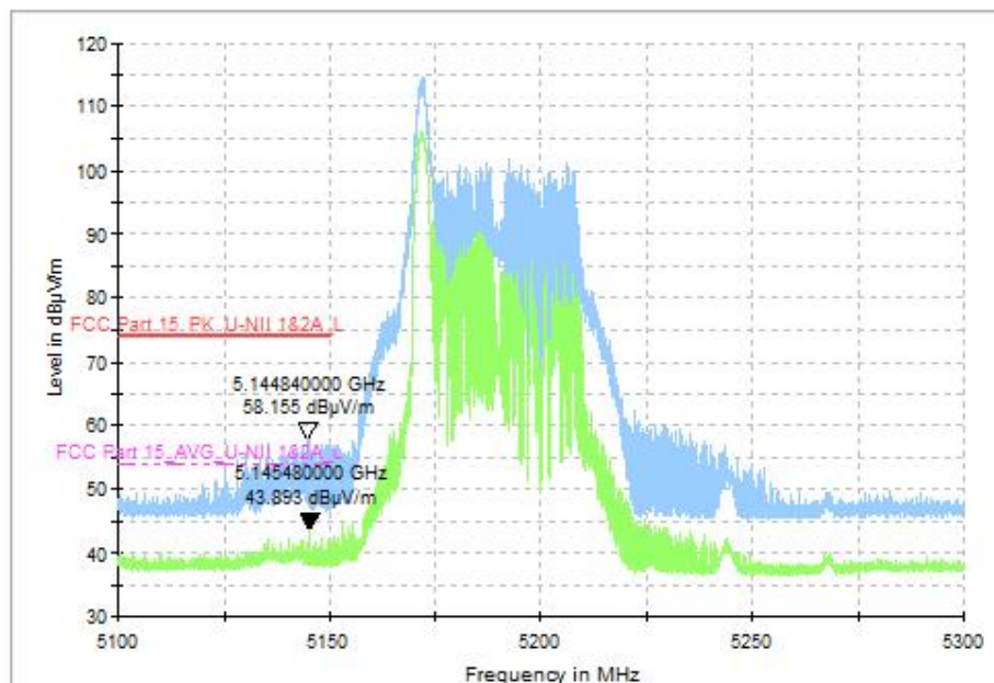
Fig. 34 Band Edges (802.11ax-HE40(RU26), CH38 5190MHz)
