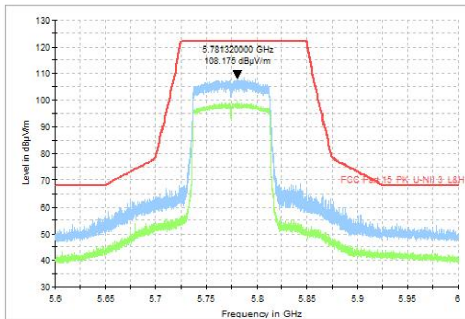
Fig. 38 Band Edges (802.11ac-VHT80, CH155 5775MHz)
