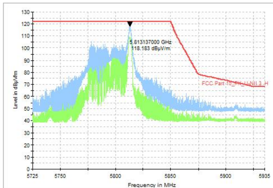
Fig. 36 Band Edges (802.11ax-HE40(RU26), CH159 5795MHz)
