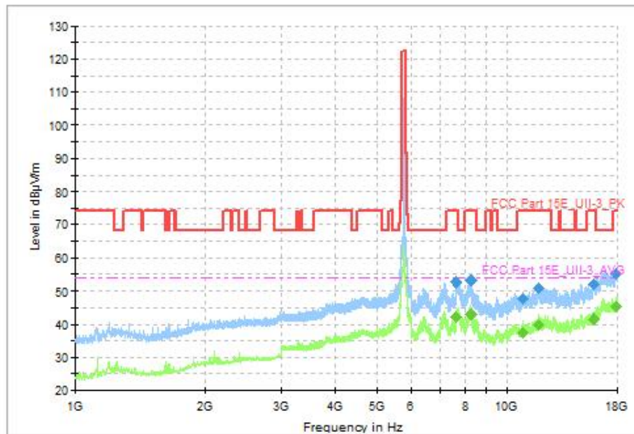
Fig. 68 Transmitter Spurious Emission (802.11ac-VHT80, CH155 5775MHz, 1GHz-18GHz)
