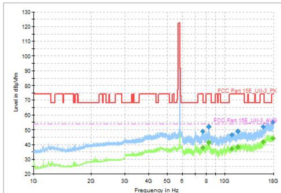
Fig. 79 Transmitter Spurious Emission (802.11ax-HE20, CH165 5825MHz, 1GHz-18GHz), MIMO
