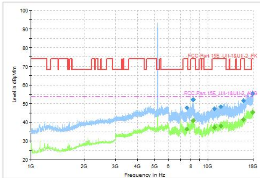
Fig. 75 Transmitter Spurious Emission (802.11ax-HE20, CH40 5200MHz, 1GHz-18GHz), MIMO
