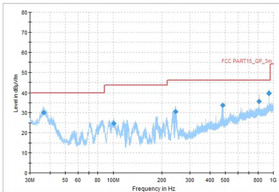
Fig. 86 Transmitter Spurious Emission (All channel, 30MHz~1GHz), MIMO
