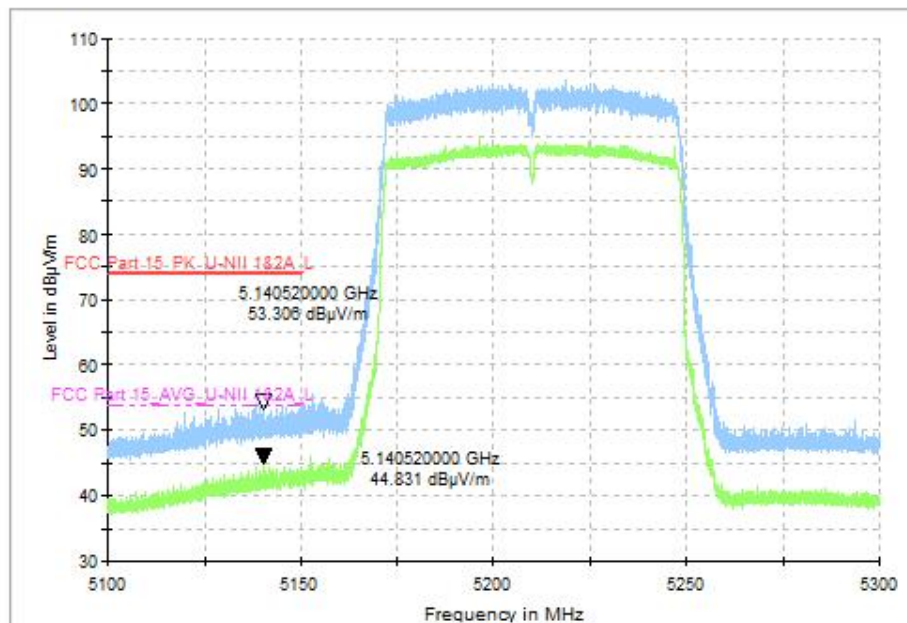
Fig. 47 Band Edges (802.11ac-VHT80, CH42 5210MHz), MIMO
