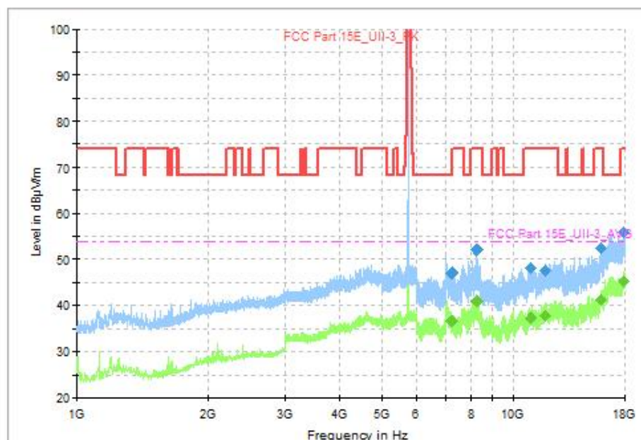
Fig. 52 Transmitter Spurious Emission (802.11ax-HE20, CH149 5745MHz, 1GHz-18GHz)
