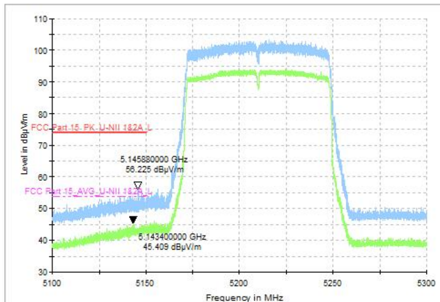
Fig. 37 Band Edges (802.11ac-VHT80, CH42 5210MHz)
