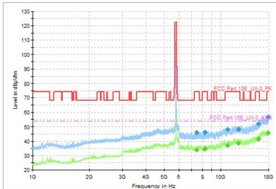
Fig. 62 Transmitter Spurious Emission (802.11n-HT40, CH159 5795MHz, 1GHz-18GHz)
