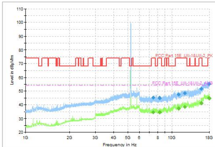
Fig. 60 Transmitter Spurious Emission (802.11n-HT40, CH46 5230MHz, 1GHz-18GHz)
