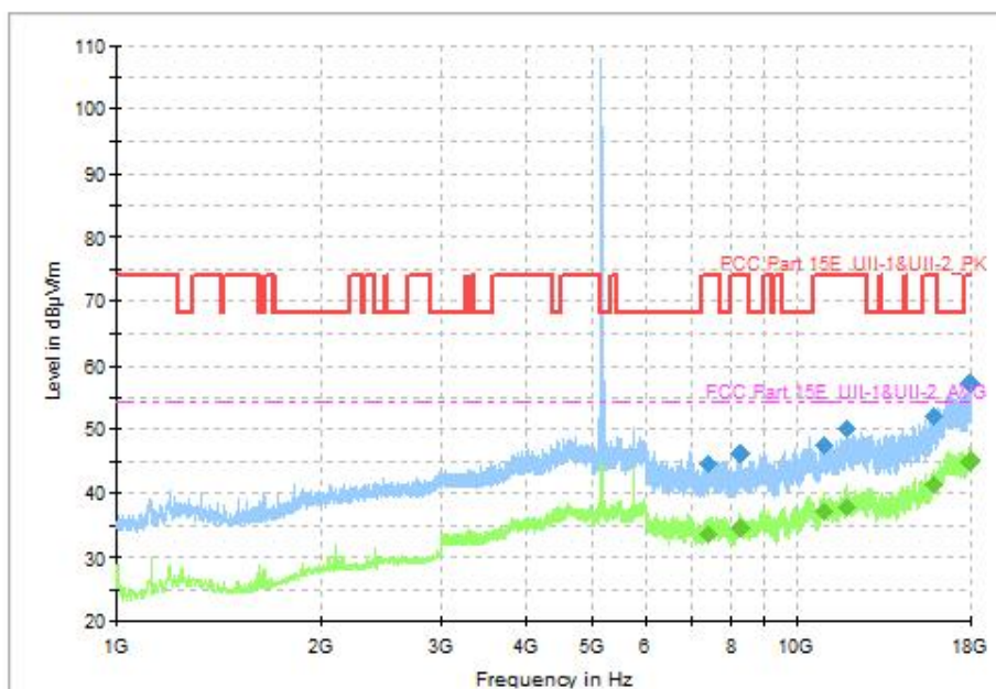
Fig. 55 Transmitter Spurious Emission (802.11ax-HE20(RU26), CH36 5180MHz, 1GHz-18GHz)
