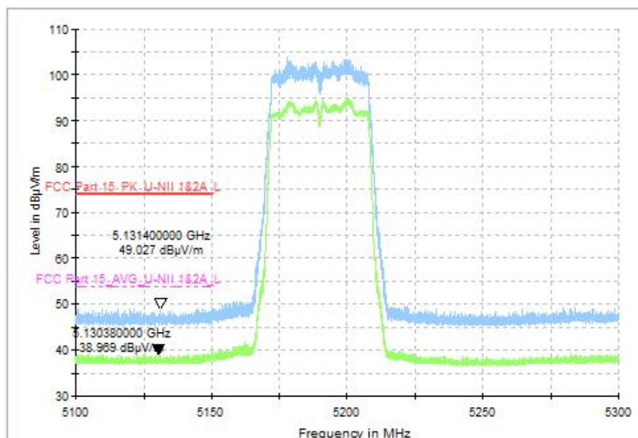
Fig. 44 Band Edges (802.11n-HT40, CH38 5190MHz), MIMO
