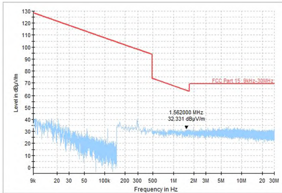
Fig. 95 Radiated Spurious Emission (DH5 & 802.11ac-VHT80, CH0 2402MHz & CH42 5210MHz, 9KHz~30MHz)
