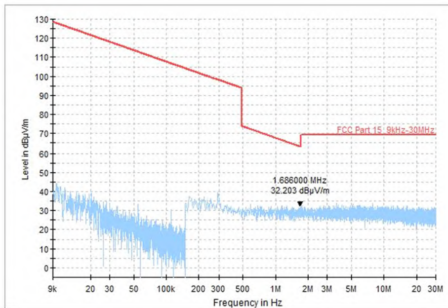
Fig. 94 Radiated Spurious Emission (All Channel, 9 kHz ~30 MHz), MIMO
