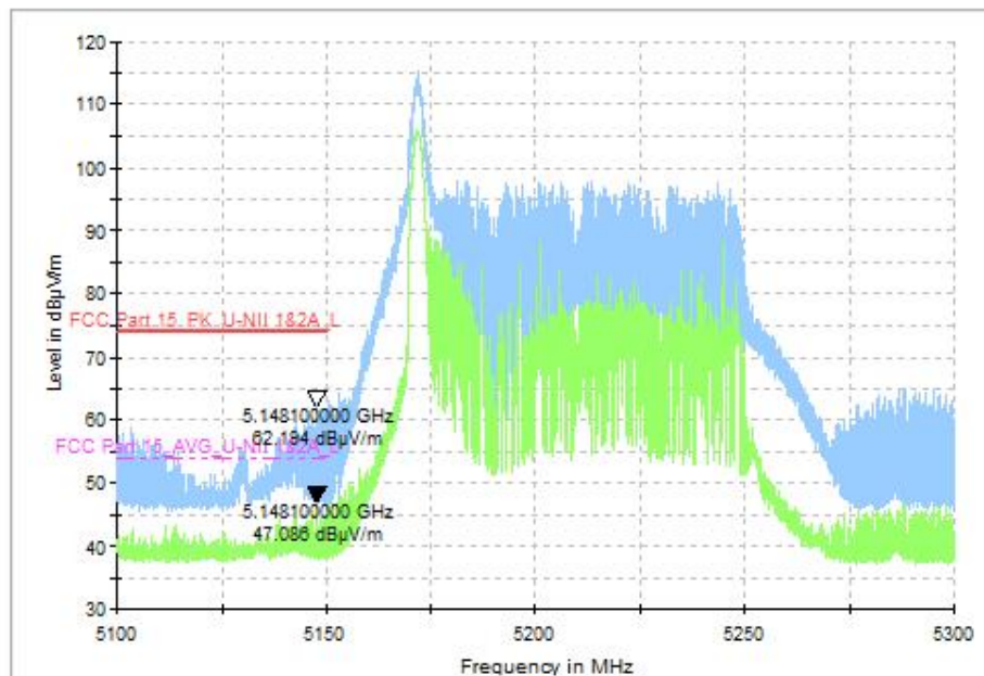
Fig. 39 Band Edges (802.11ax-HE80(RU26), CH42 5210MHz)
