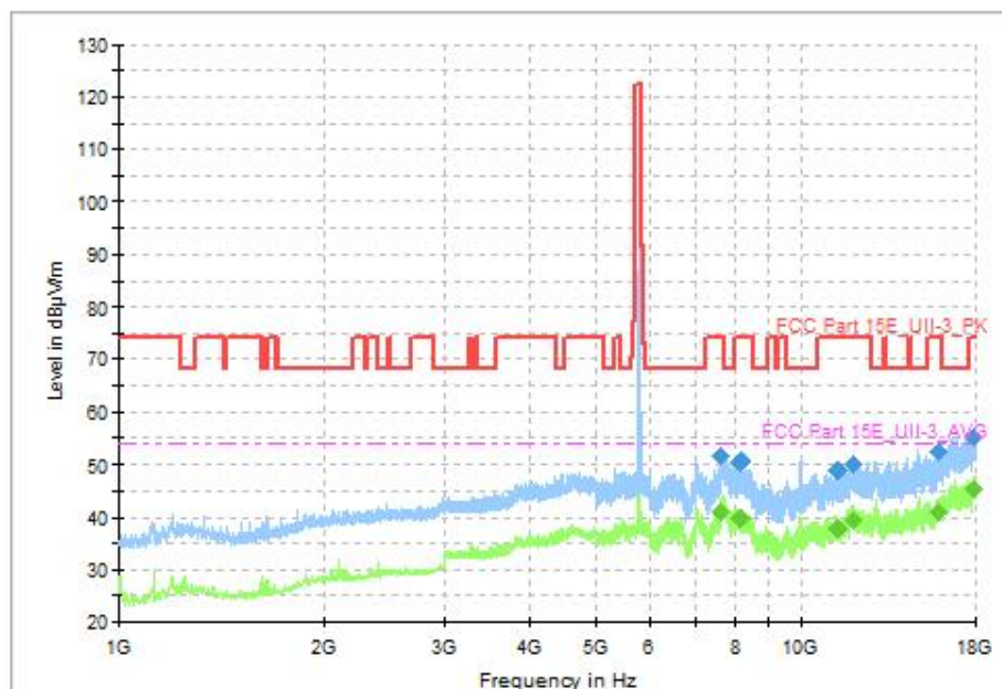
Fig. 66 Transmitter Spurious Emission (802.11ax-HE40(RU26), CH159 5795MHz, 1GHz-18GHz)
