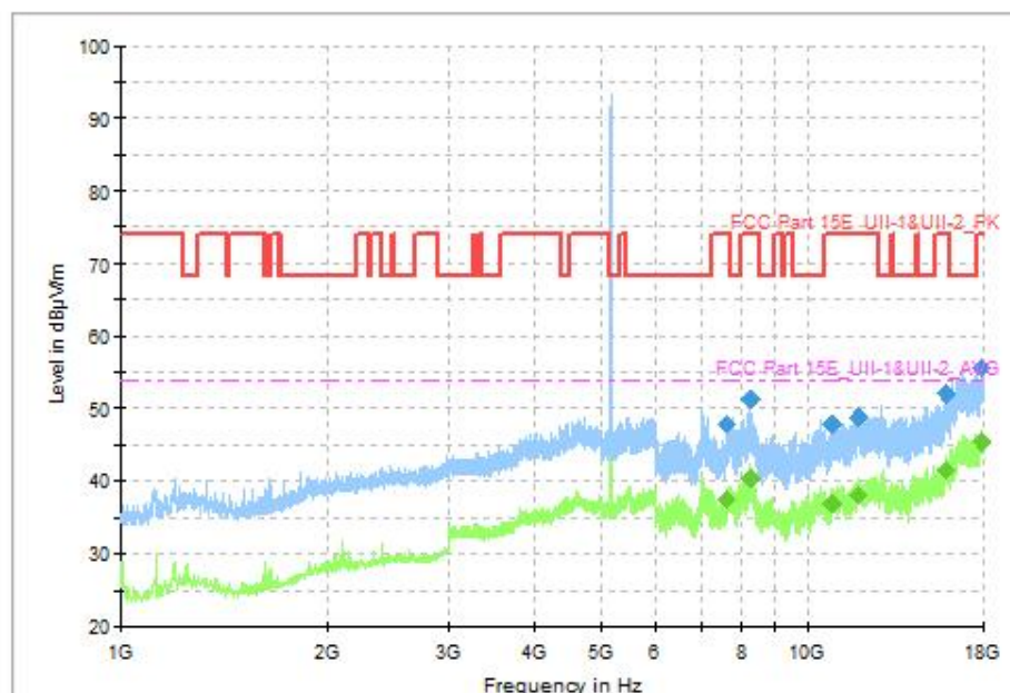
Fig. 74 Transmitter Spurious Emission (802.11ax-HE20, CH36 5180MHz, 1GHz-18GHz), MIMO
