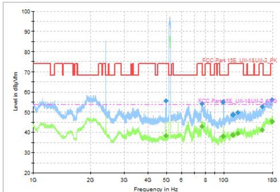
Fig. 90 Transmitter Spurious Emission (DH5 & 802.11ac-VHT80, CH0 2402MHz & CH42 5210MHz, 1GHz-18GHz)
