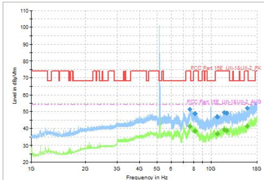
Fig. 63 Transmitter Spurious Emission (802.11ax-HE40(RU26), CH38 5190MHz, 1GHz-18GHz)
