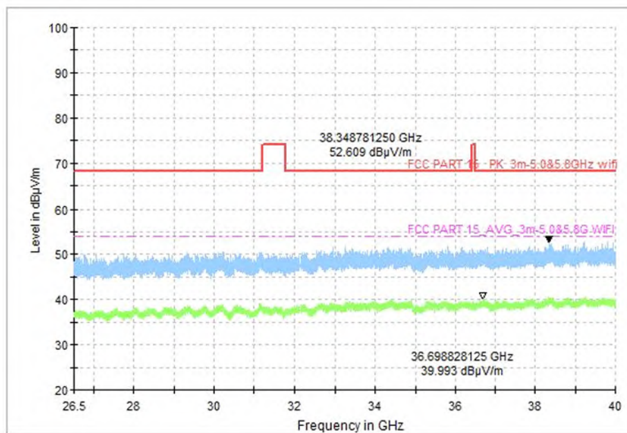
Fig. 92 Transmitter Spurious Emission (DH5 & 802.11ac-VHT80, CH0 2402MHz & CH42 5210MHz, 26.5GHz~40GHz)
