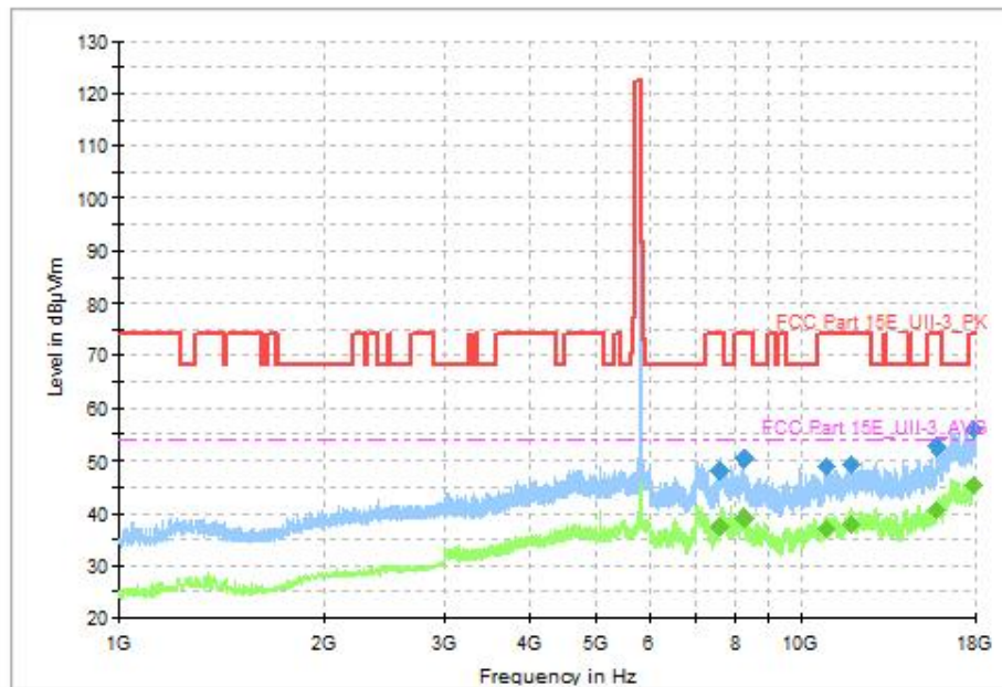
Fig. 58 Transmitter Spurious Emission (802.11ax-HE20(RU26), CH165 5825MHz, 1GHz-18GHz)
