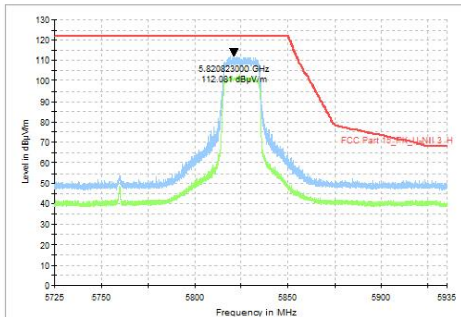
Fig. 43 Band Edges (802.11ax-HE20, CH165 5825MHz), MIMO
