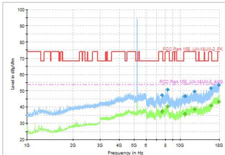
Fig. 51 Transmitter Spurious Emission (802.11ax-HE20, CH48 5240MHz, 1GHz-18GHz)
