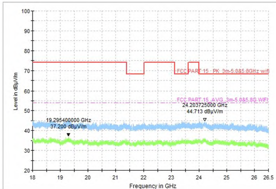
Fig. 87 Transmitter Spurious Emission (All channel, 18GHz~26.5GHz), MIMO
