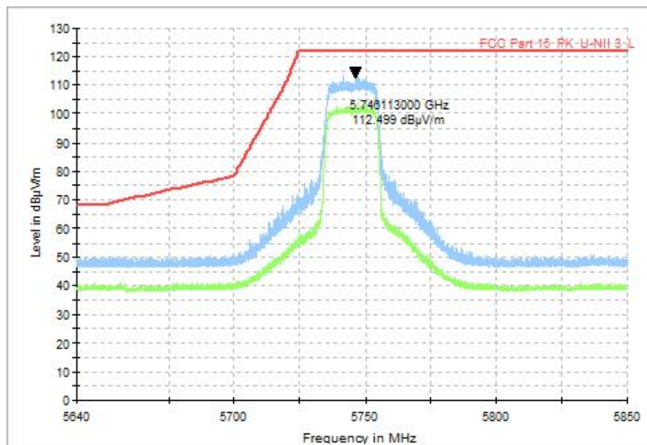
Fig. 42 Band Edges (802.11ax-HE20, CH149 5745MHz), MIMO
