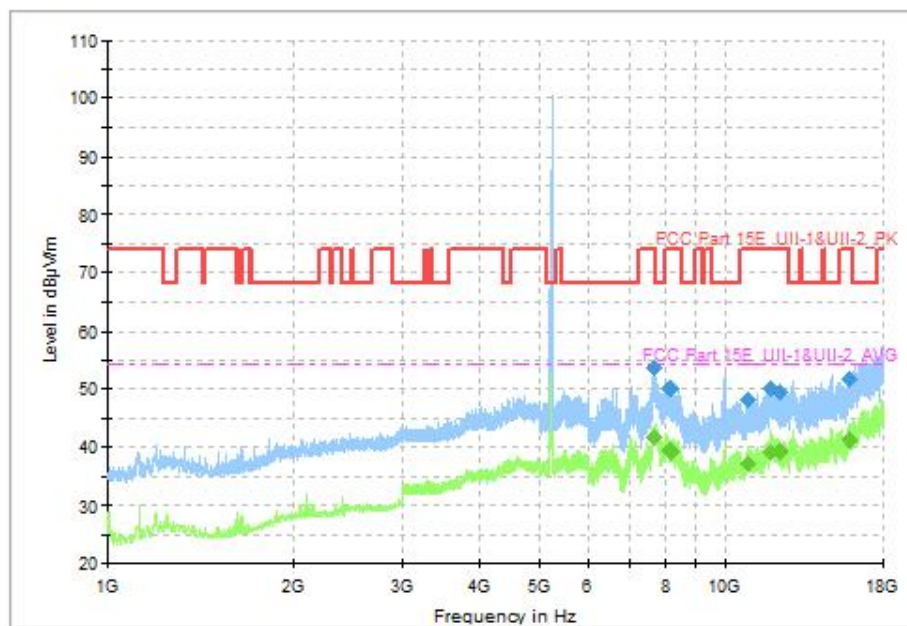
Fig. 64 Transmitter Spurious Emission (802.11ax-HE40(RU26), CH46 5230MHz, 1GHz-18GHz)
