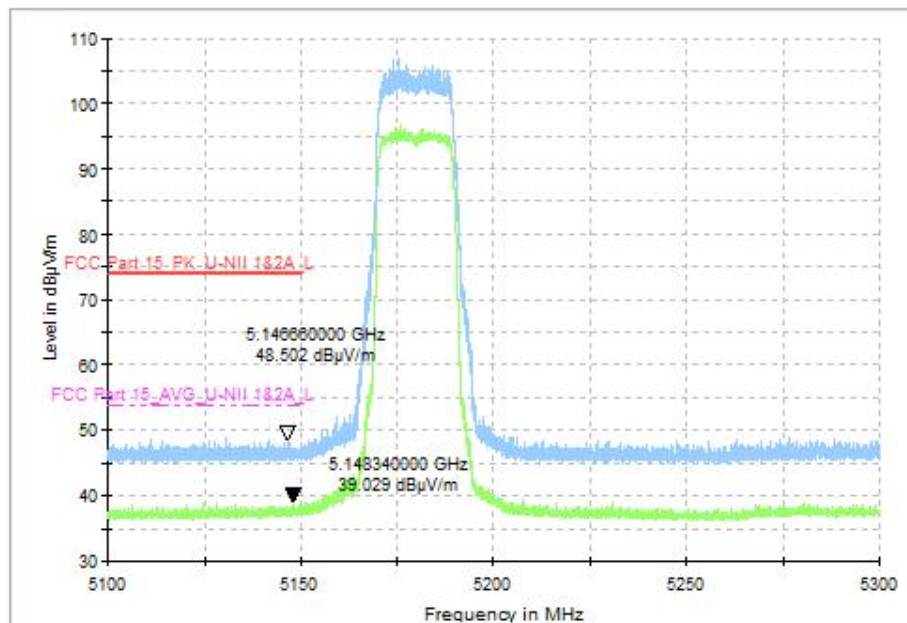
Fig. 41 Band Edges (802.11ax-HE20, CH36 5180MHz), MIMO
