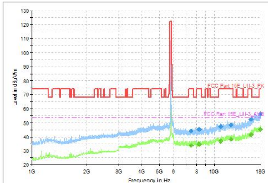
Fig. 83 Transmitter Spurious Emission (802.11n-HT40, CH159 5795MHz, 1GHz-18GHz), MIMO
