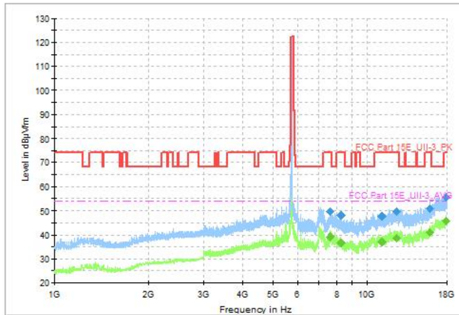
Fig. 57 Transmitter Spurious Emission (802.11ax-HE20(RU26), CH149 5745MHz, 1GHz-18GHz)
